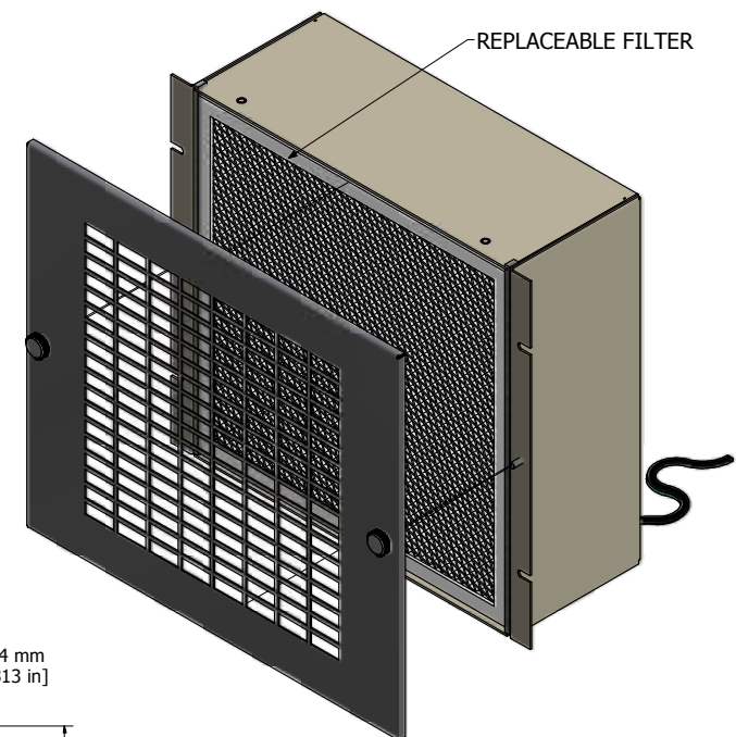
EXPLODED ASSEMBLY VIEW
