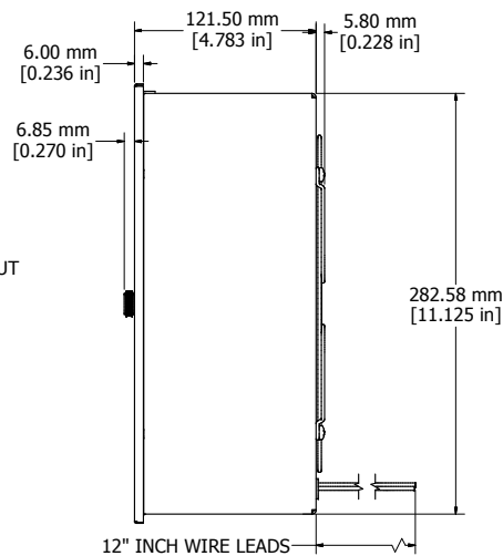
ASSEMBLY - VIEW FROM SIDE
