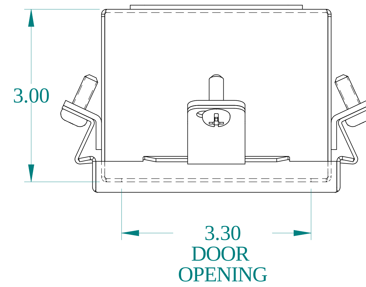
TOP VIEW
