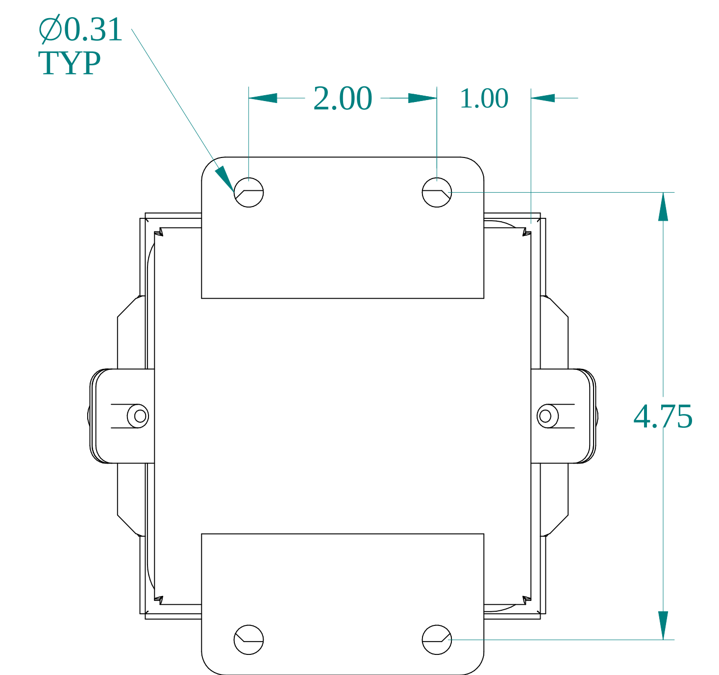
BACK VIEW
