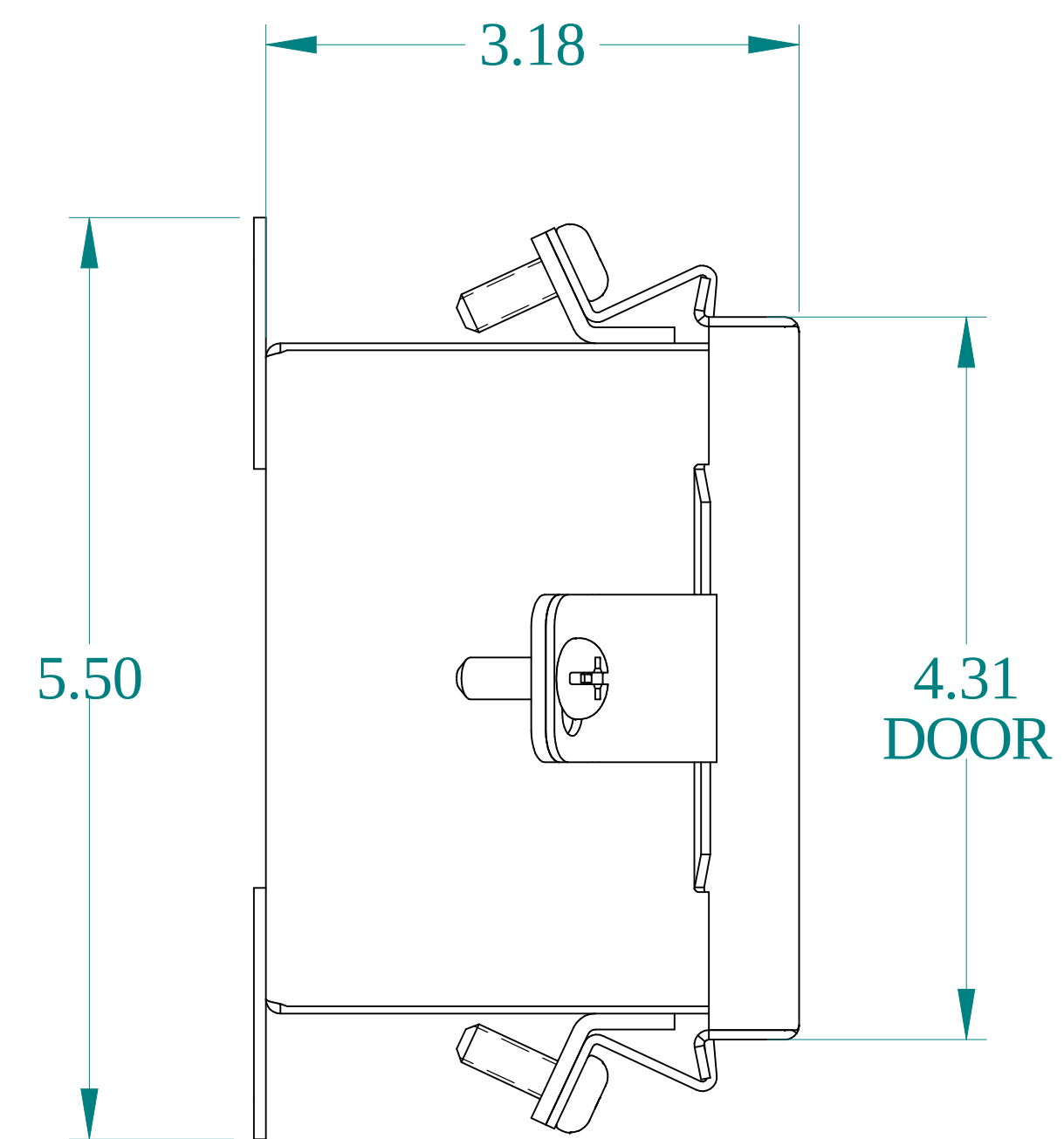
SIDE VIEW
