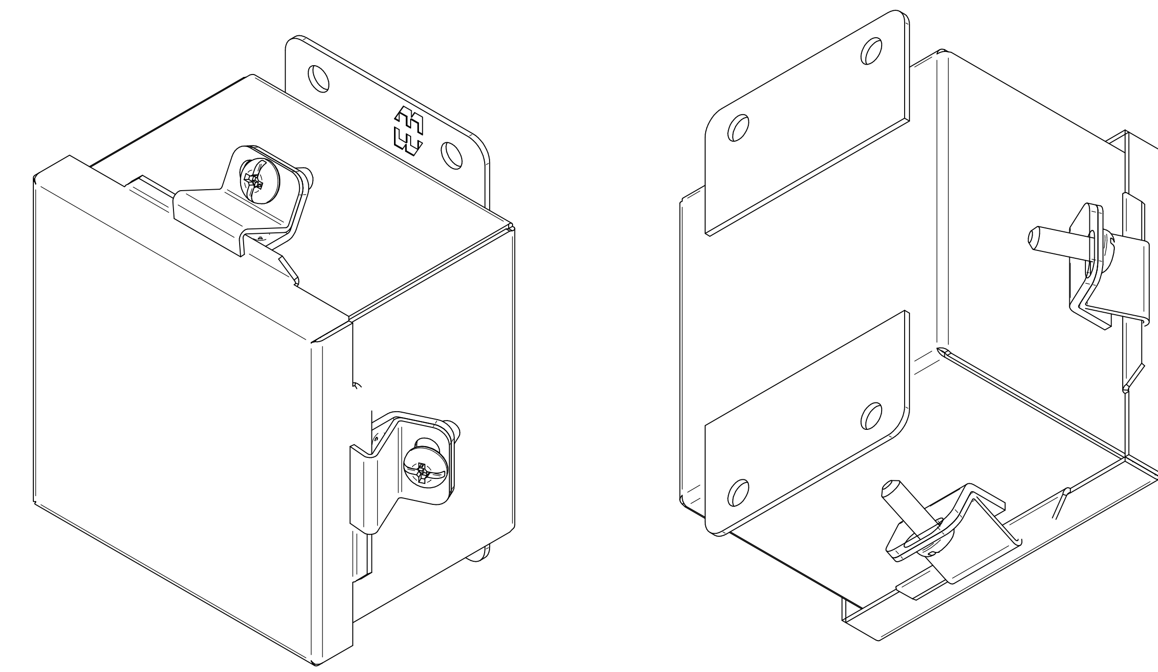
ISOMETRIC VIEWS
