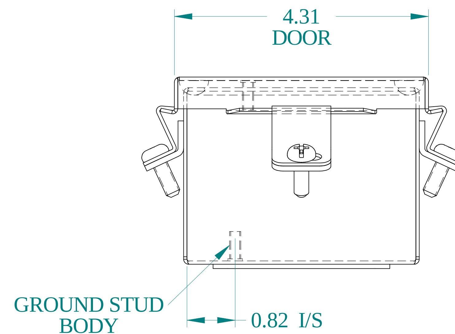
BOTTOM VIEW
