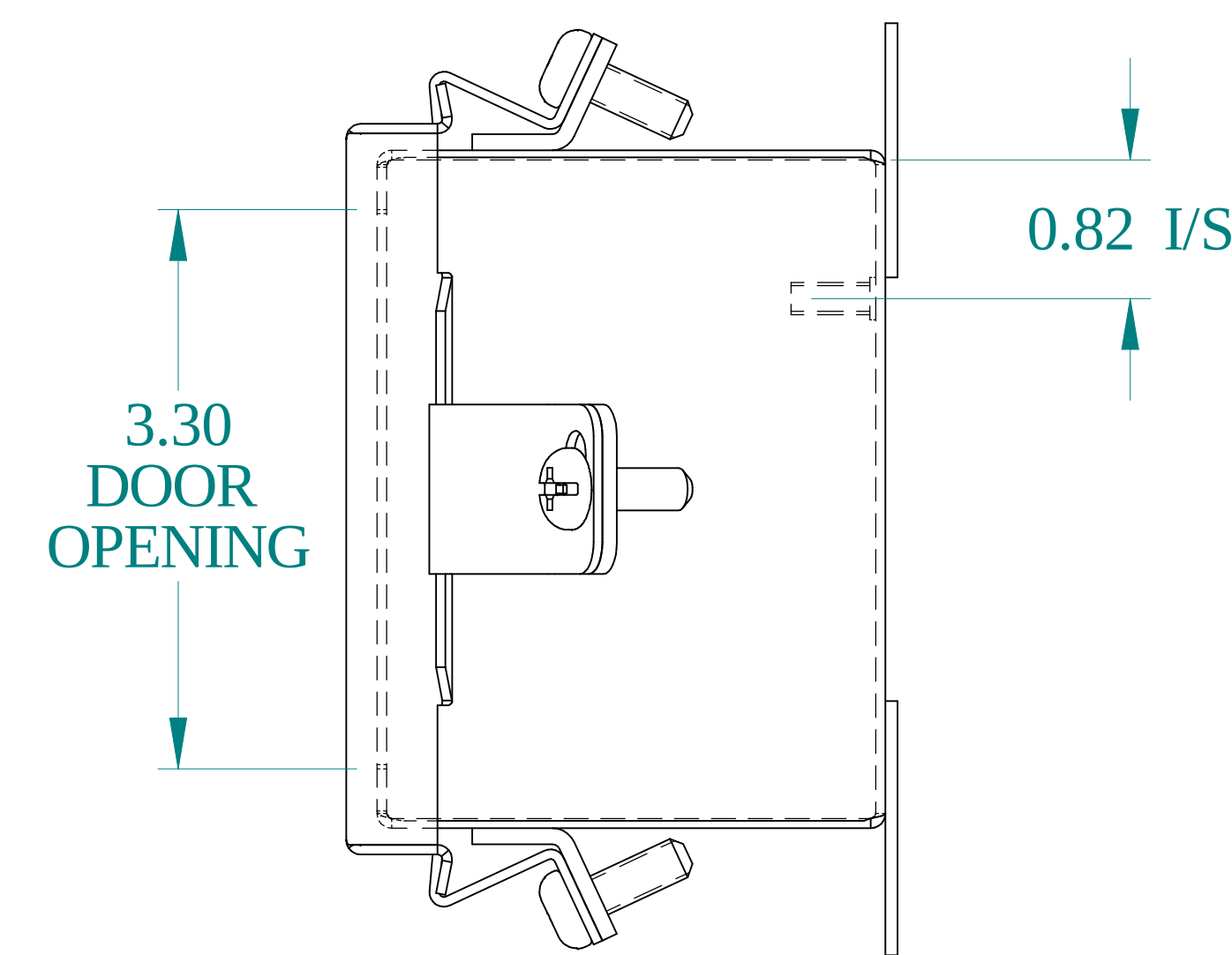
SIDE VIEW
