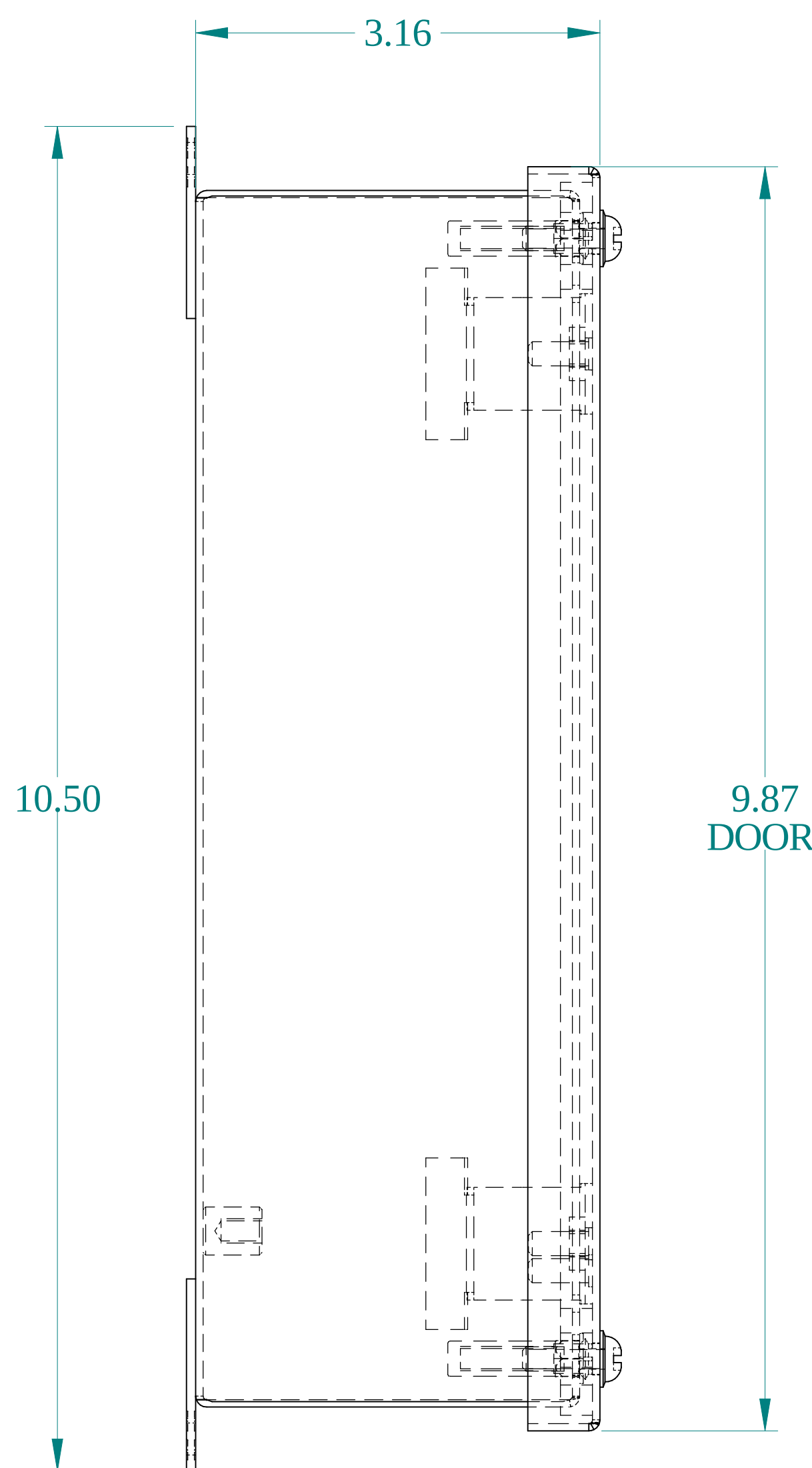
SIDE VIEW
