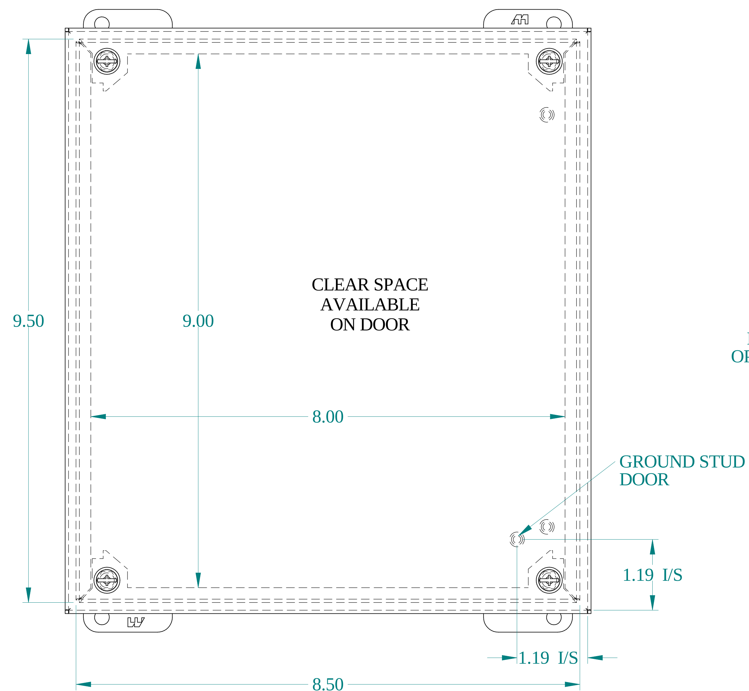
FRONT VIEW
