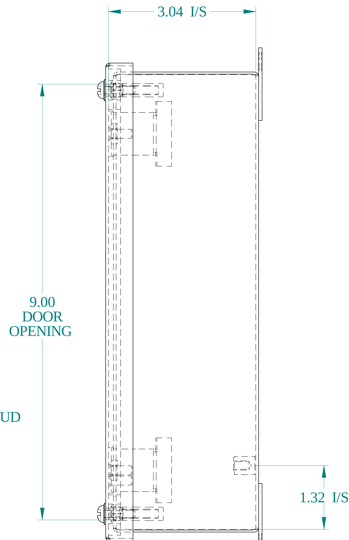
SIDE VIEW
