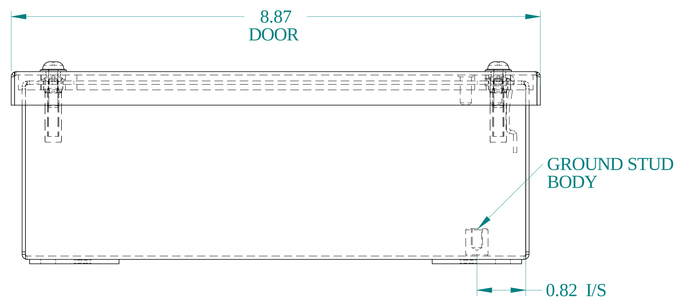
BOTTOM VIEW
