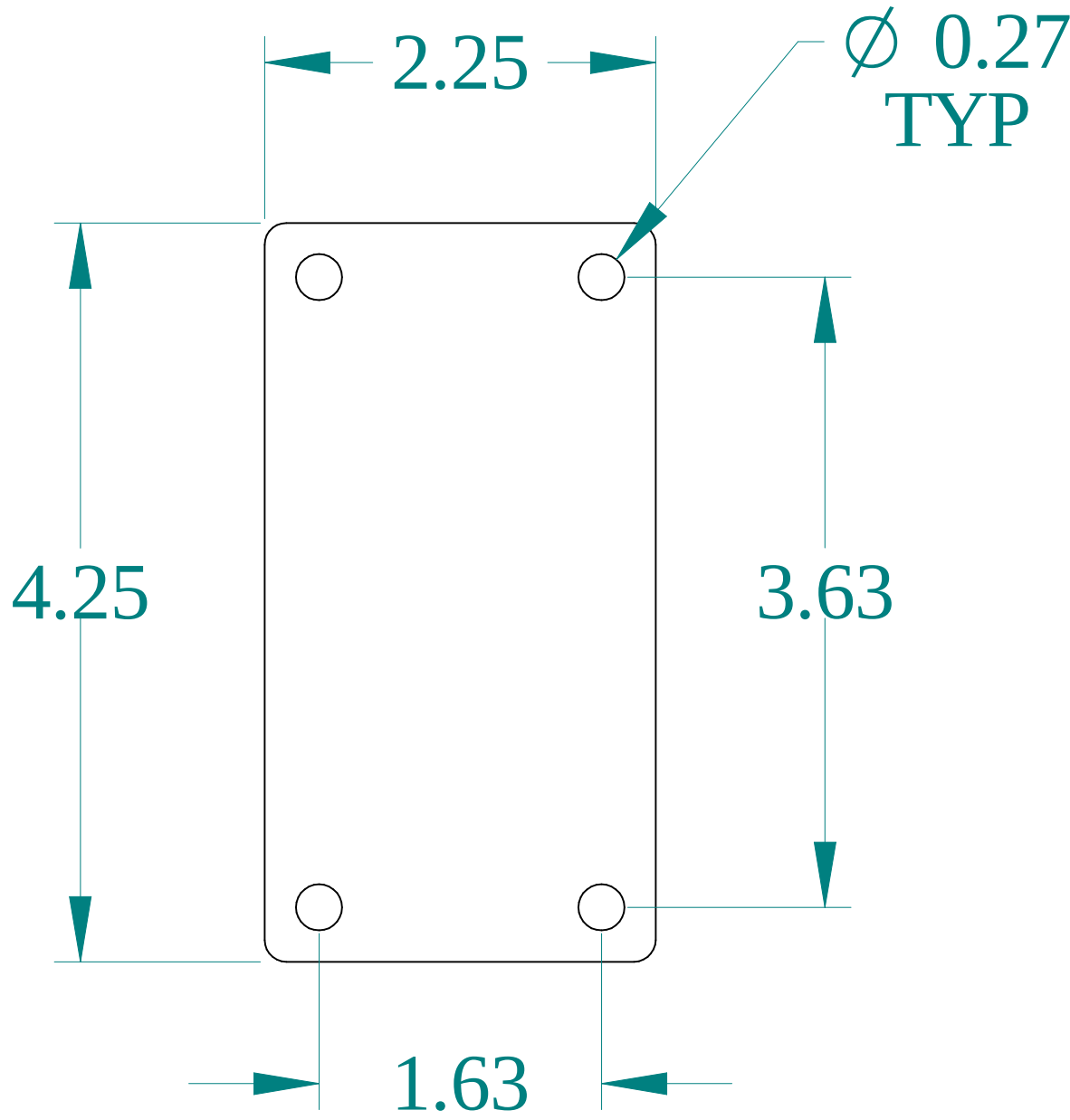
TOP VIEW
