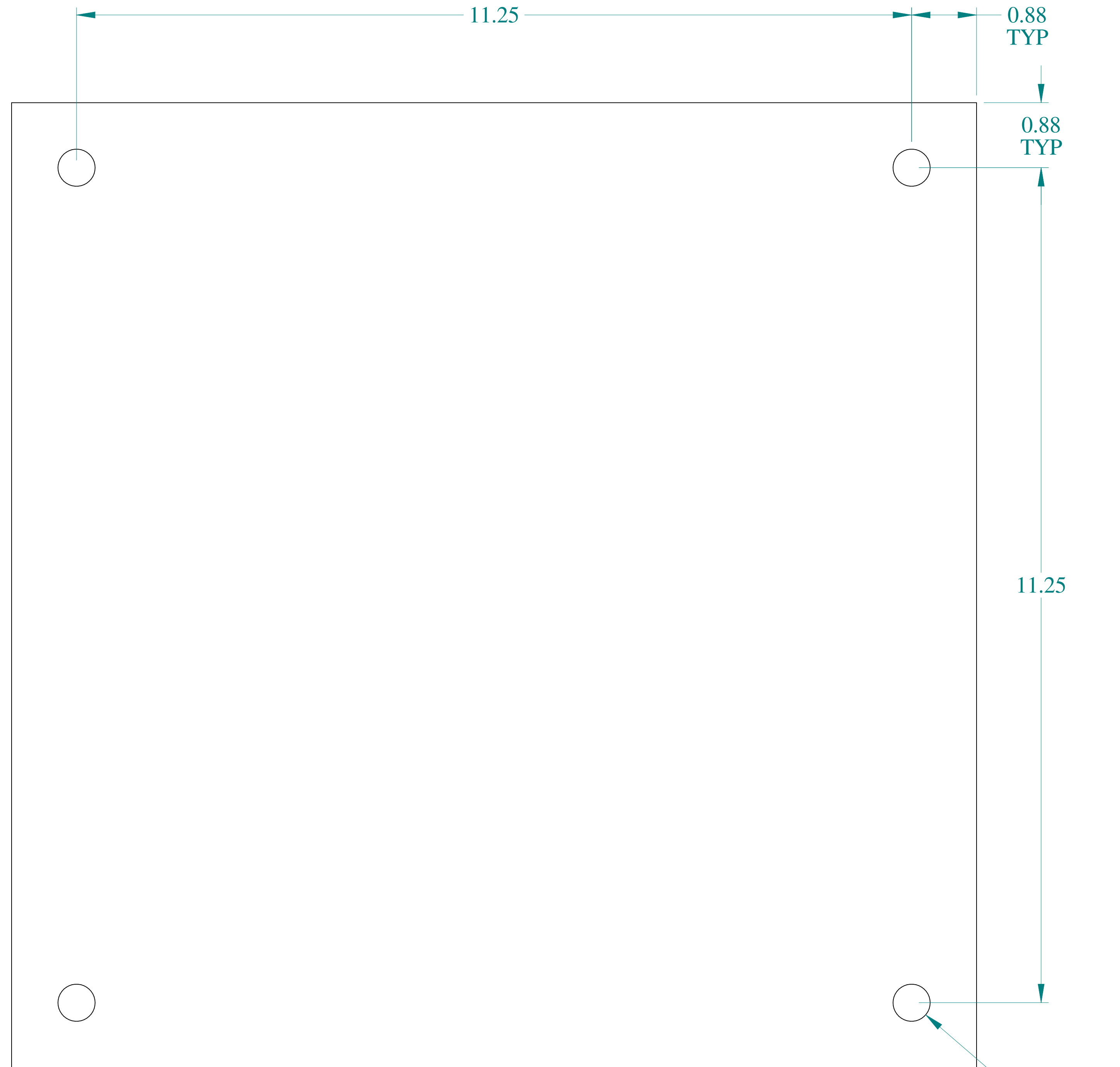
FRONT VIEW
