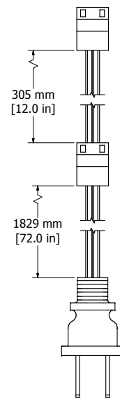
NEMA 1-15P DAISY CHAIN (2 FAN) CORD (1X)
