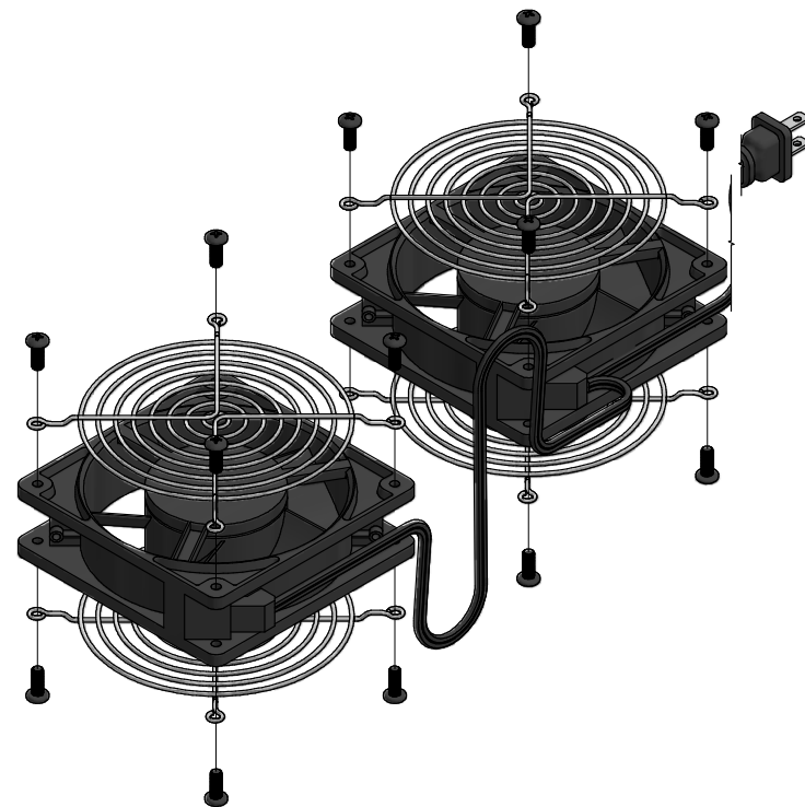
EXPLODED ASSEMBLY VIEW
