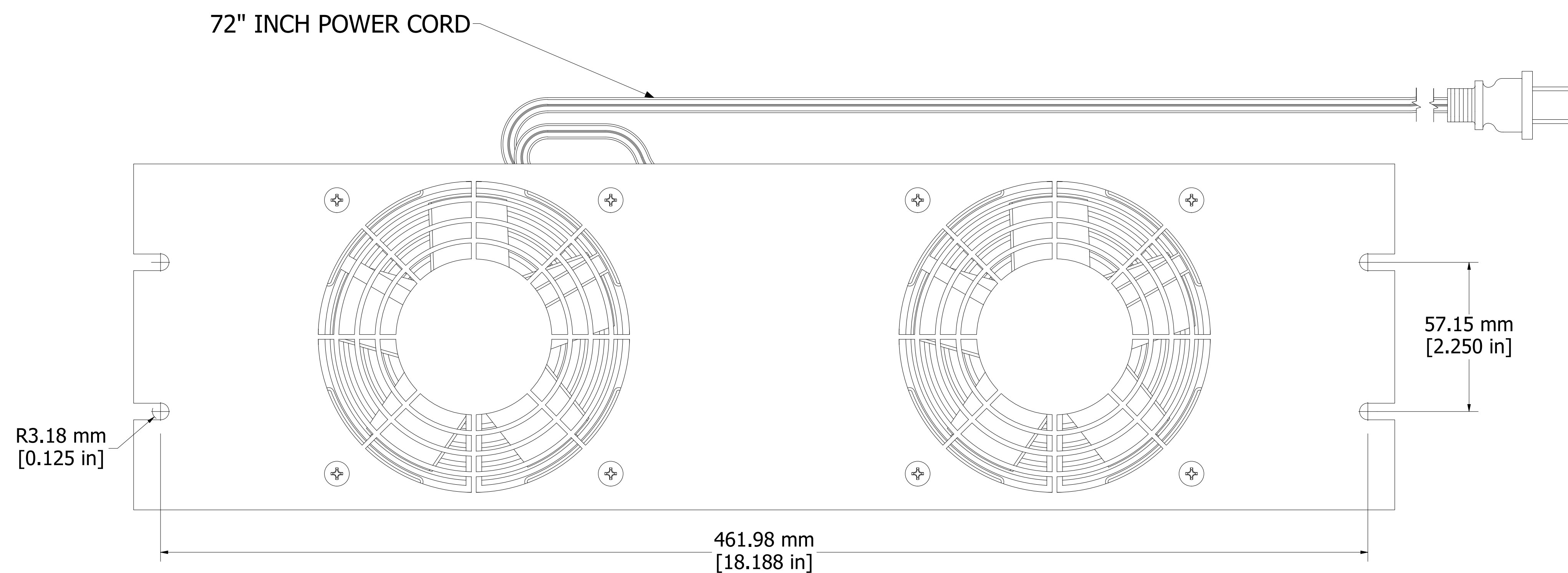
ASSEMBLY - VIEW FROM FRONT
