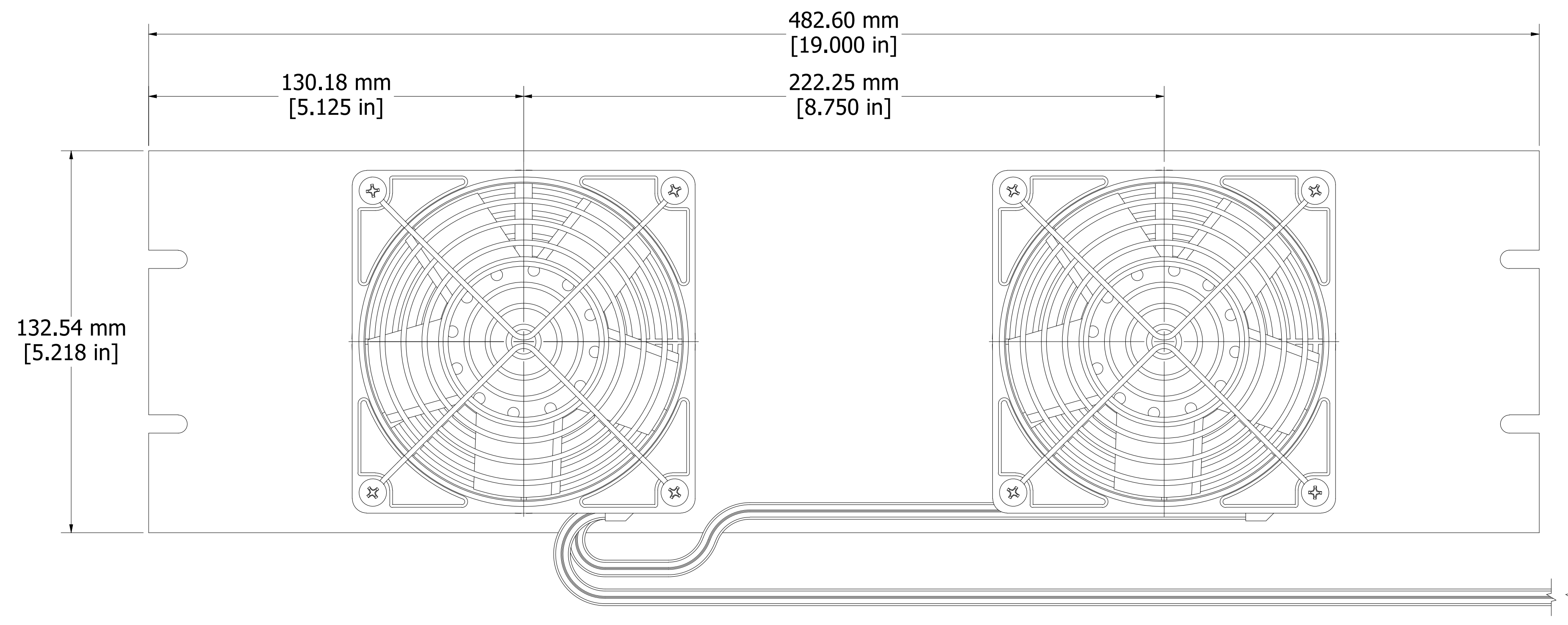
ASSEMBLY - VIEW FROM REAR
