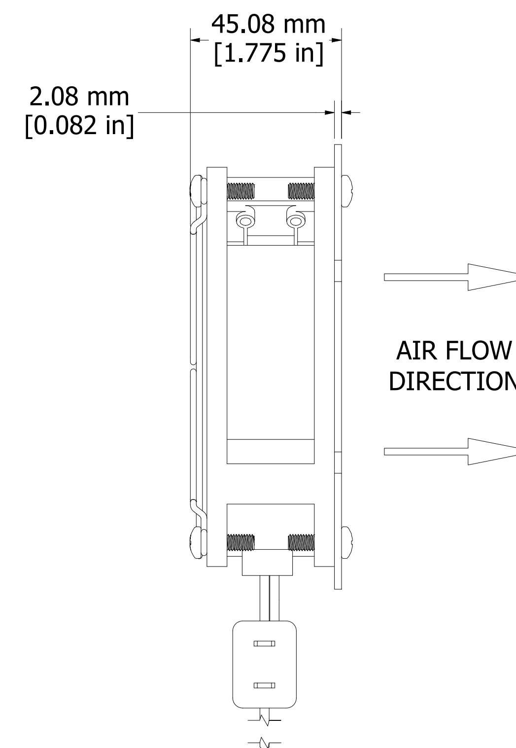
ASSEMBLY - VIEW FROM SIDE
