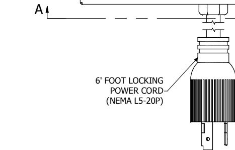
ASSEMBLY - VIEW FROM BOTTOM
