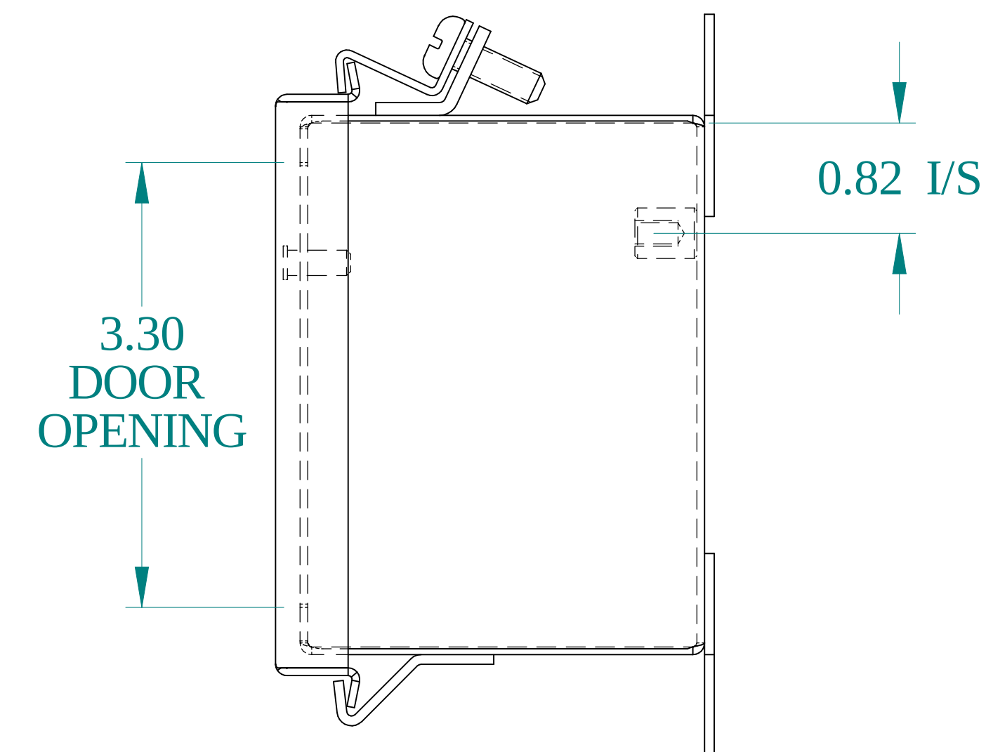
SIDE VIEW
