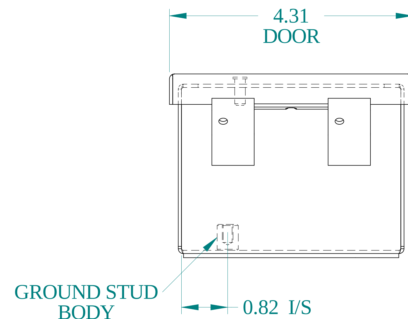
BOTTOM VIEW
