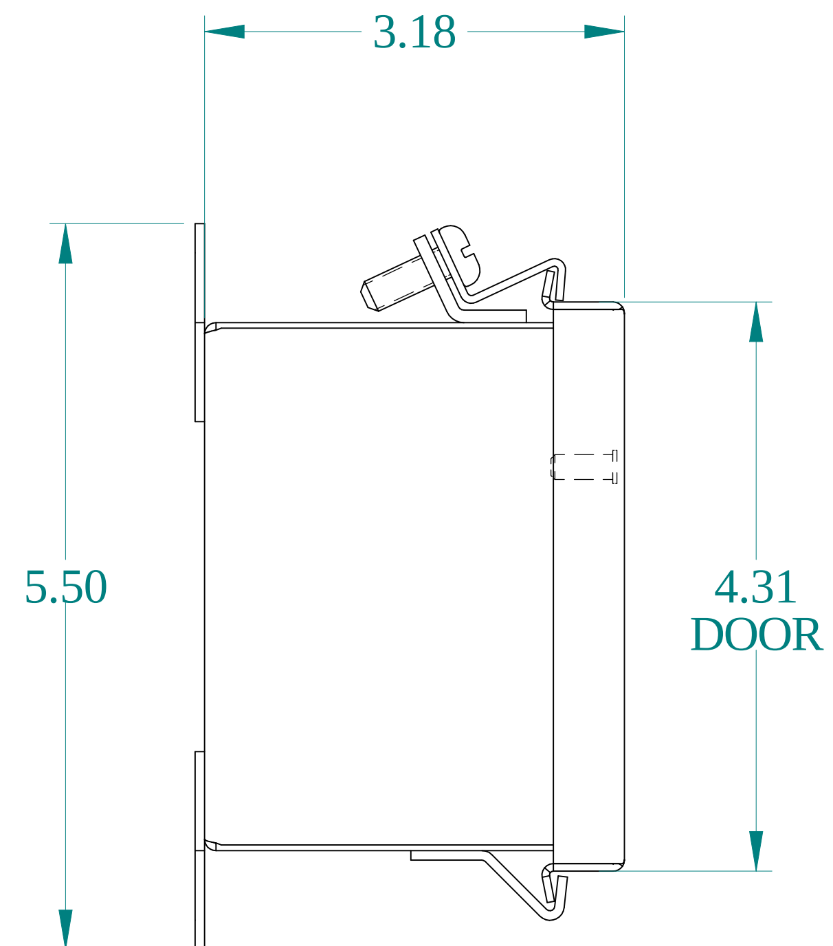
SIDE VIEW
