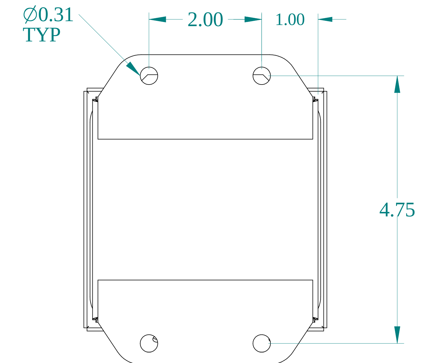
BACK VIEW
