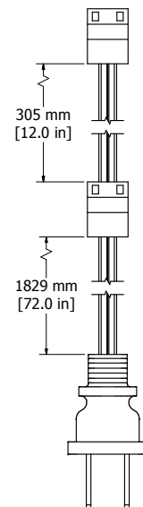
NEMA 1-15P DAISY CHAIN (2 FAN) CORD (1X)
