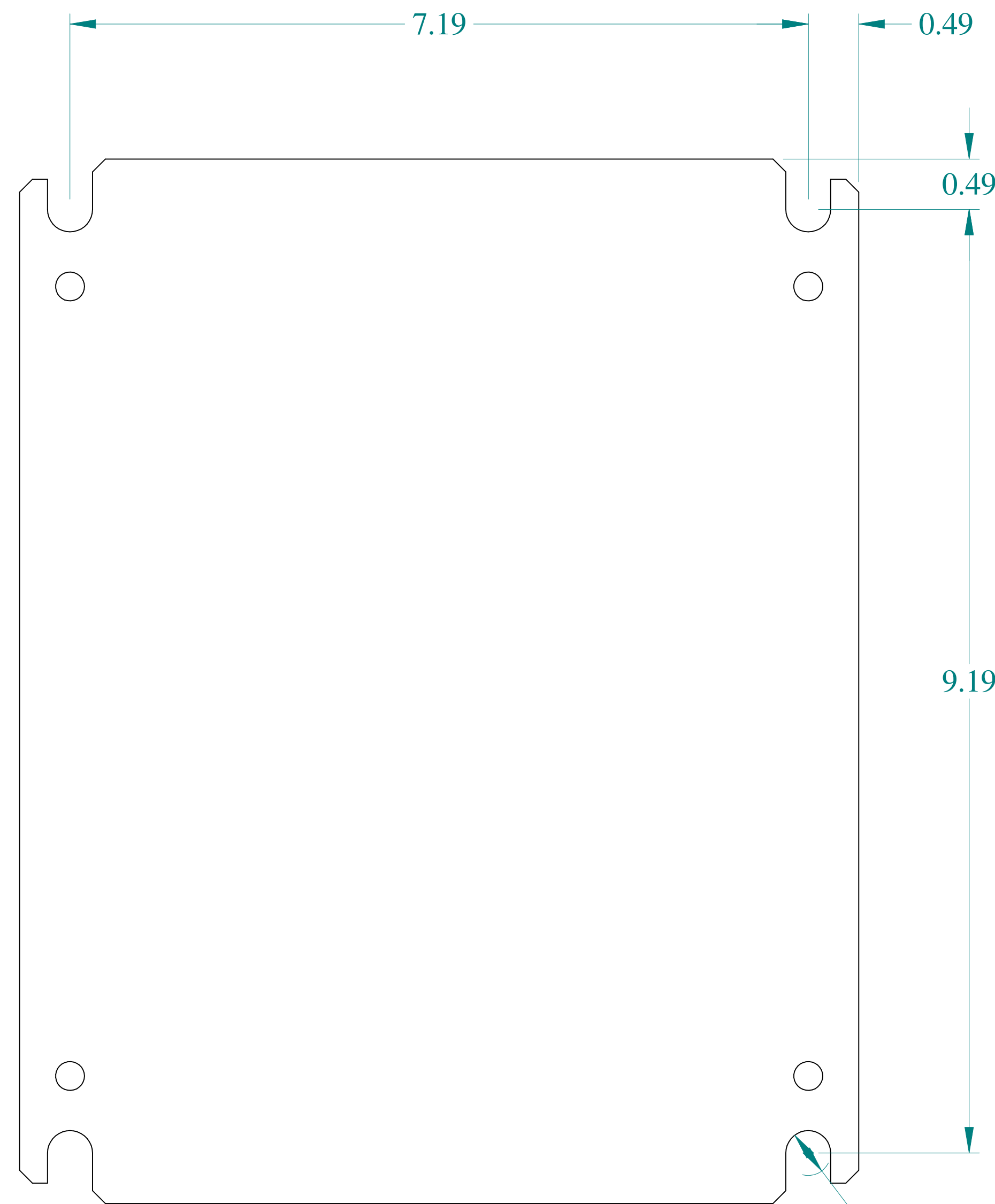
FRONT VIEW
