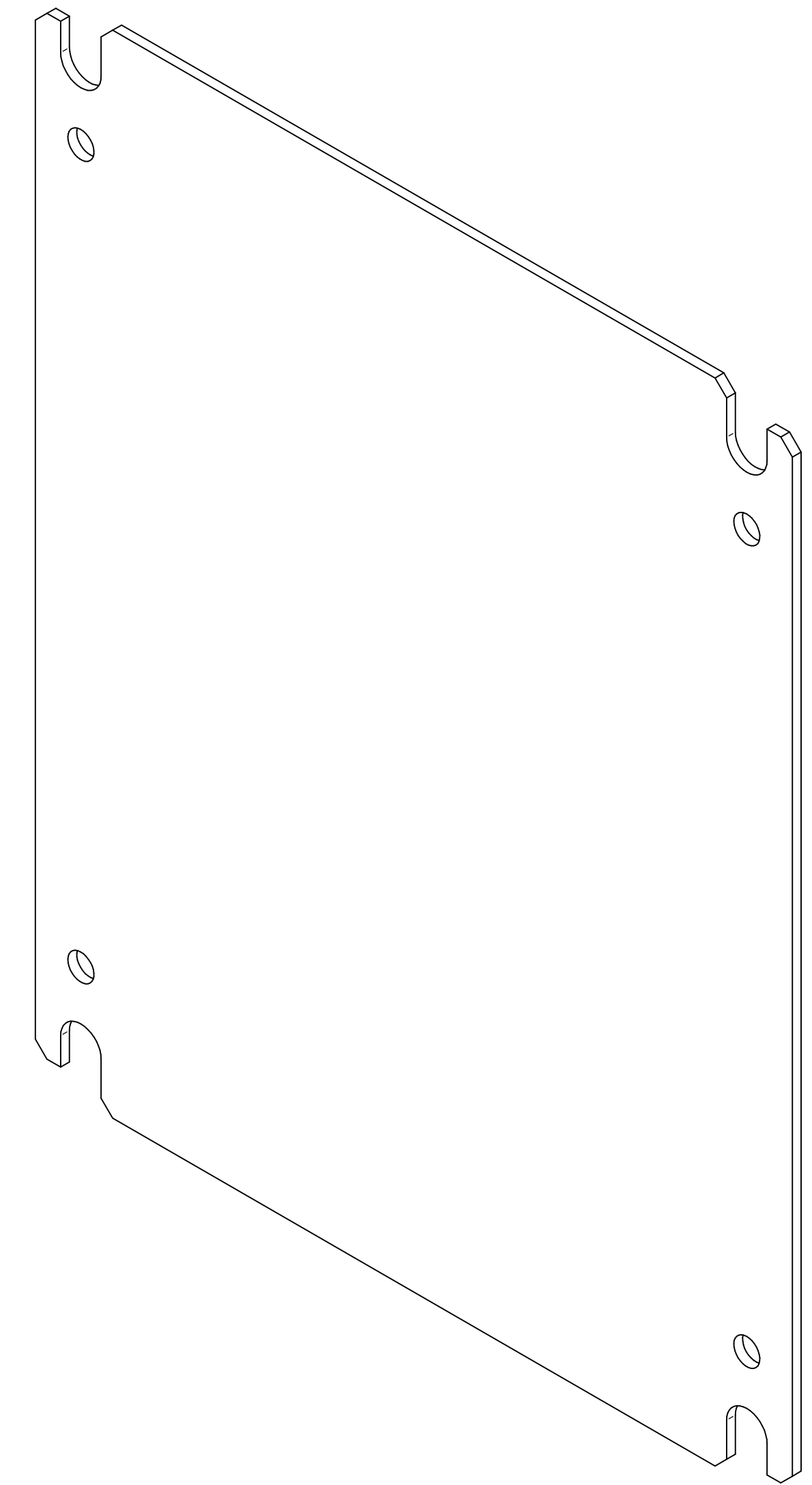
ISOMETRIC VIEW
