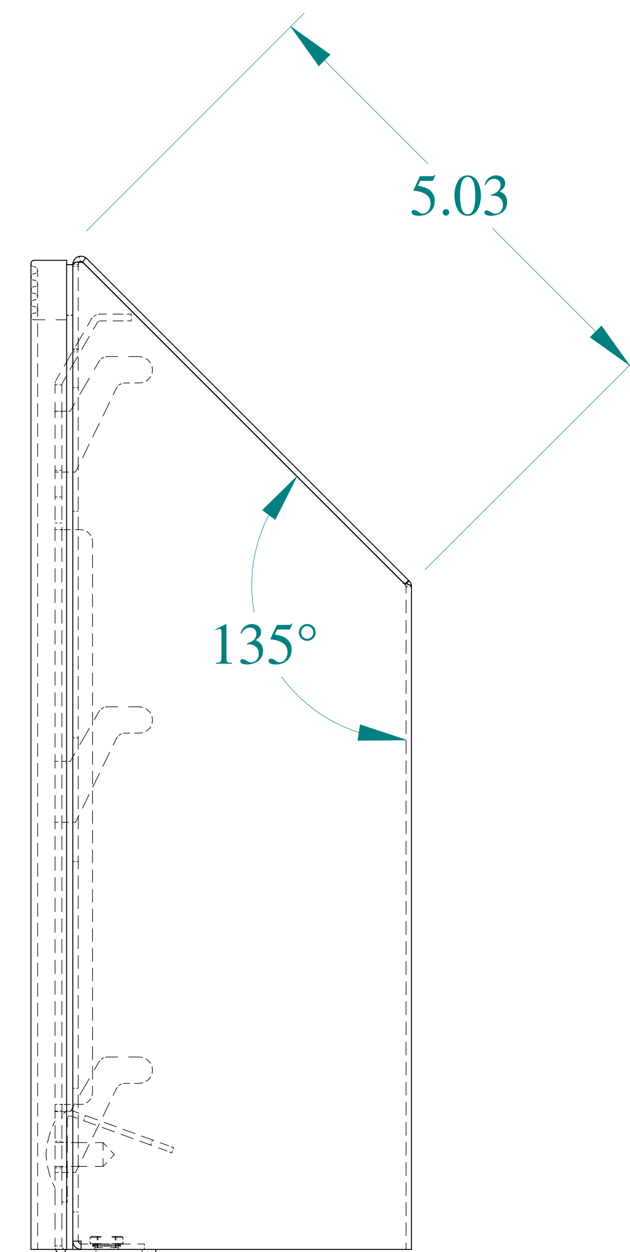
SIDE VIEW
