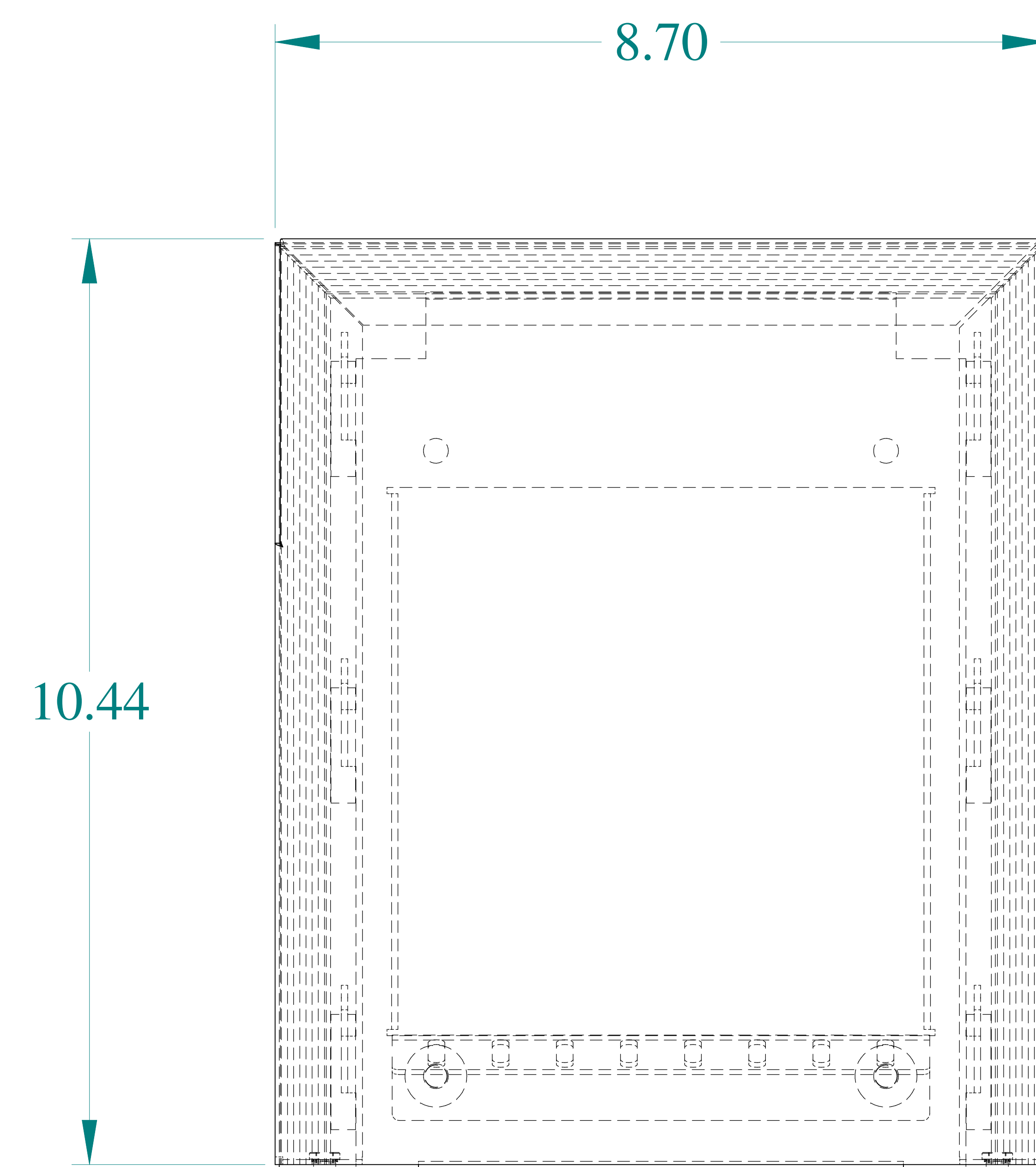
FRONT VIEW
