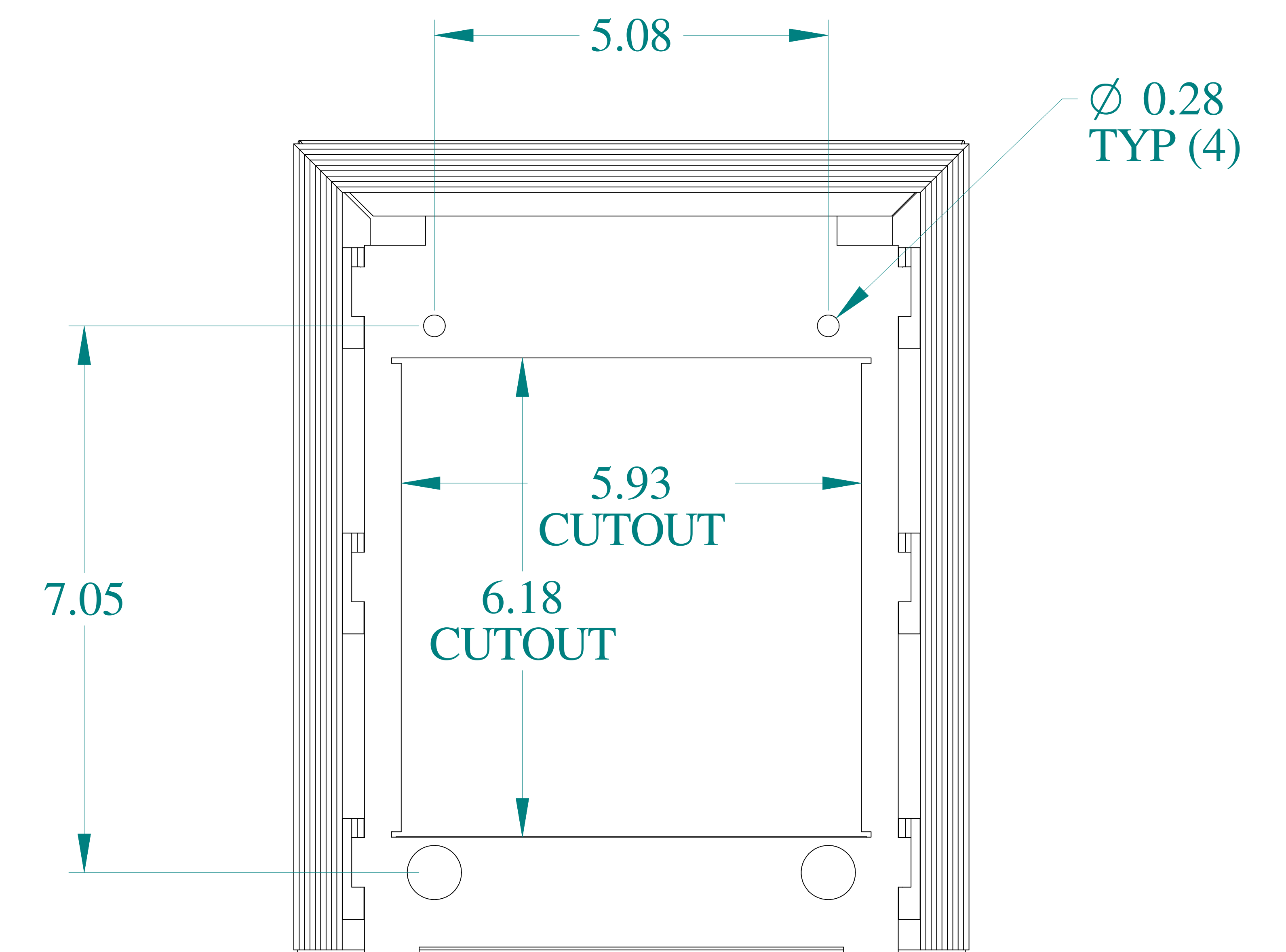
BACK VIEW
