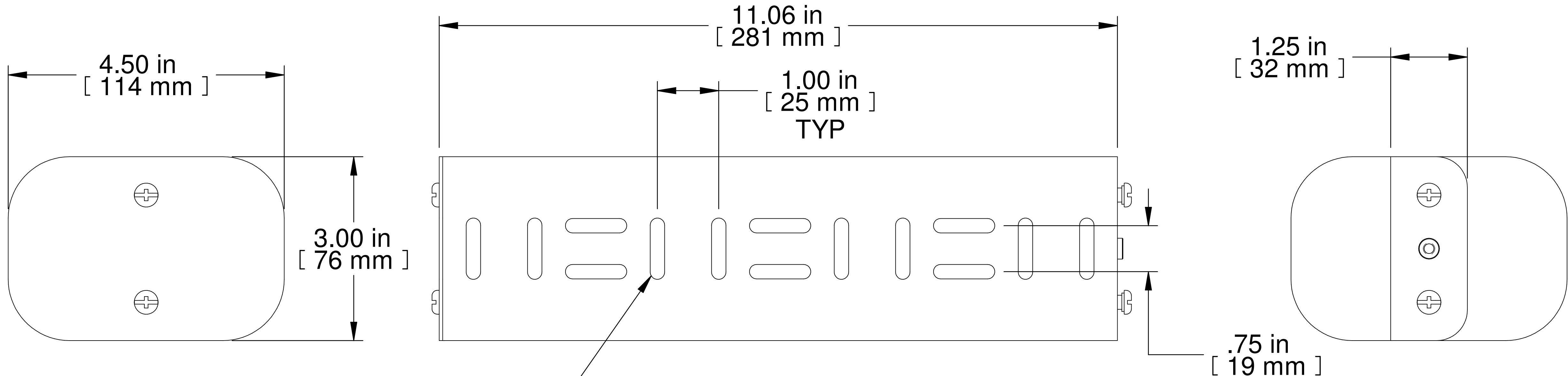
L.S. VIEW
