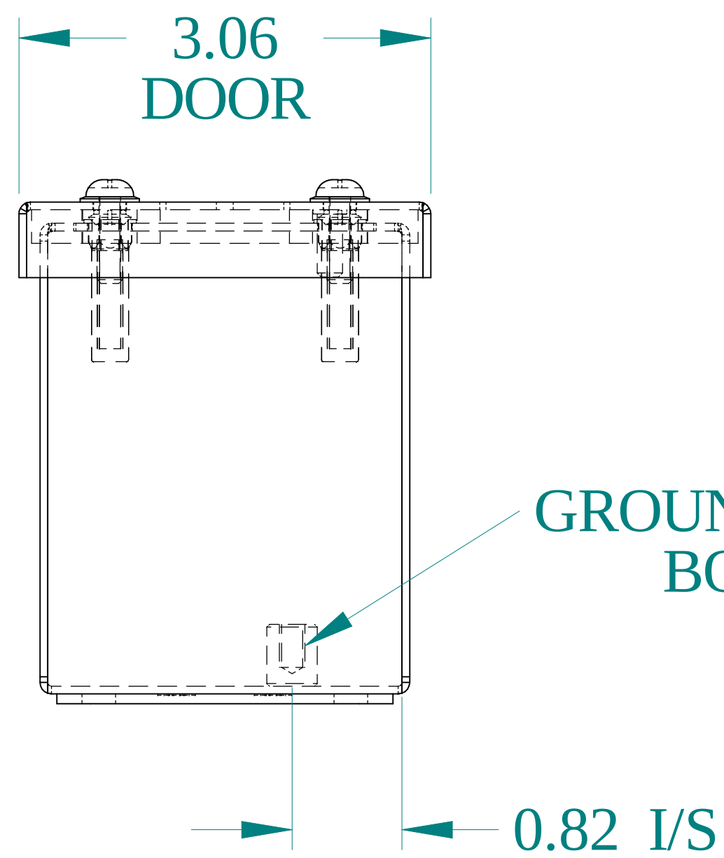
BOTTOM VIEW
