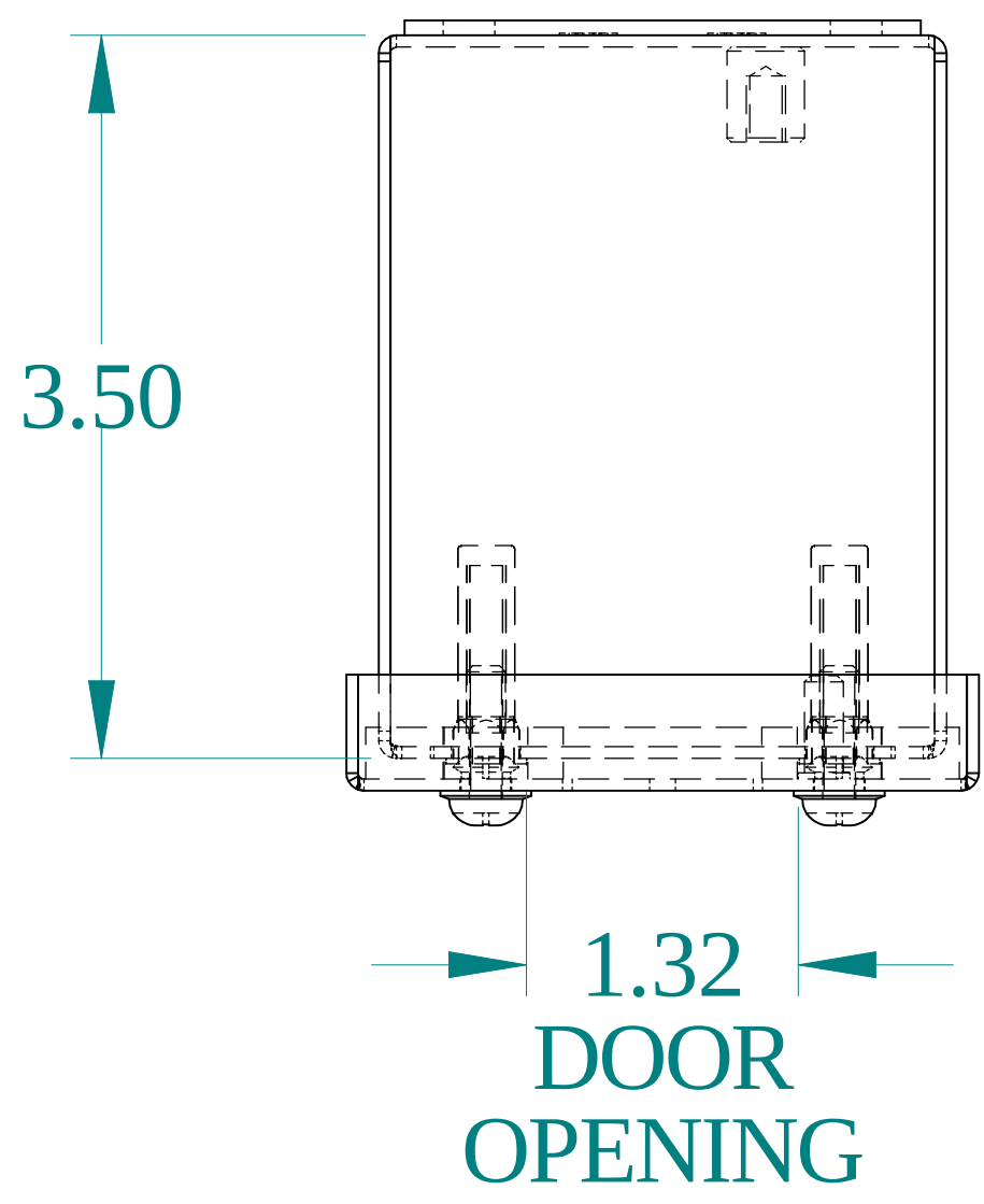
TOP VIEW
