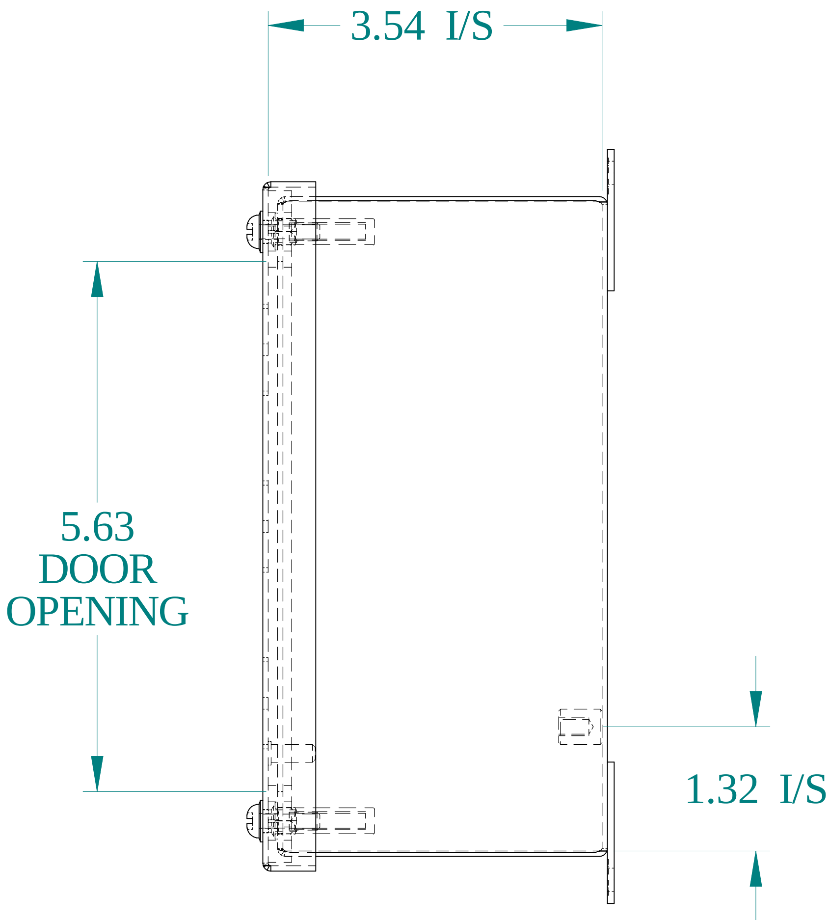
SIDE VIEW
