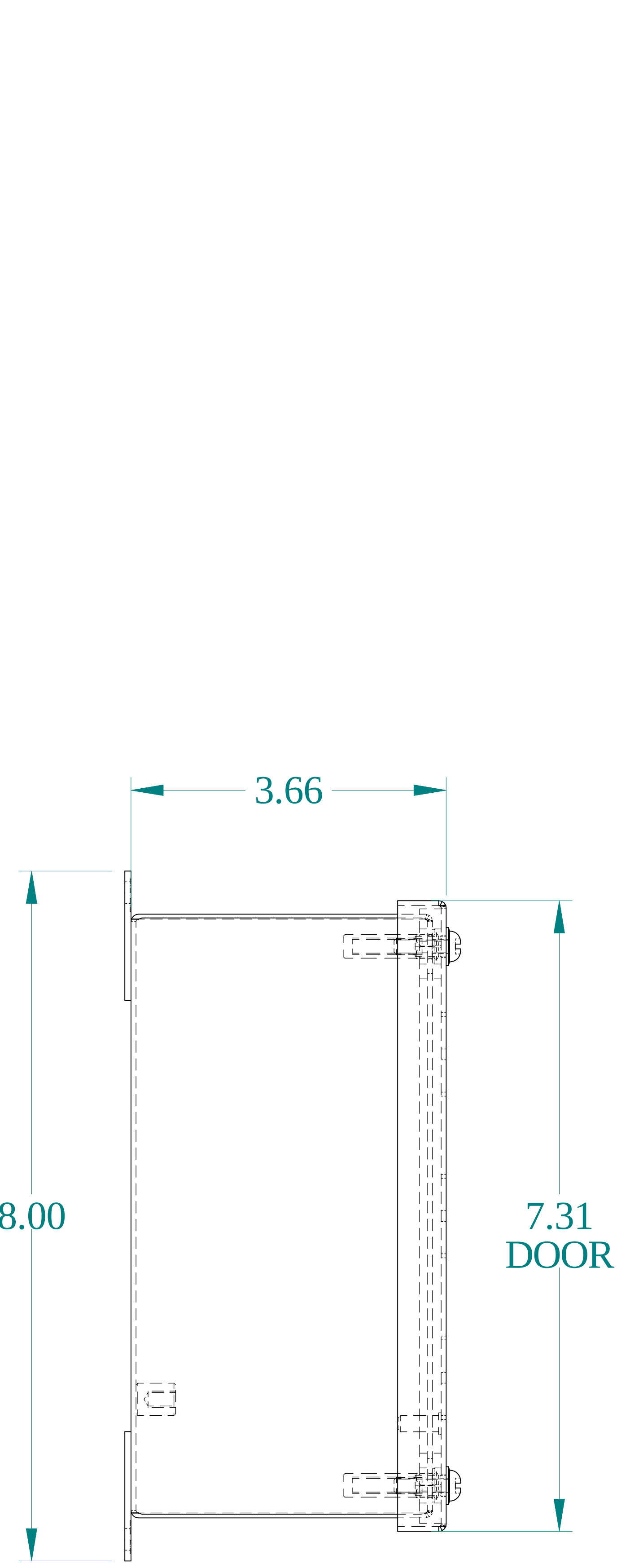
SIDE VIEW
