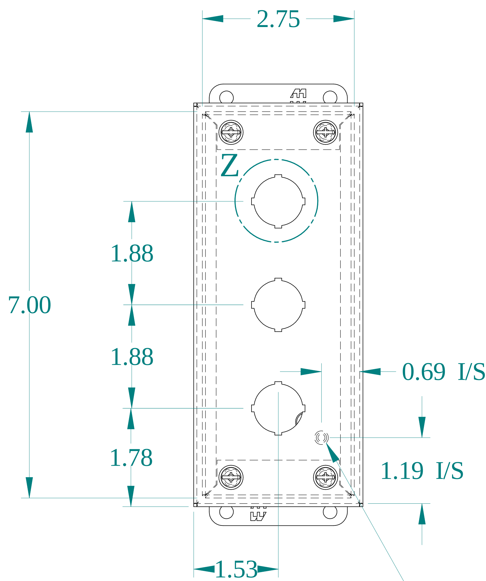
FRONT VIEW
