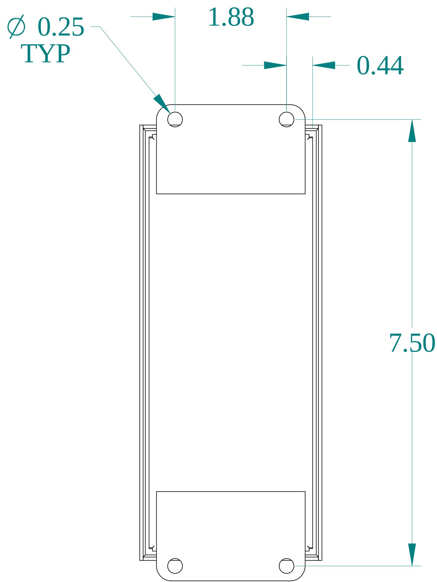
BACK VIEW
