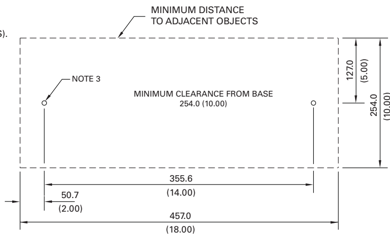
MOUNTING DETAIL
