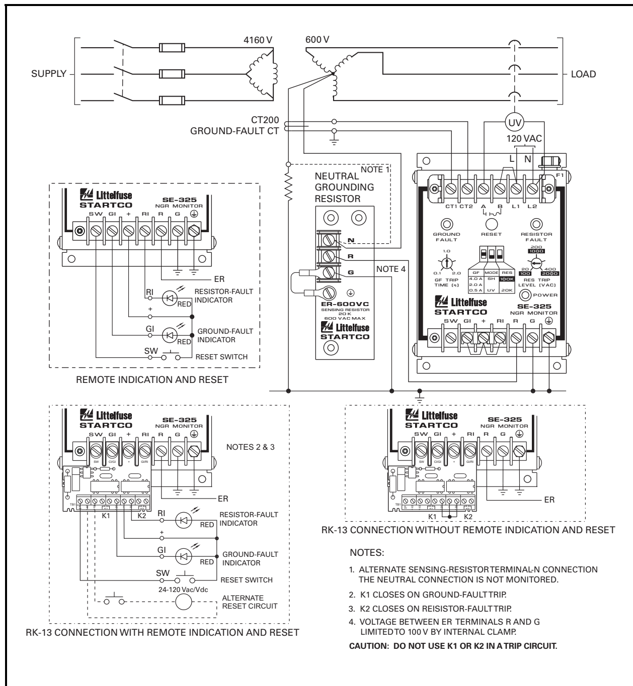
FIGURE 1. Typical Application.
