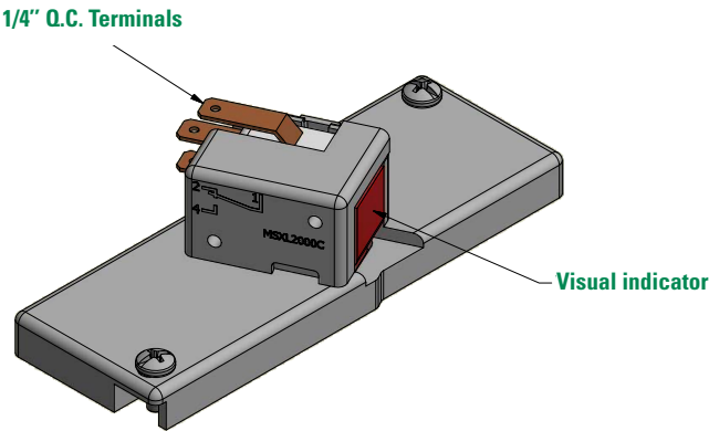
Microswitch [Dimensions in millimeters] (MSXL2000C)
