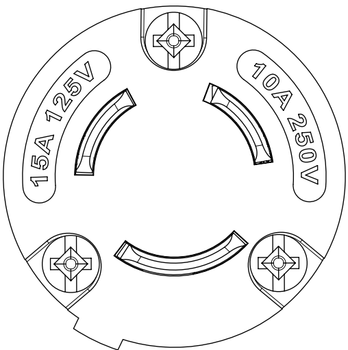
FACE VIEW
