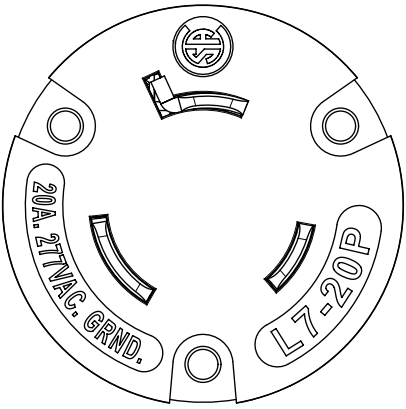
FACE VIEW
