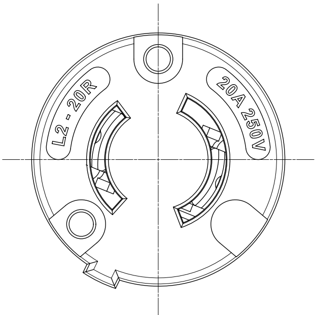
FACE VIEW
