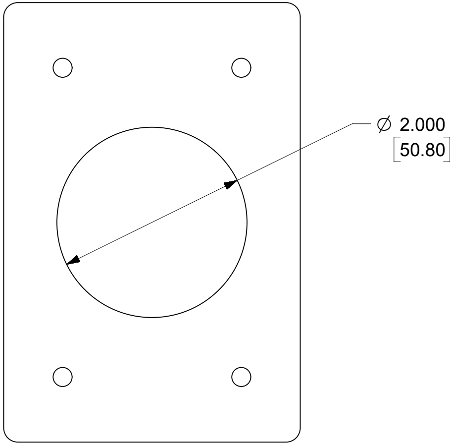
CLEARENCE HOLE (FOR PANEL MOUNT)
