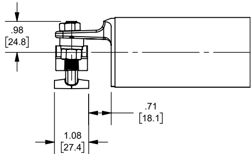
EYEBOLT
