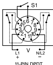
11-PIN DPDT
