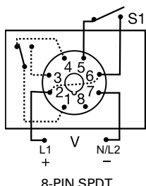
8-PIN SPDT
