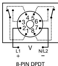
8-PIN DPDT
