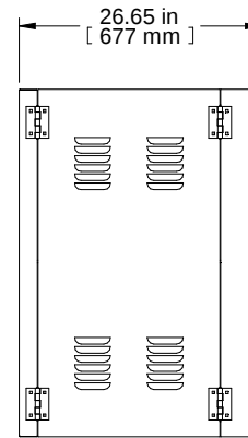
R.S. VIEW
