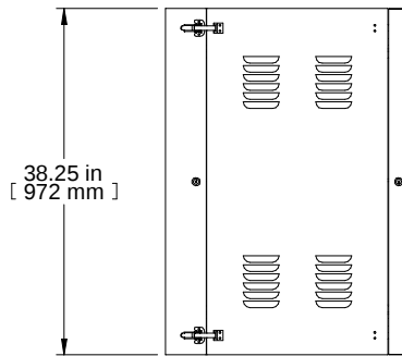
L.S. VIEW
