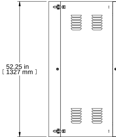
L.S. VIEW
