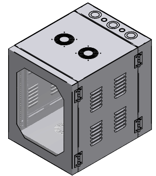
ISOMETRIC
