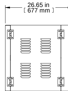
R.S. VIEW
