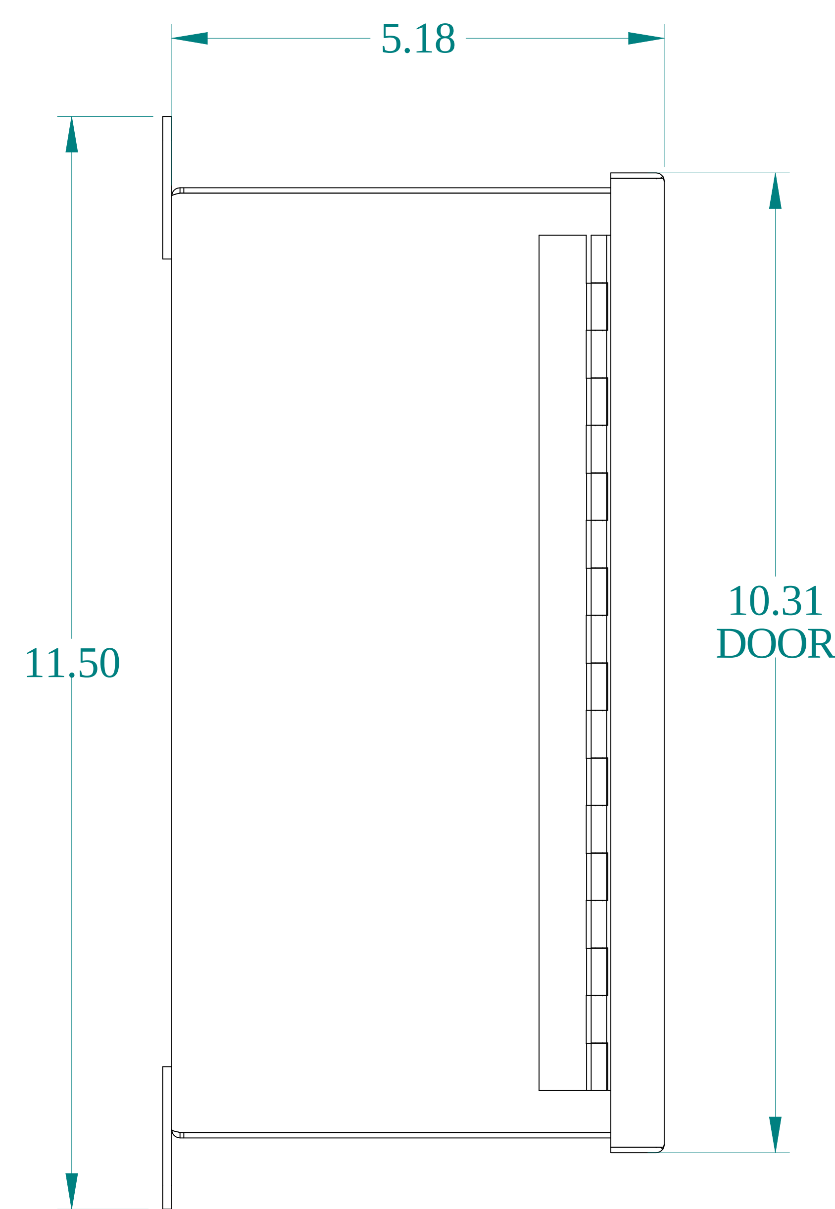
SIDE VIEW
