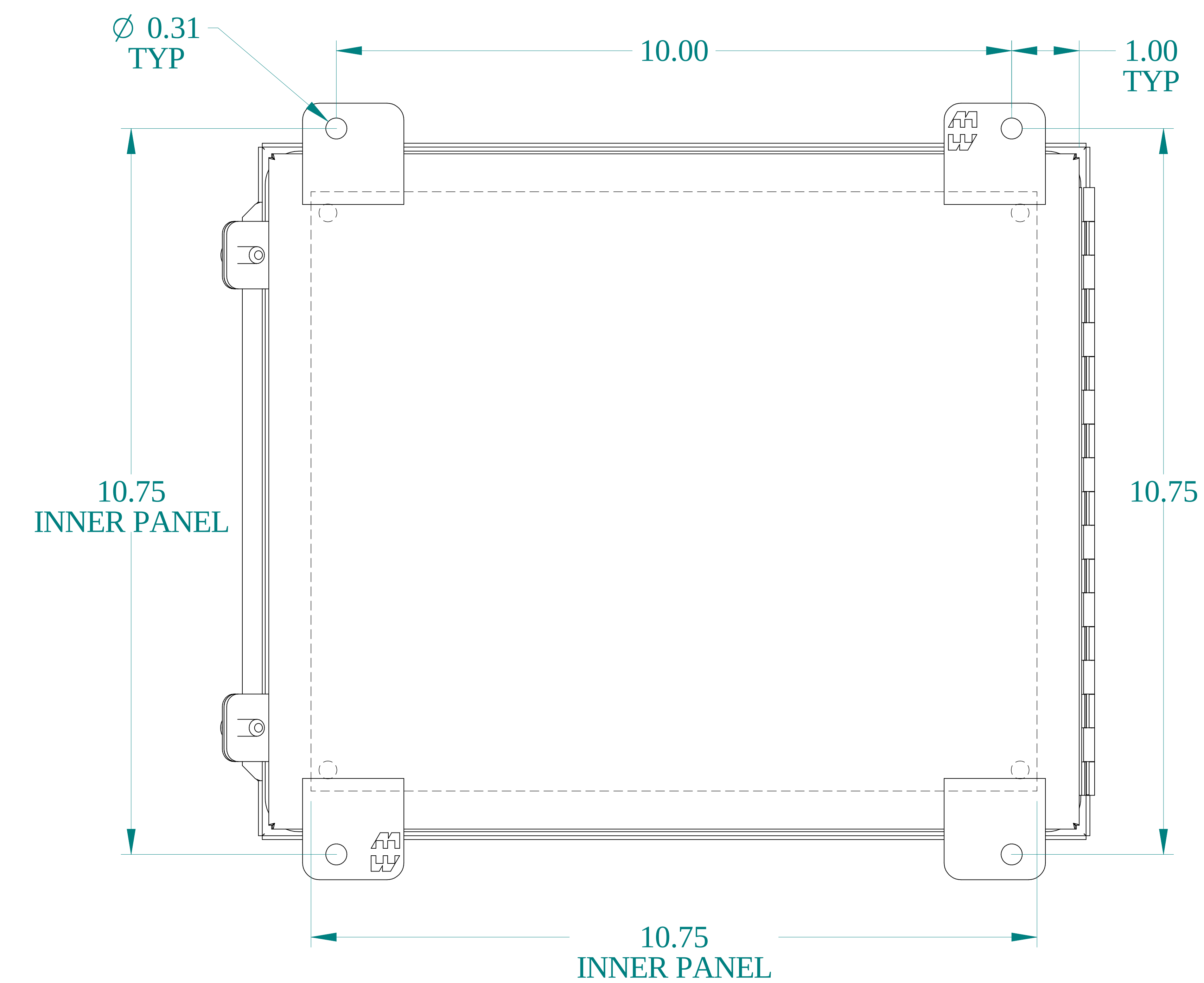
BACK VIEW
