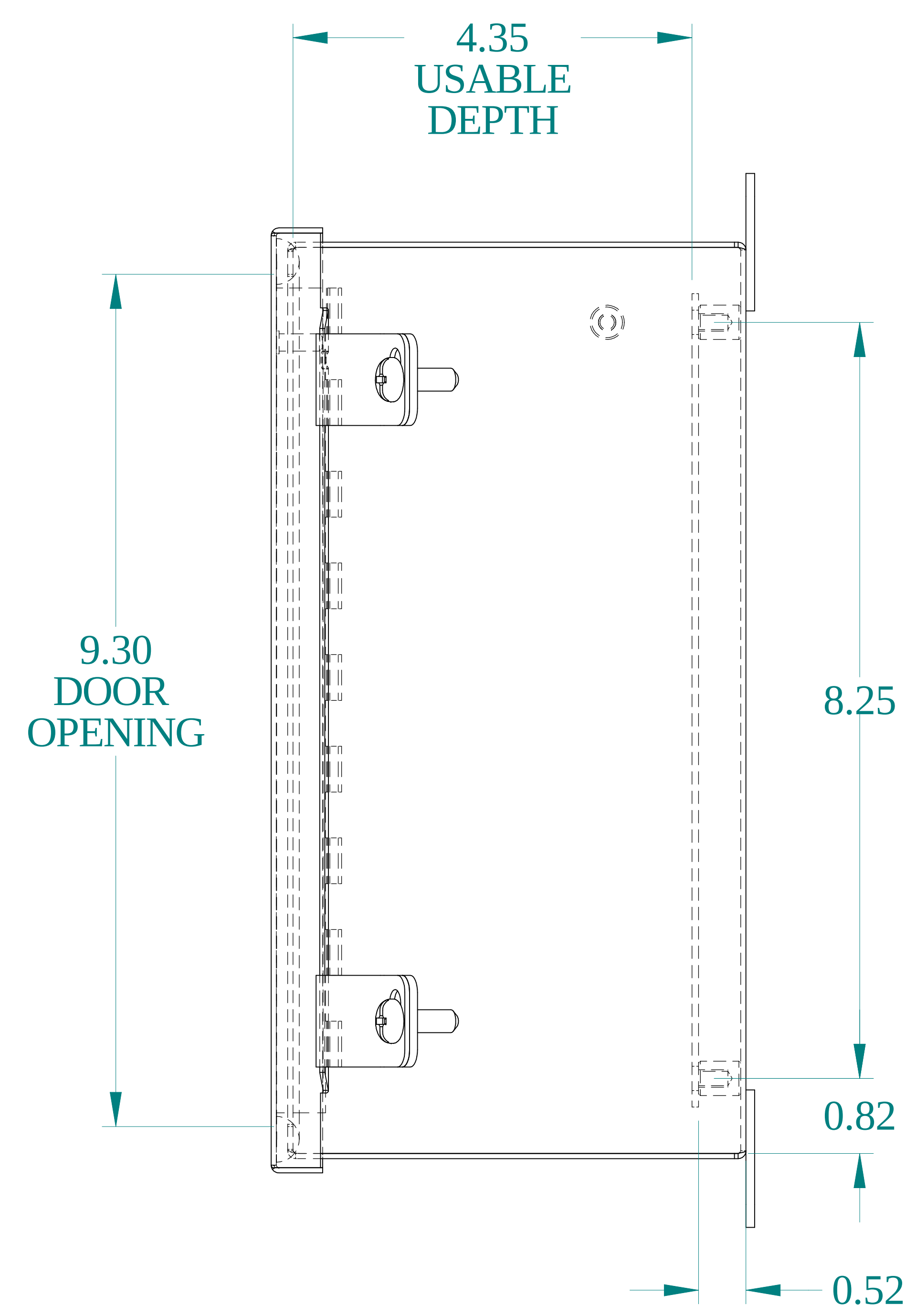
SIDE VIEW
