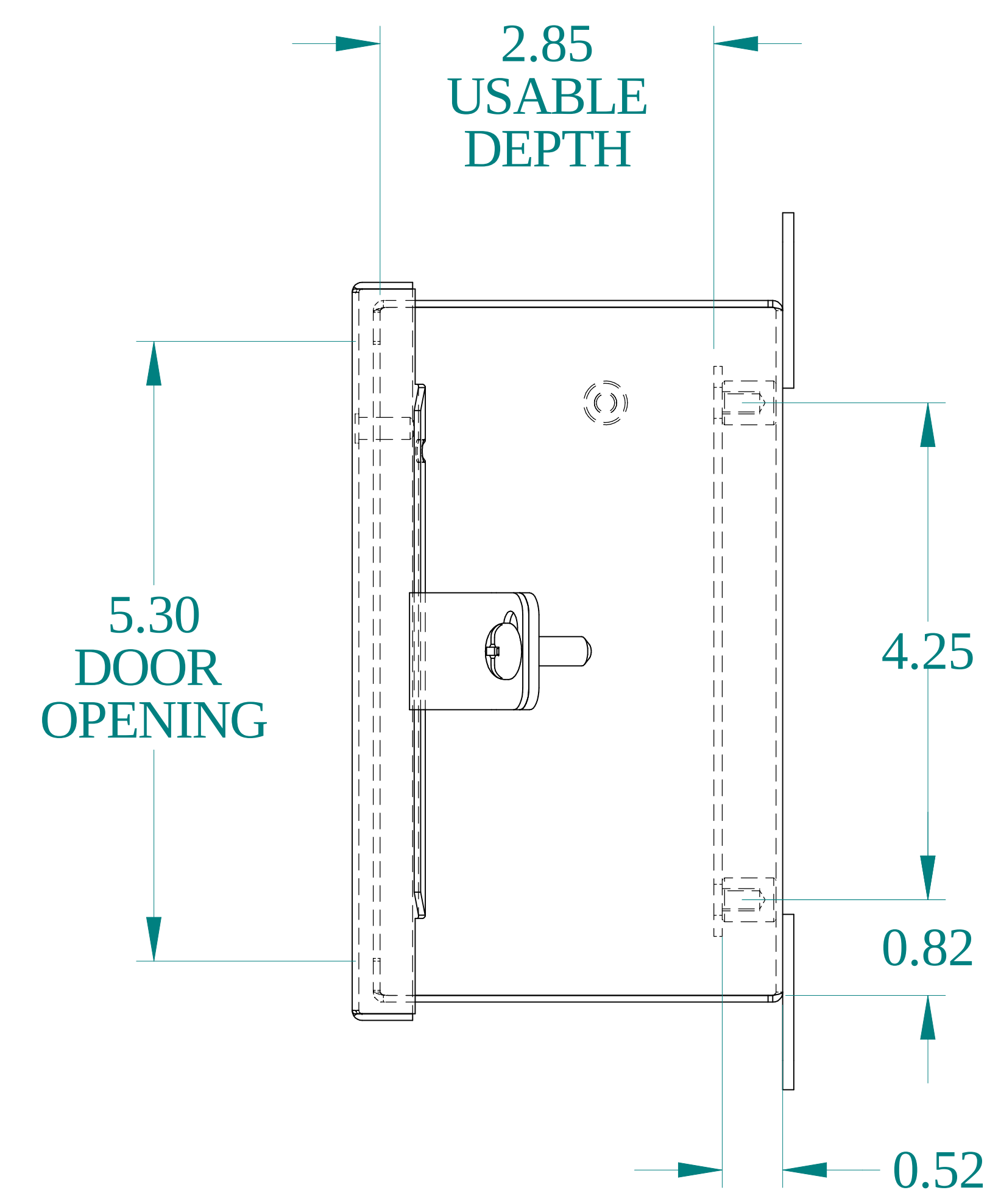
SIDE VIEW
