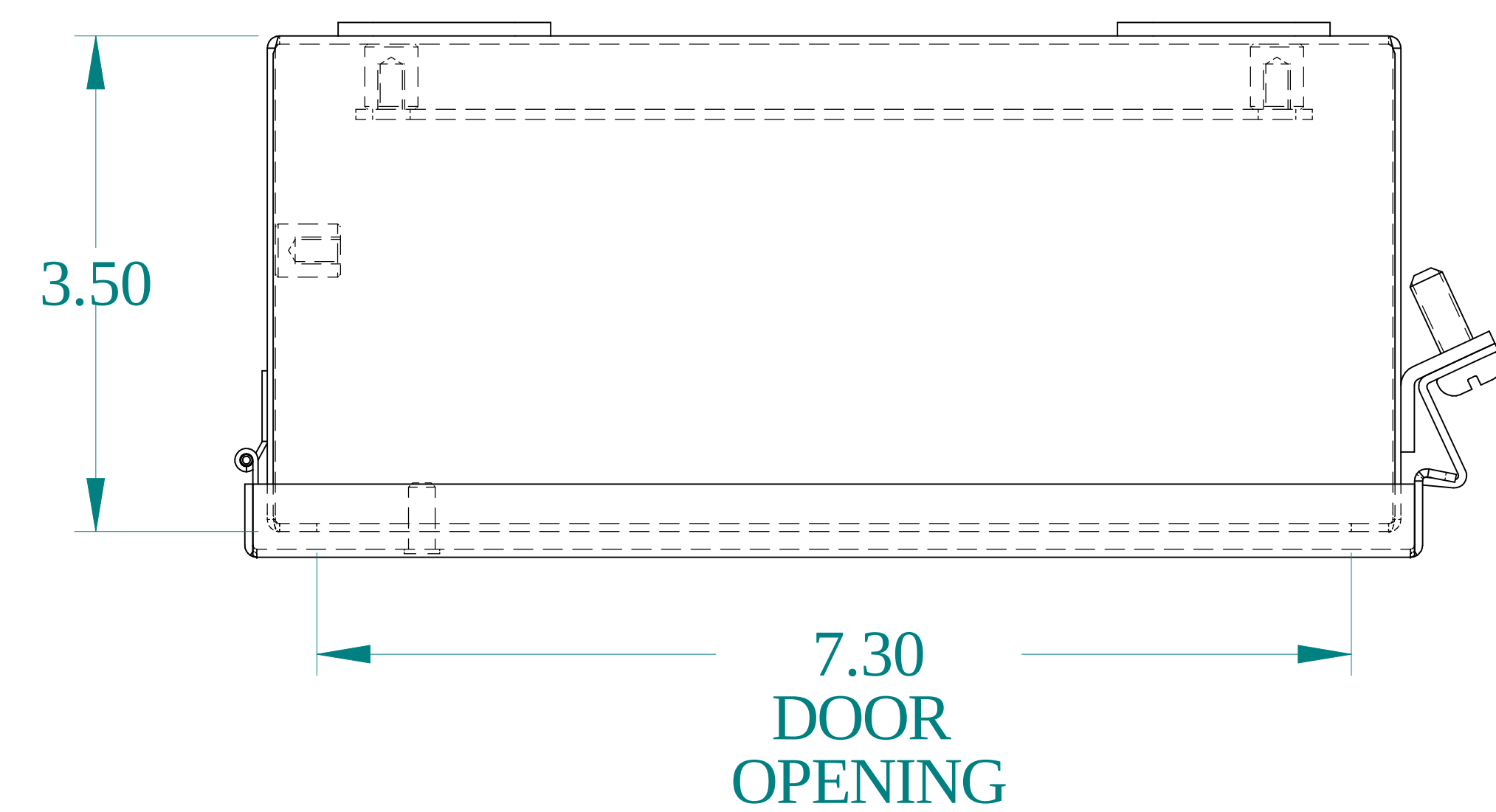
TOP VIEW
