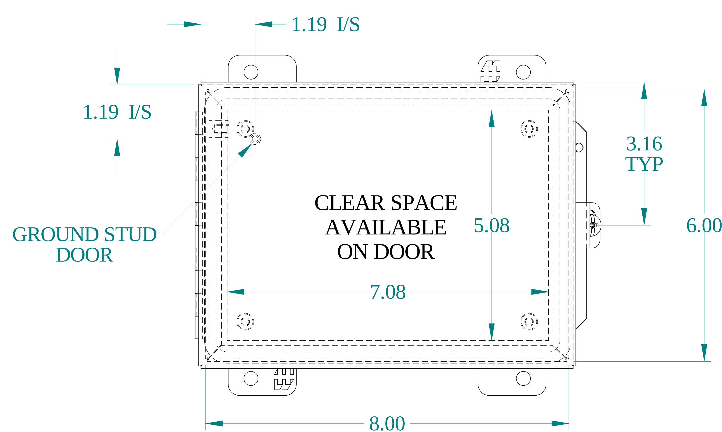
FRONT VIEW
