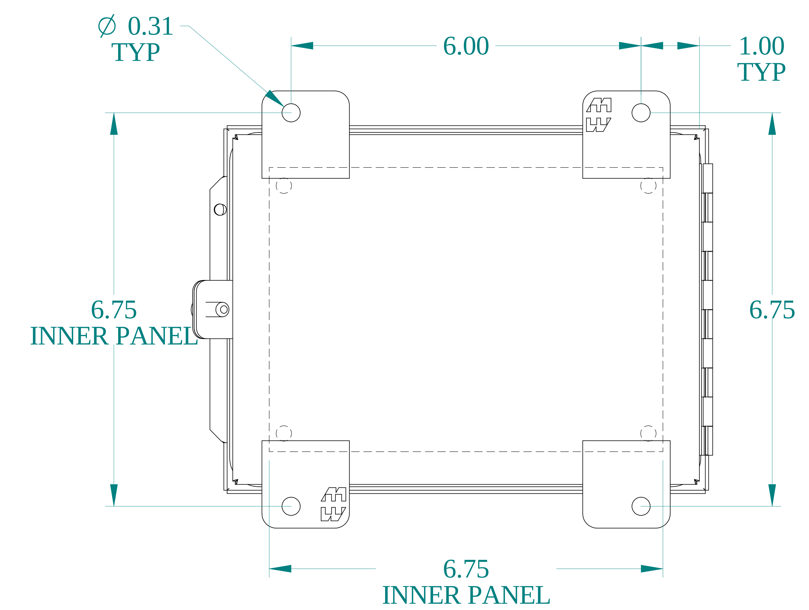
BACK VIEW
