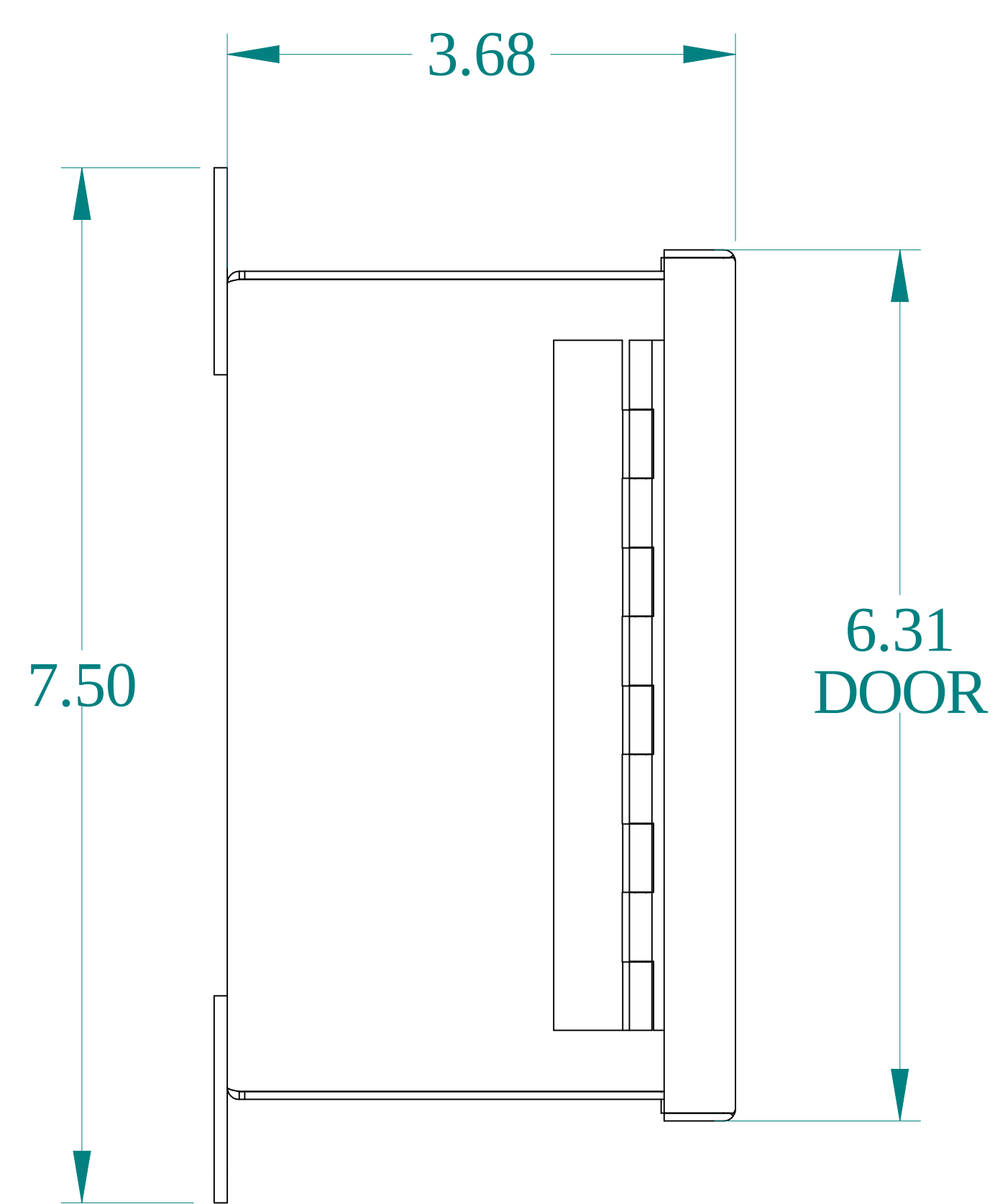
SIDE VIEW
