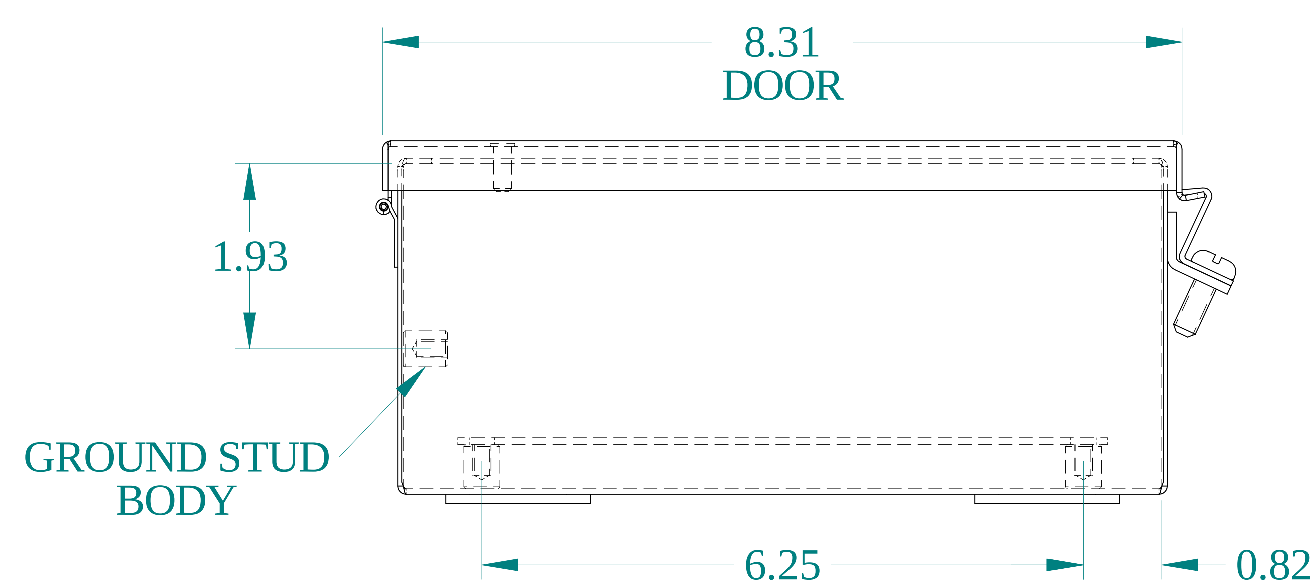
BOTTOM VIEW
