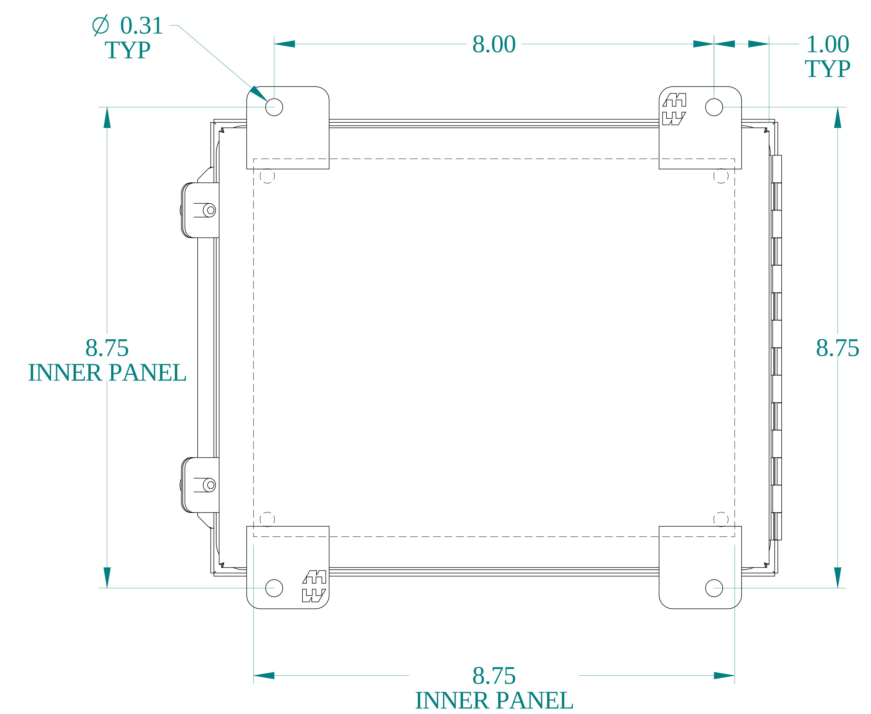
BACK VIEW
