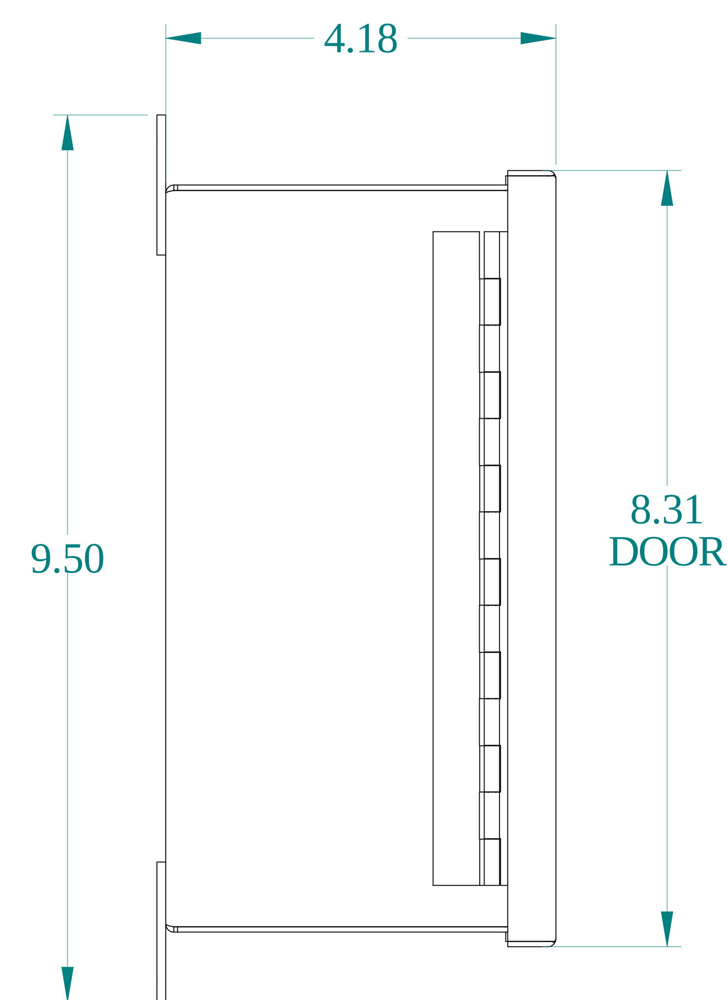
SIDE VIEW
