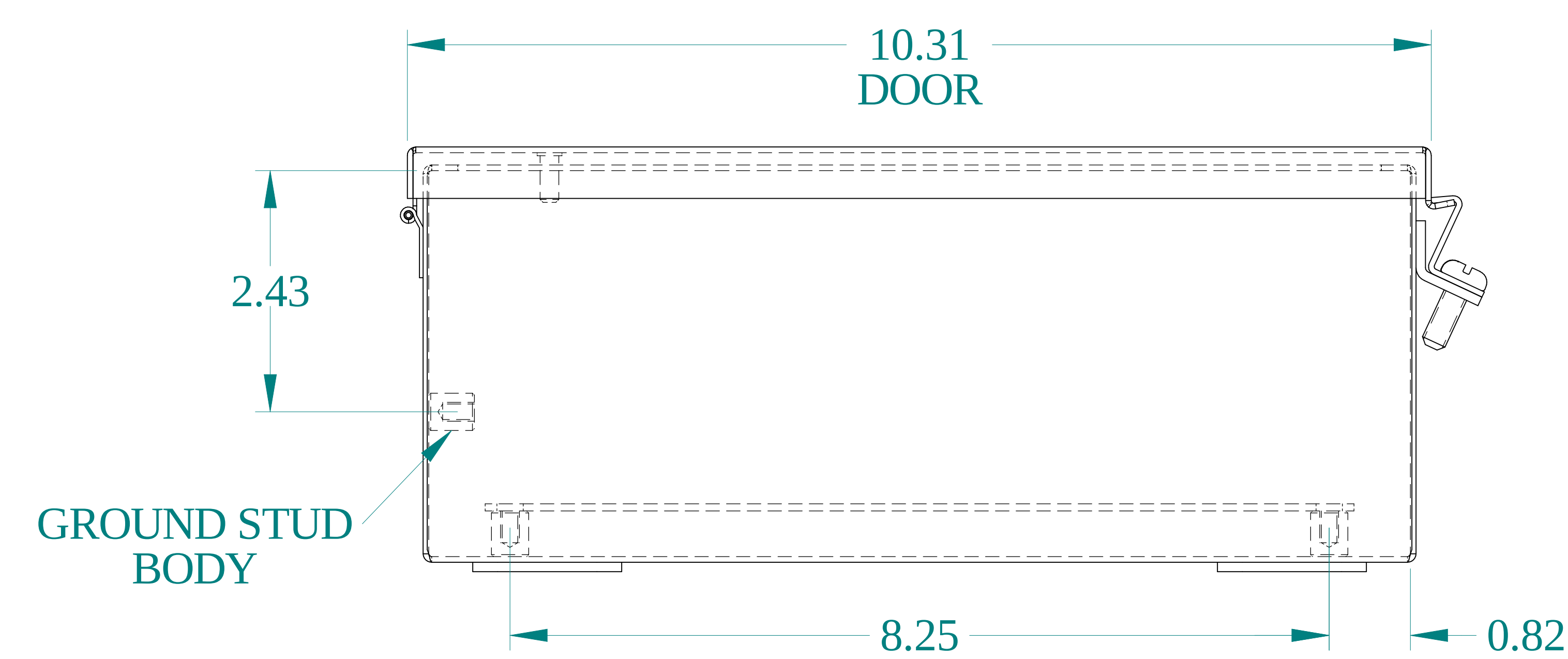
BOTTOM VIEW
