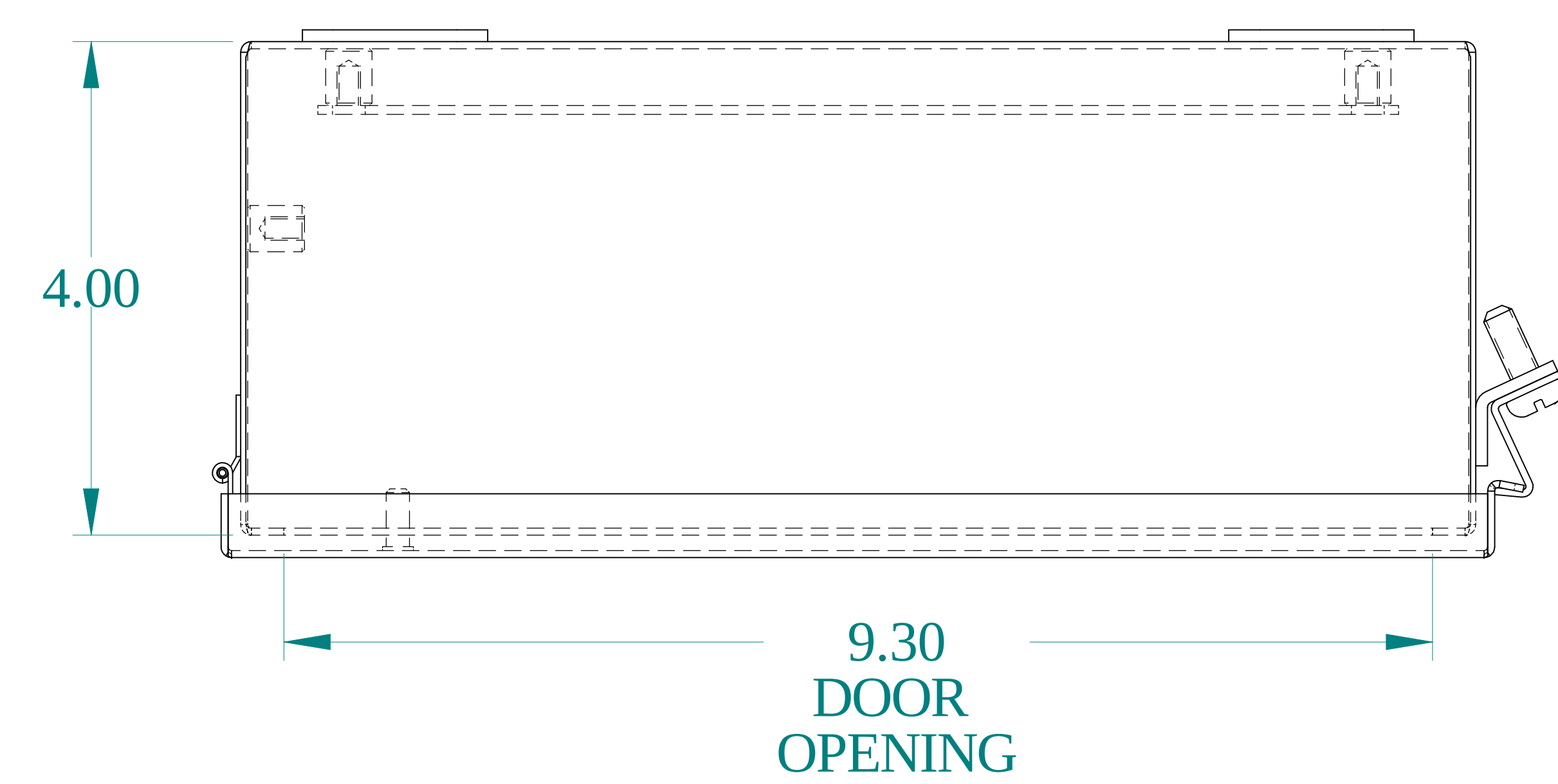
TOP VIEW
