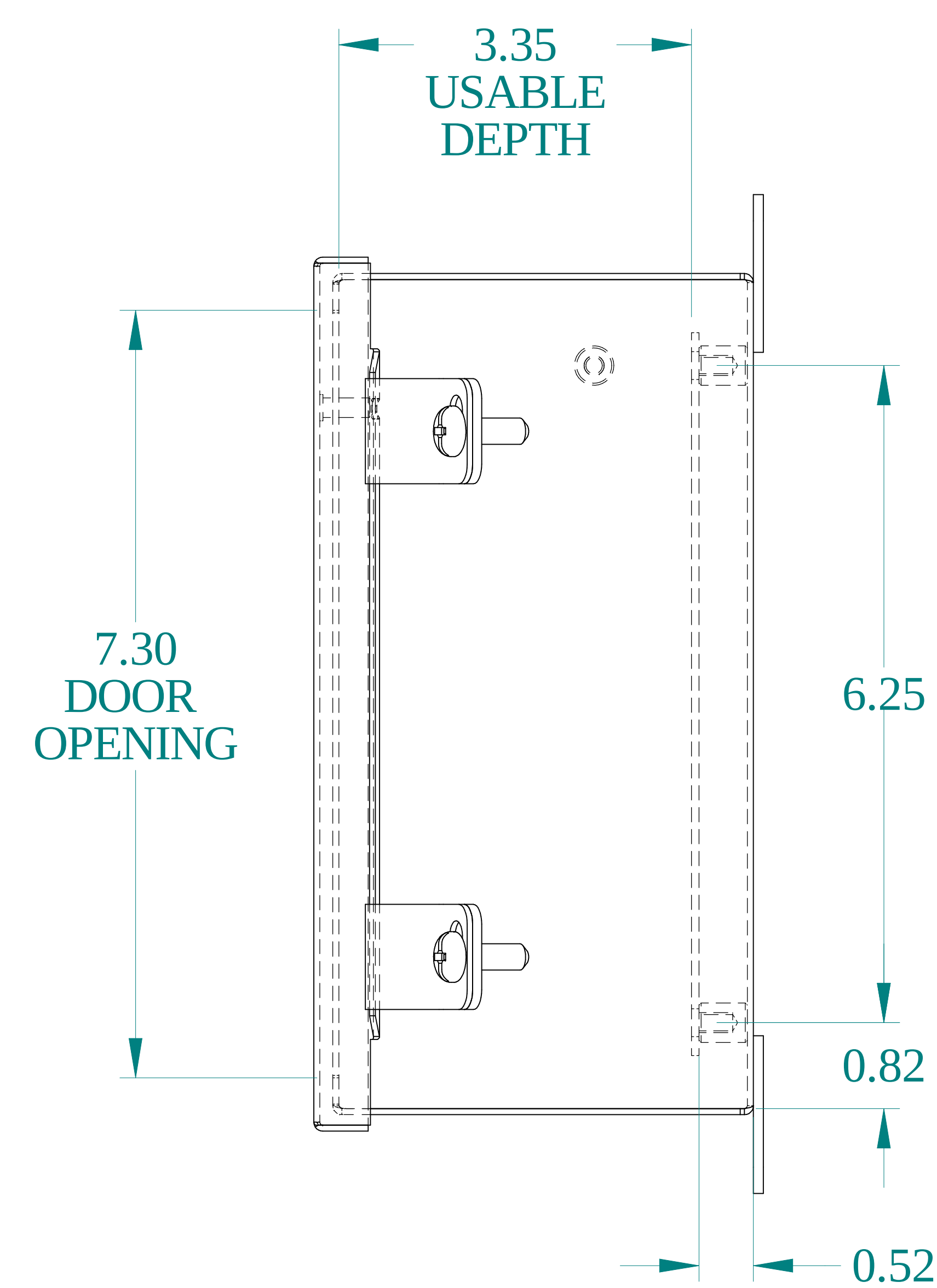
SIDE VIEW
