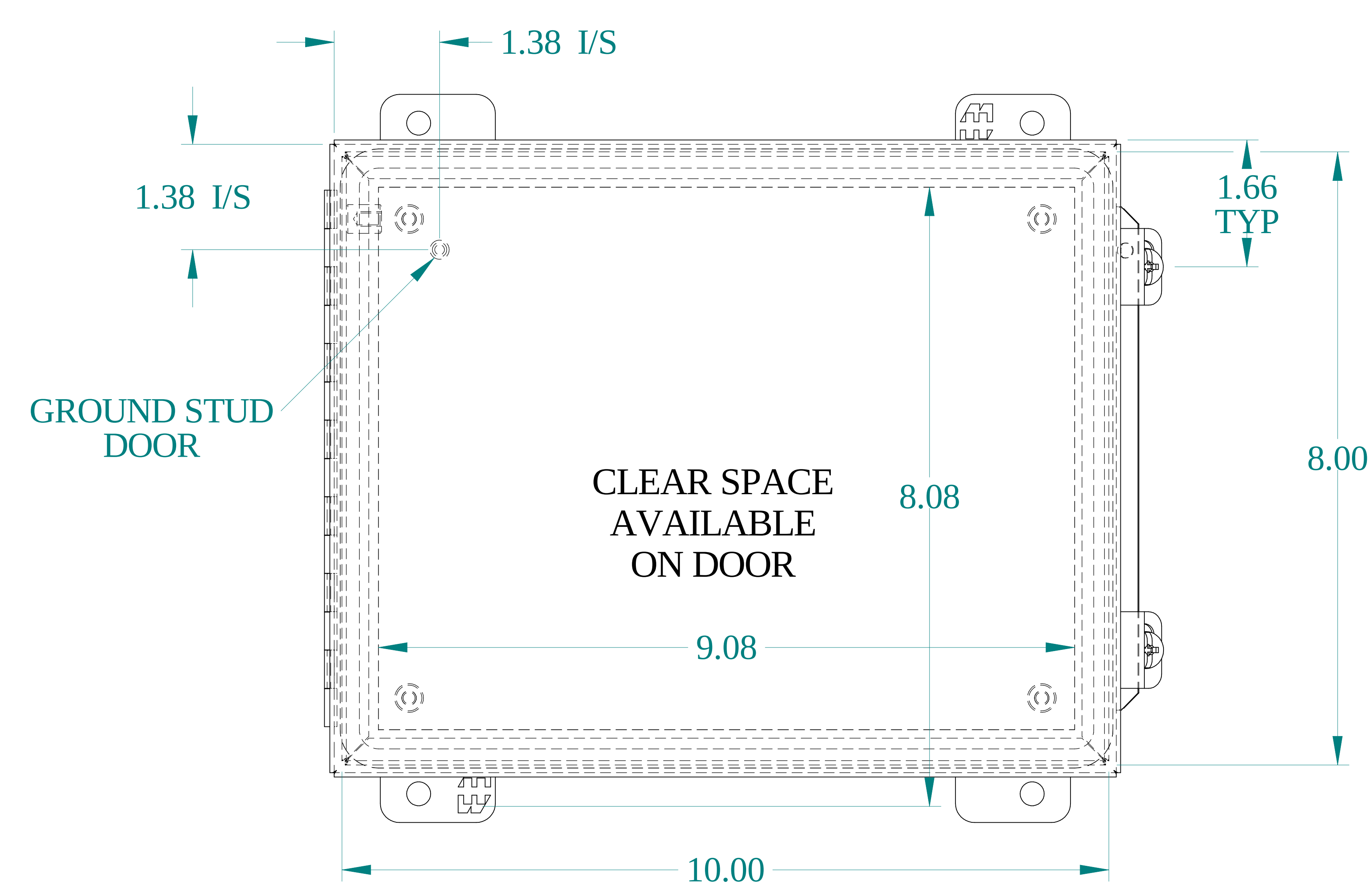
FRONT VIEW
