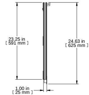
R.S. VIEW
