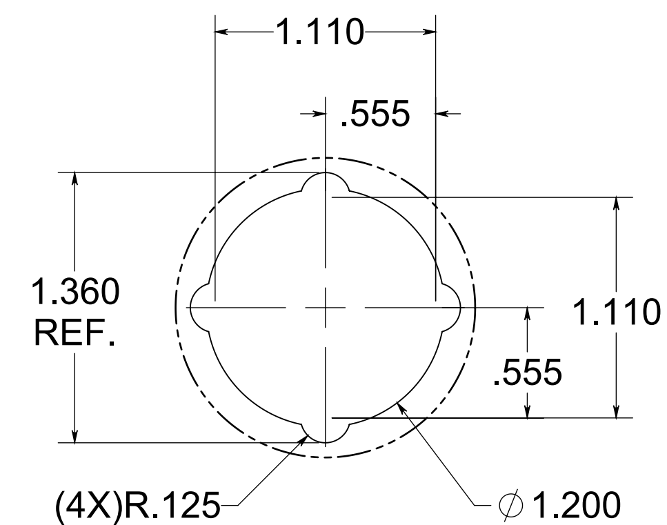
DETAIL F 30.5MM HOLE SCALE 3 : 2
