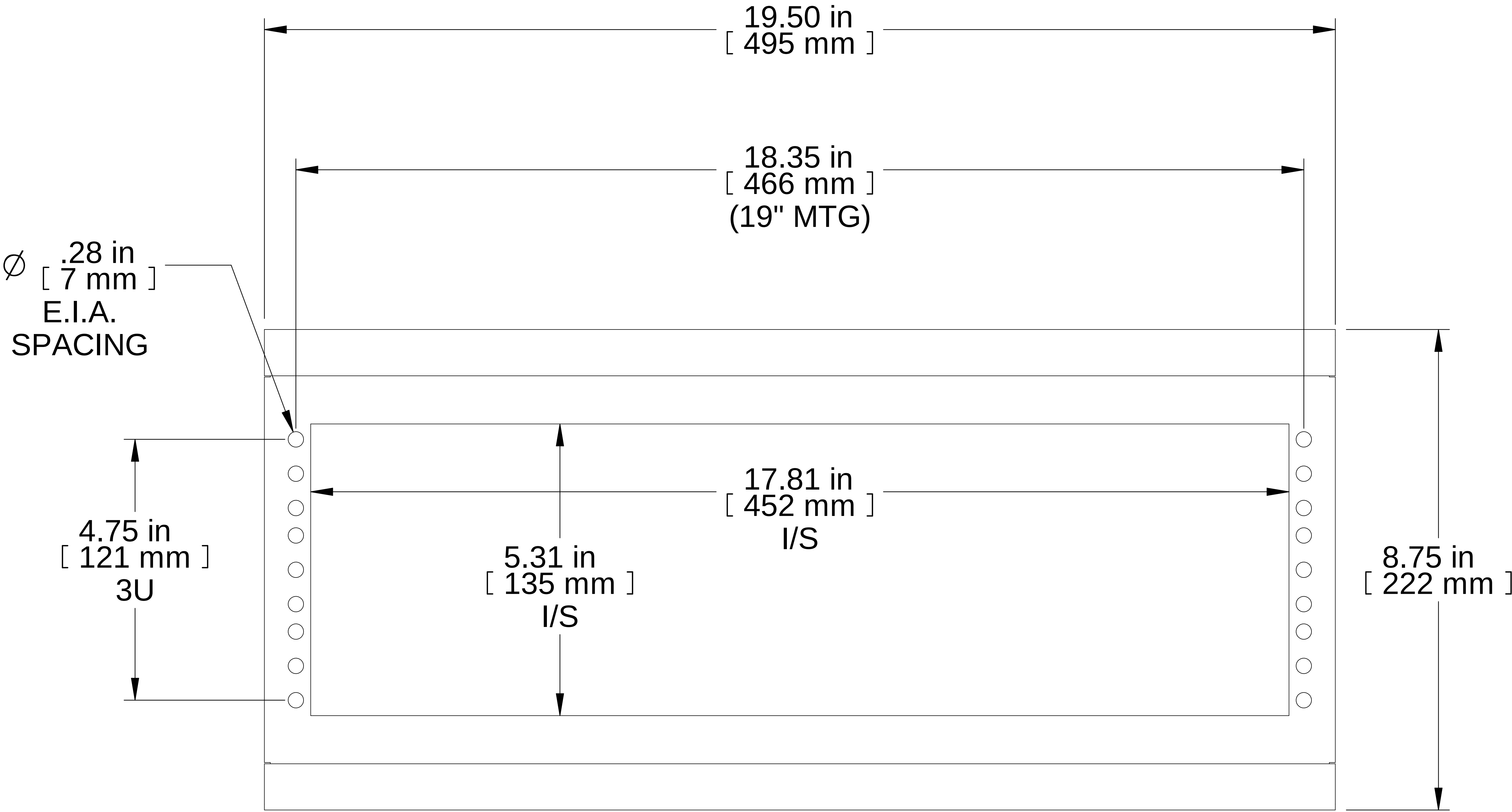
FRONT VIEW
