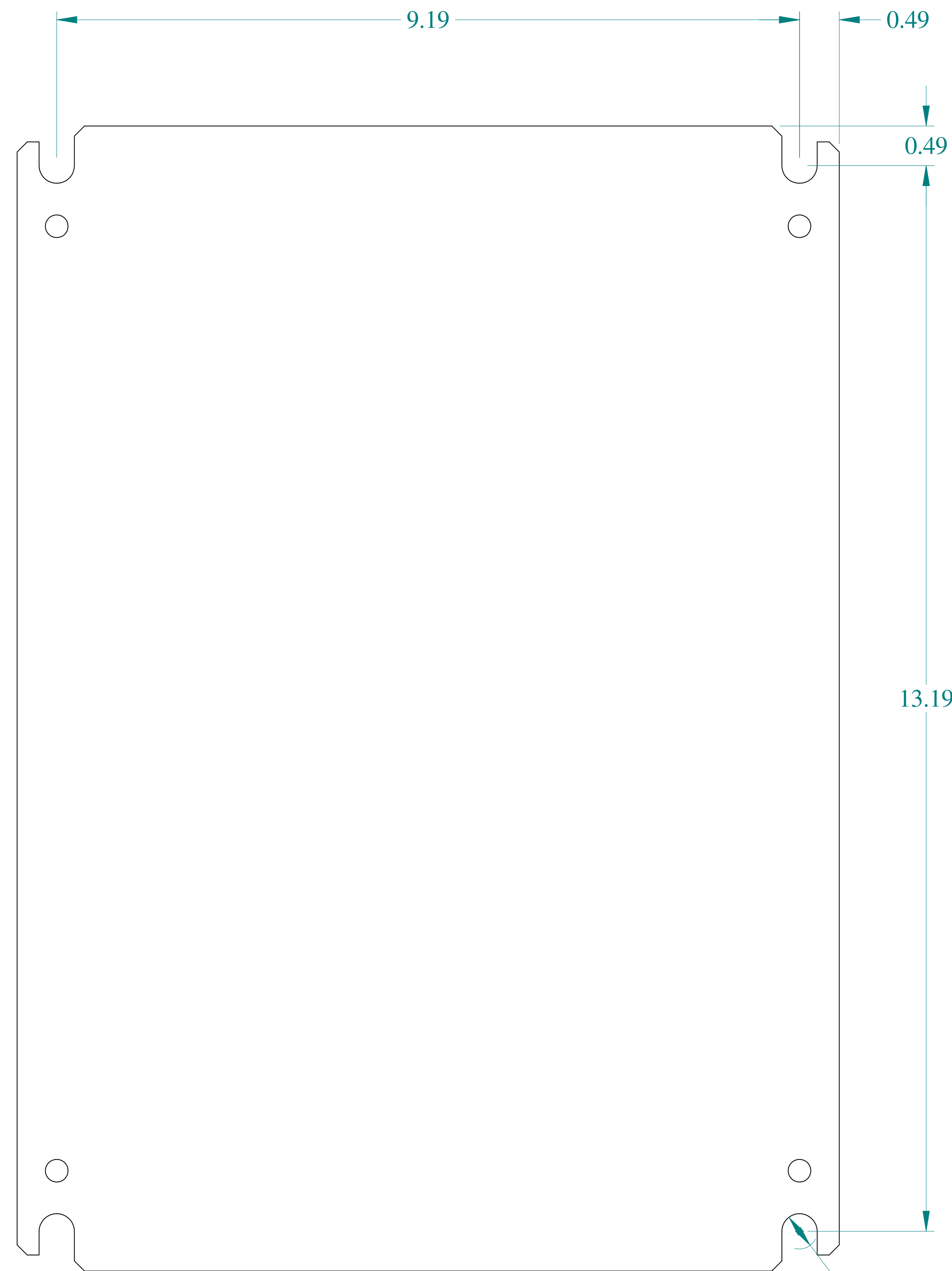
FRONT VIEW
