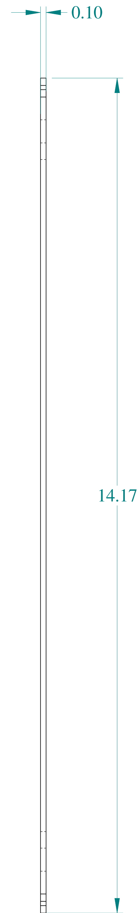
SIDE VIEW
