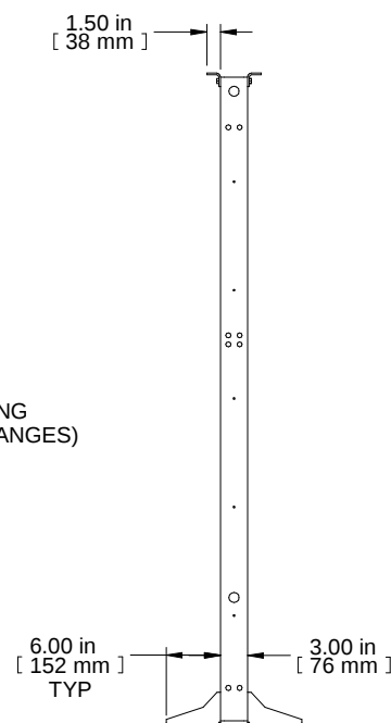
R.S. VIEW
