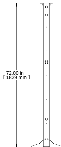
L.S. VIEW
