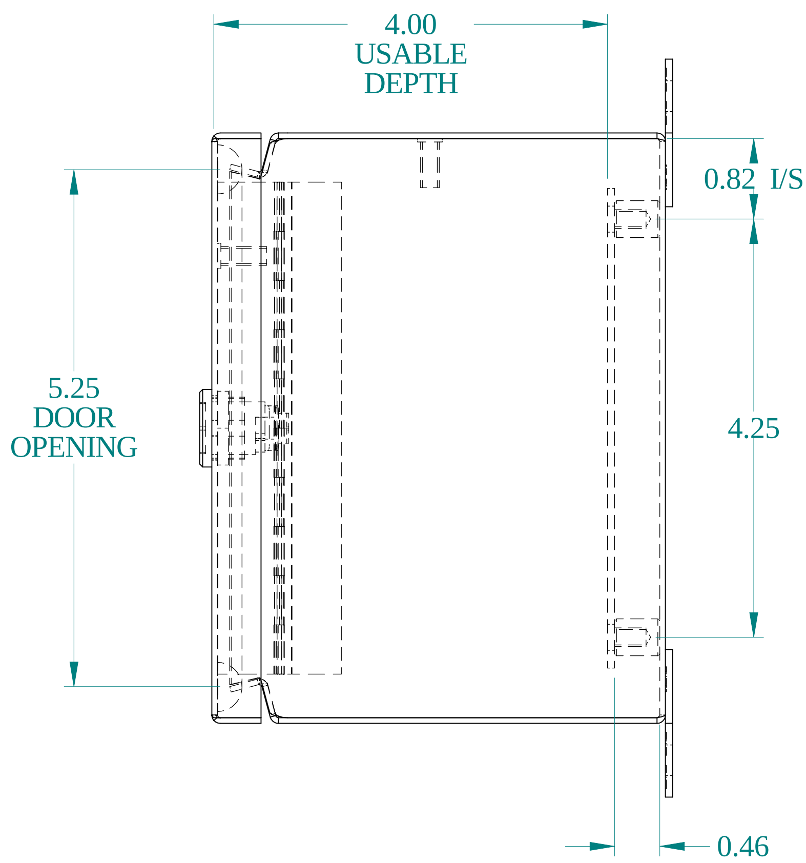
SIDE VIEW
