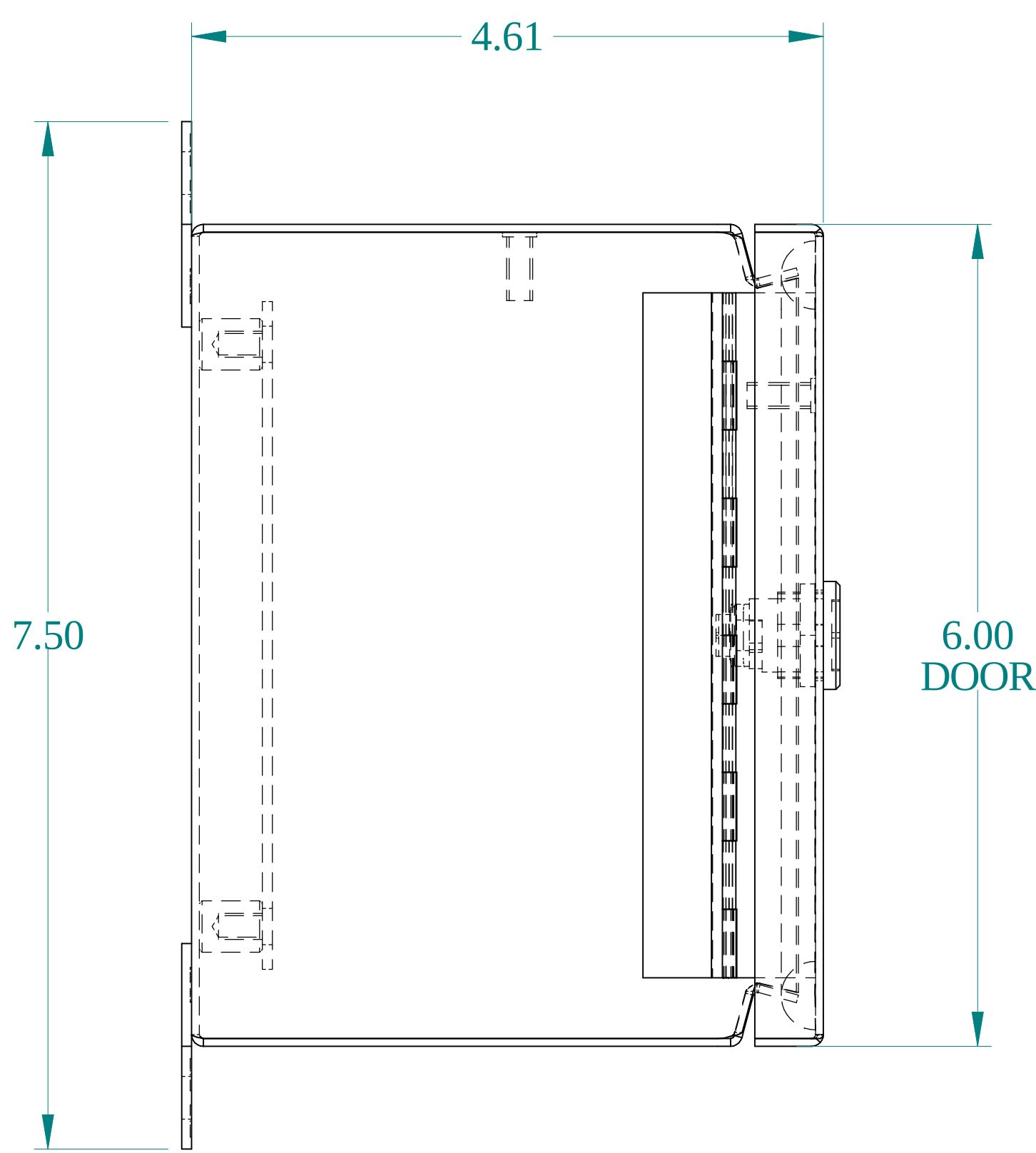
SIDE VIEW
