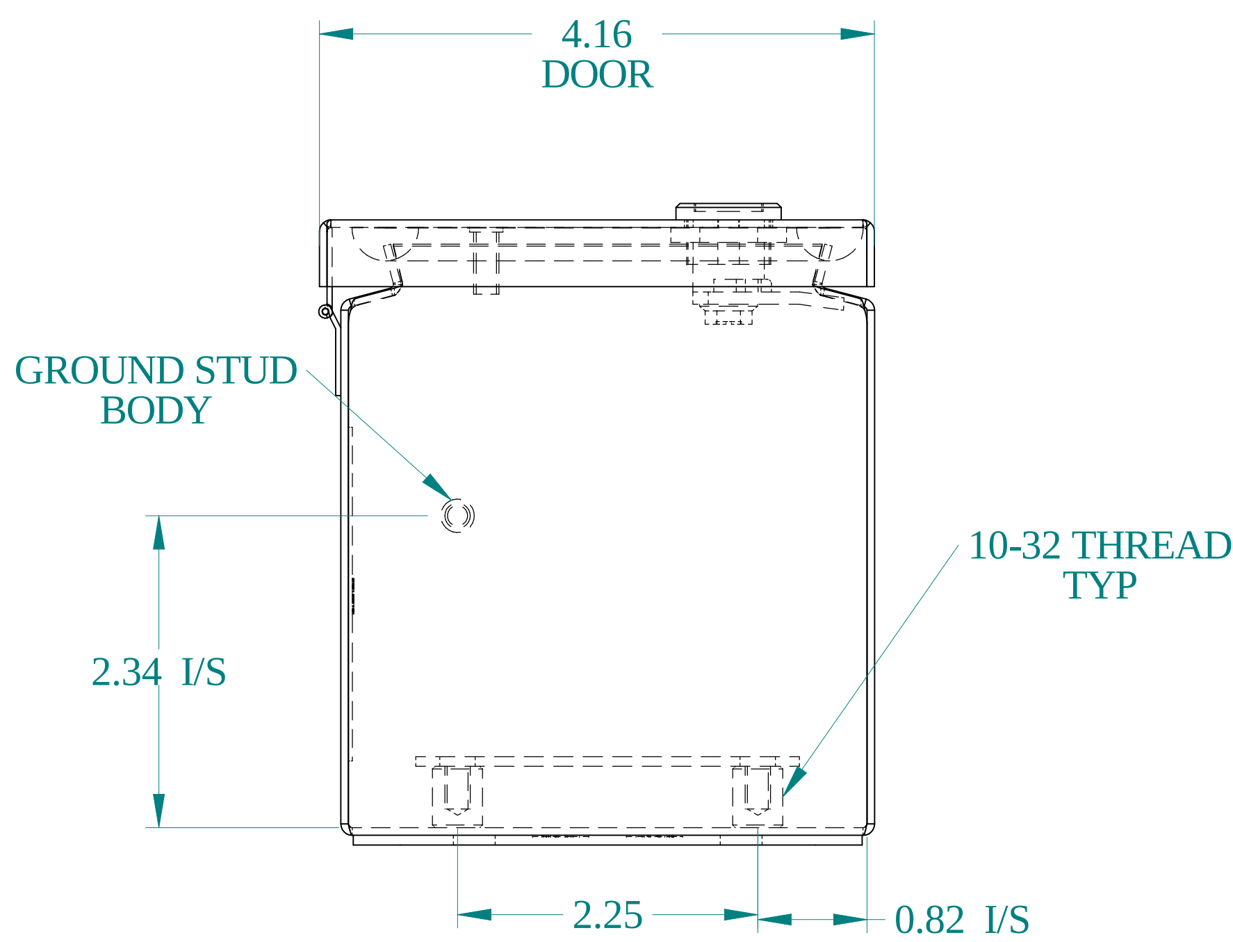
BOTTOM VIEW
