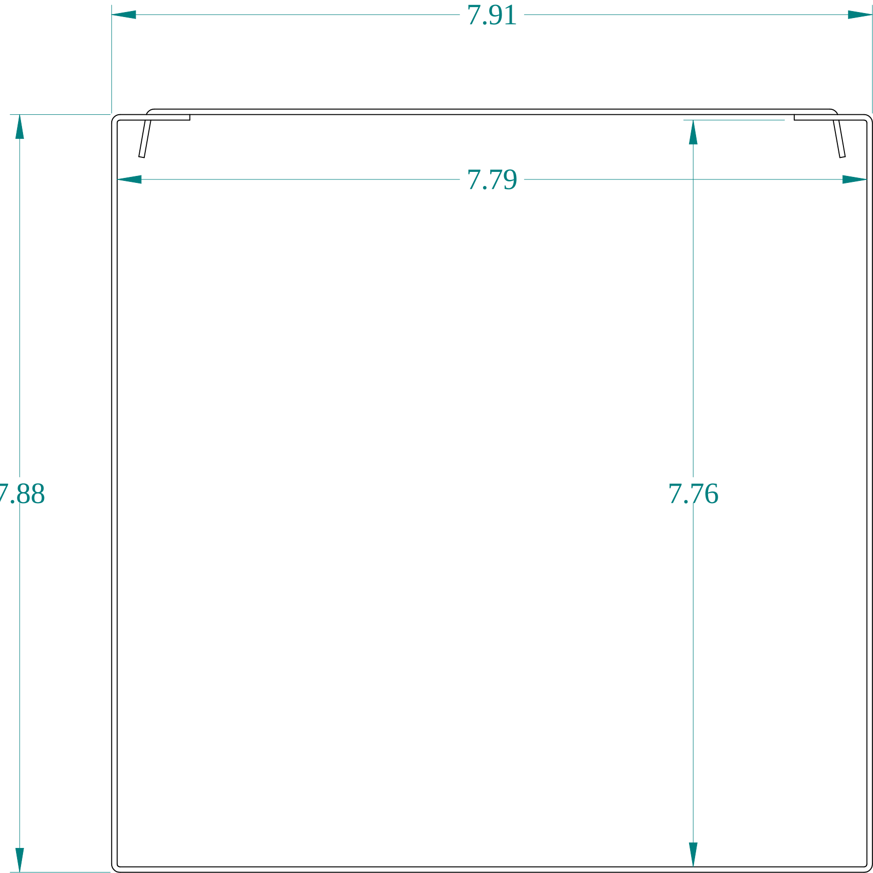
FRONT VIEW
