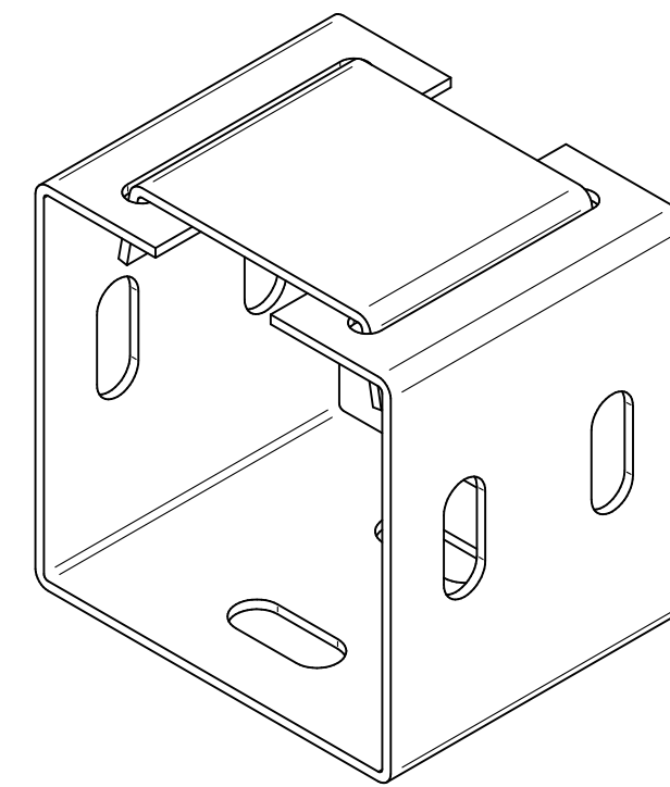
ISOMETRIC VIEWS
