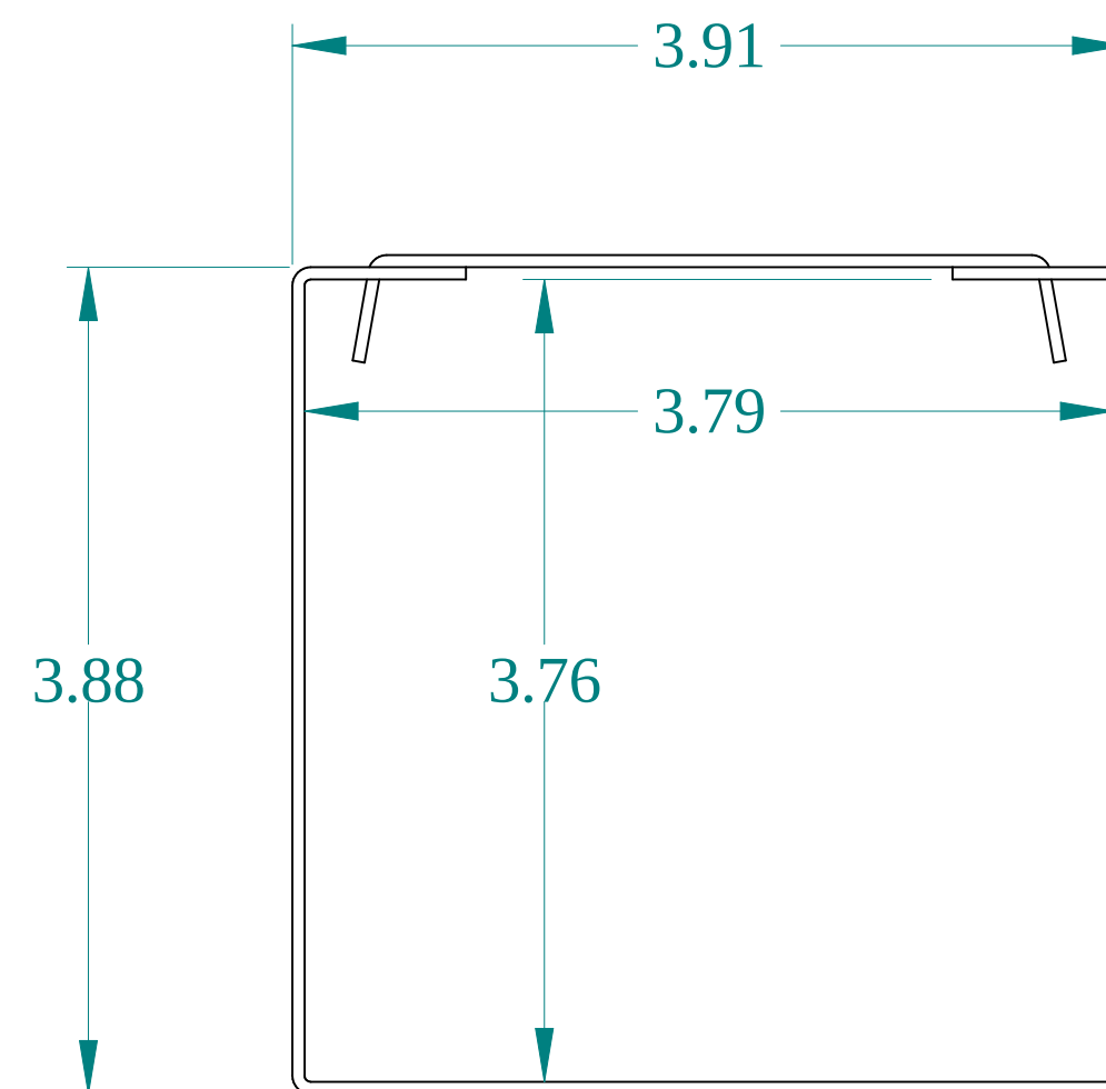
FRONT VIEW
