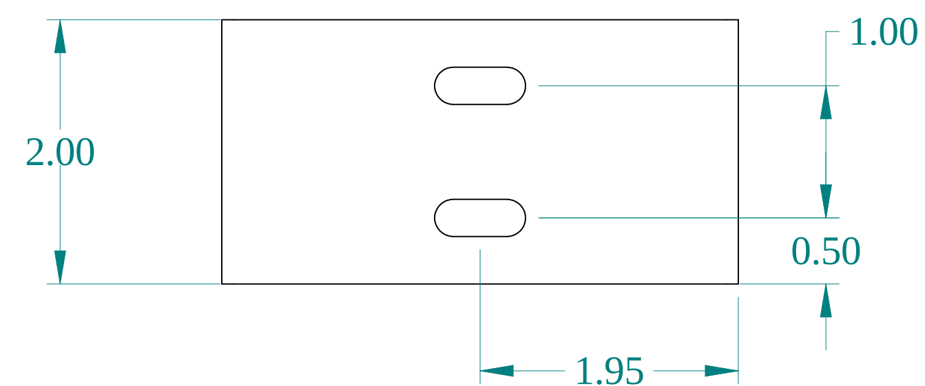
BOTTOM VIEW
