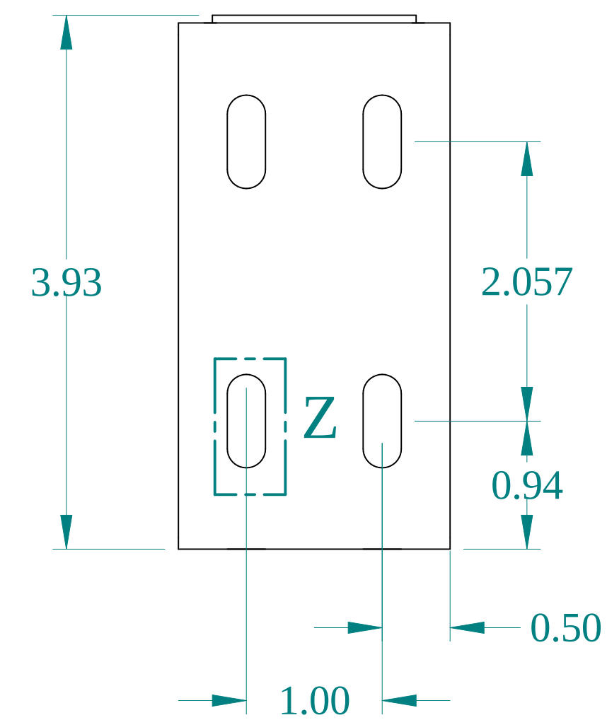
SIDE VIEW
