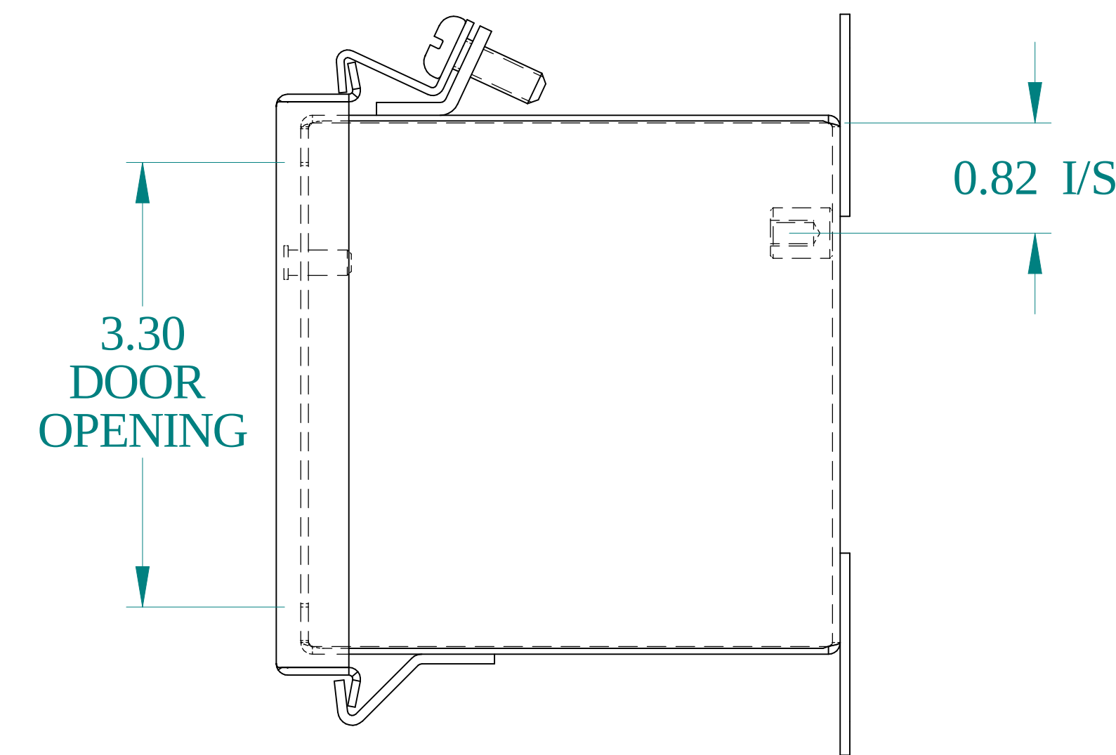
SIDE VIEW
