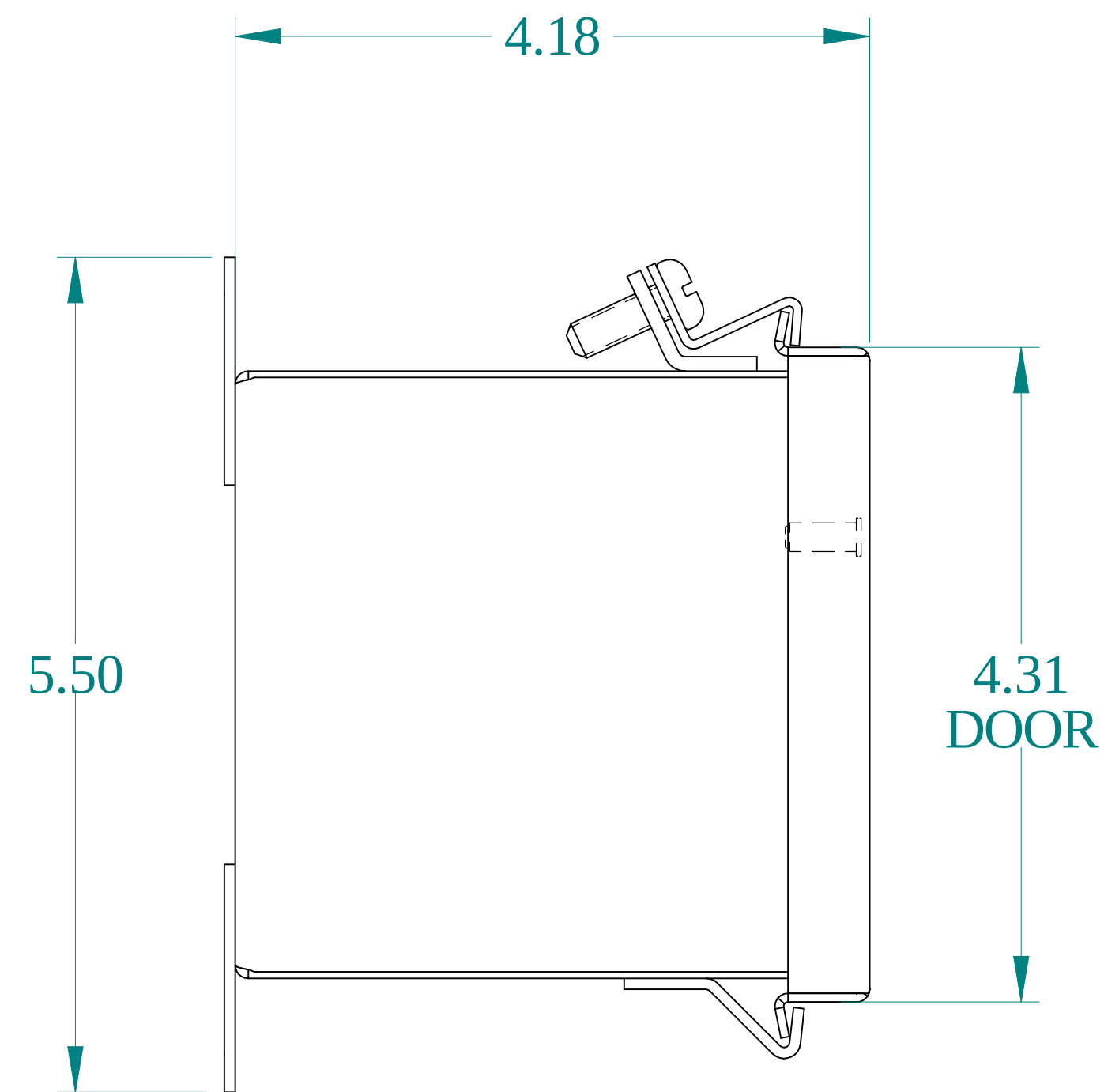
SIDE VIEW
