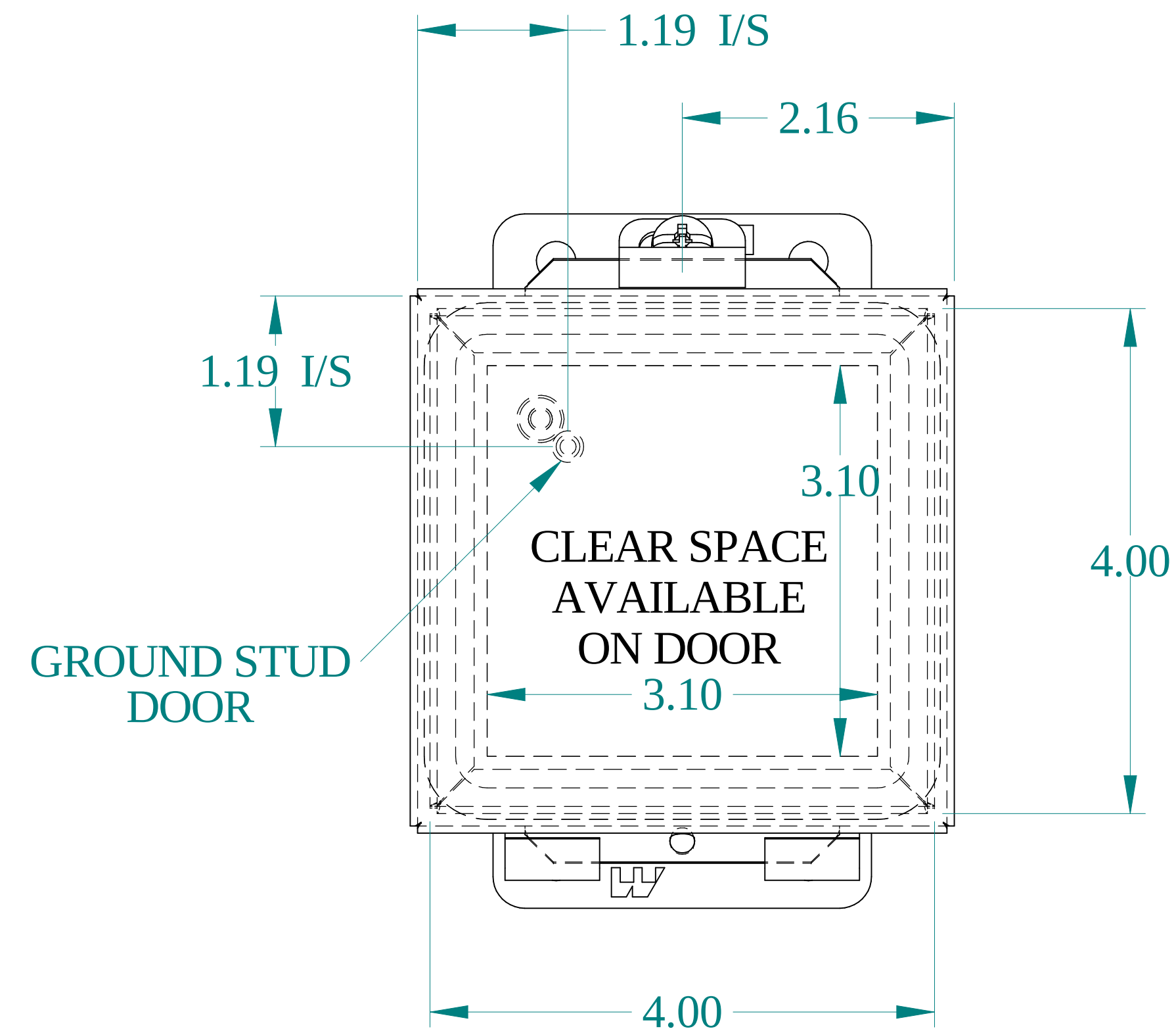
FRONT VIEW
