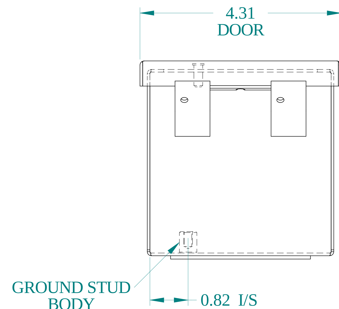
BOTTOM VIEW
