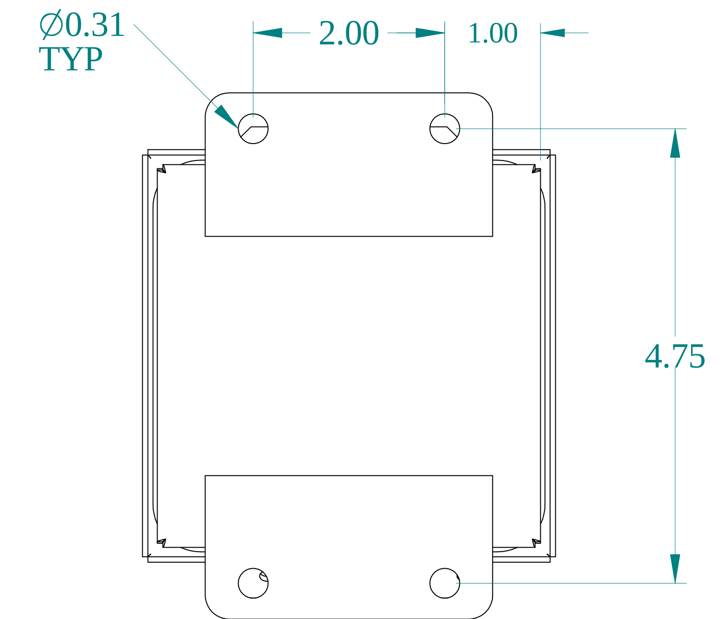
BACK VIEW
