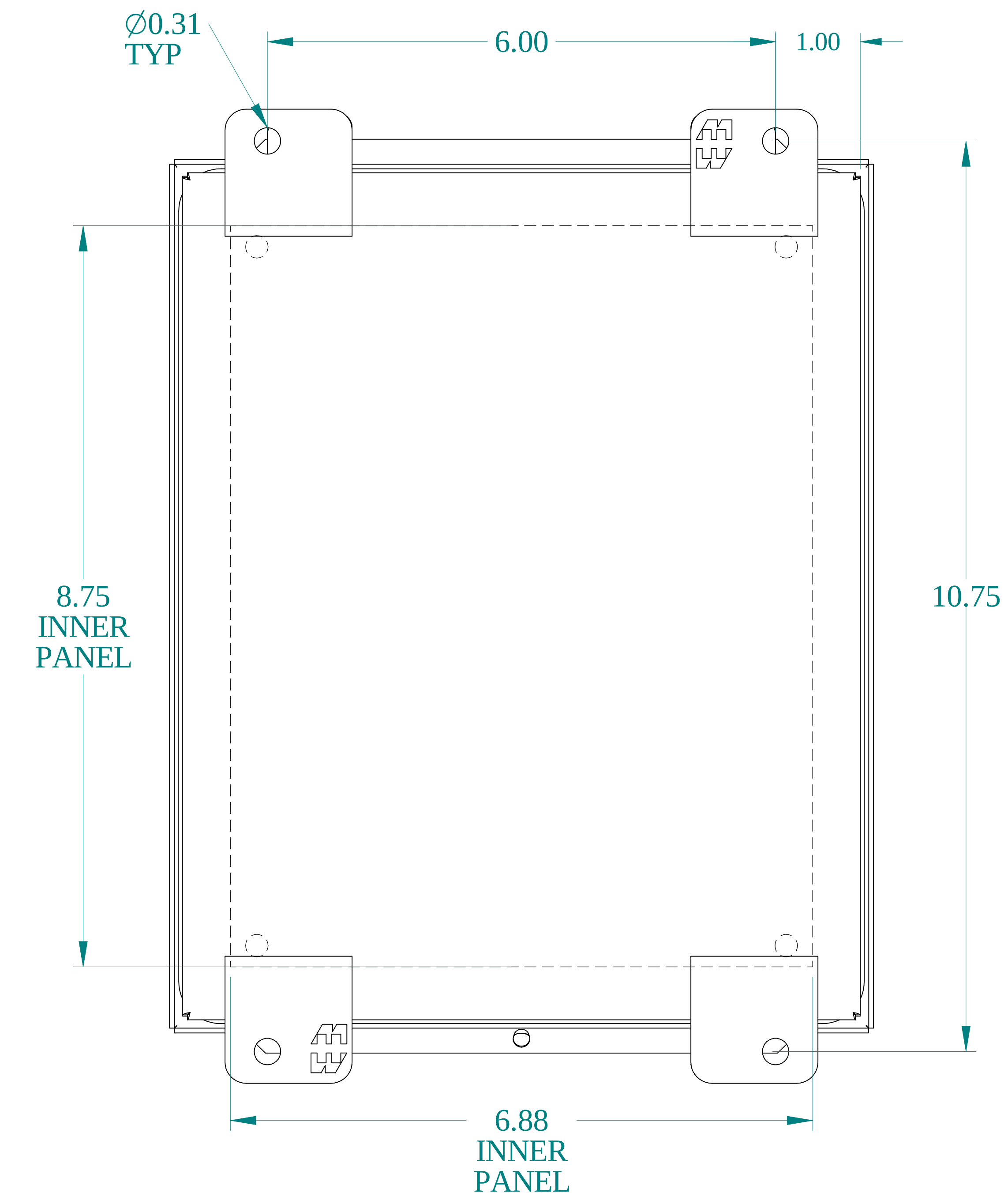
BACK VIEW
