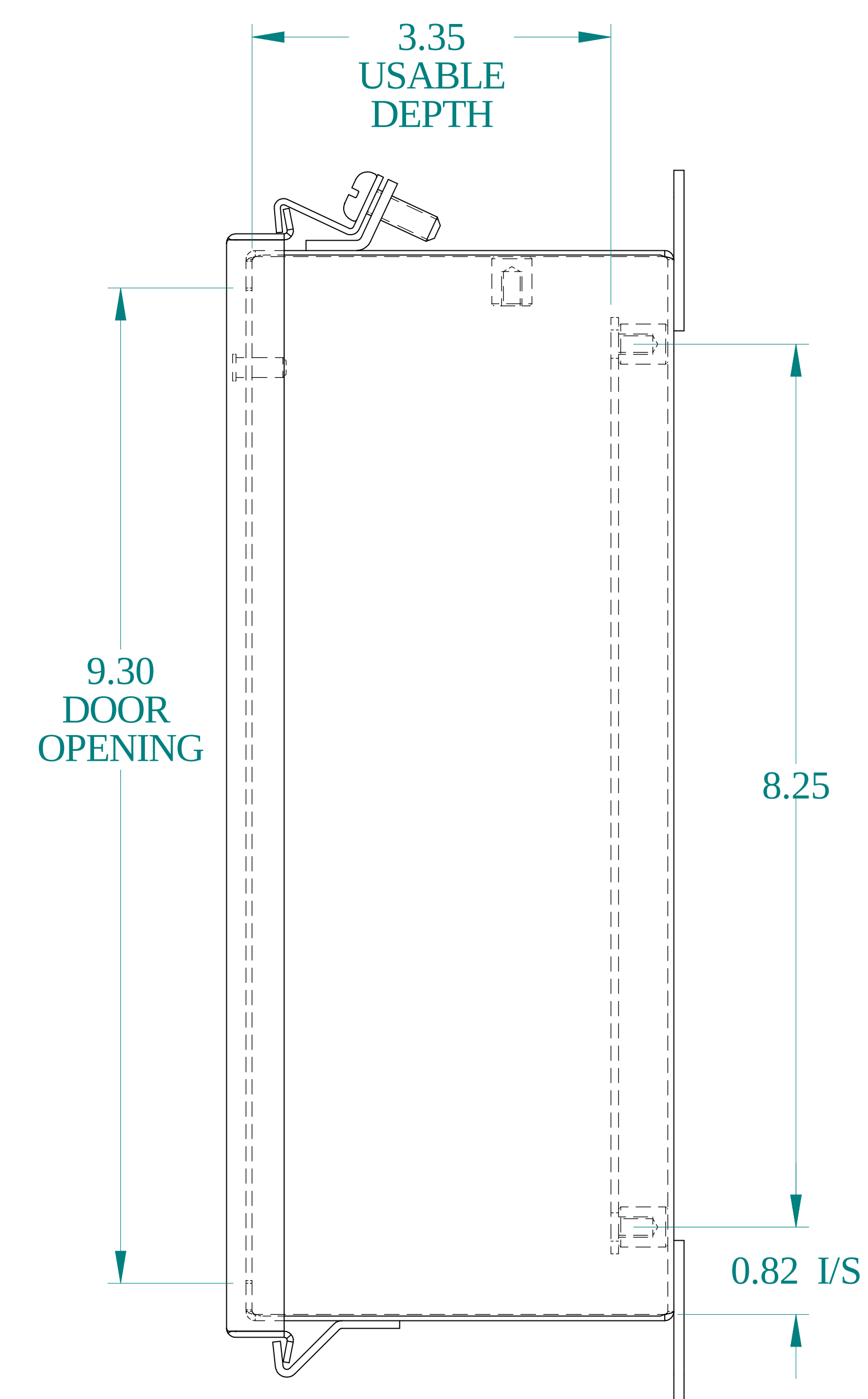
SIDE VIEW
