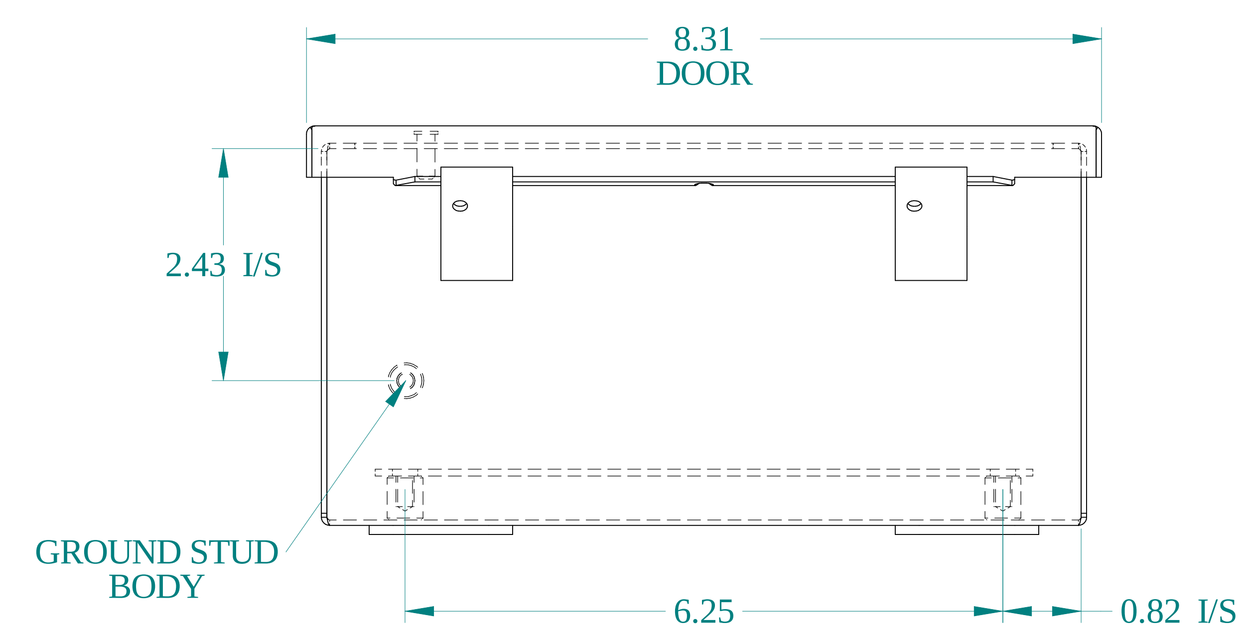
BOTTOM VIEW
