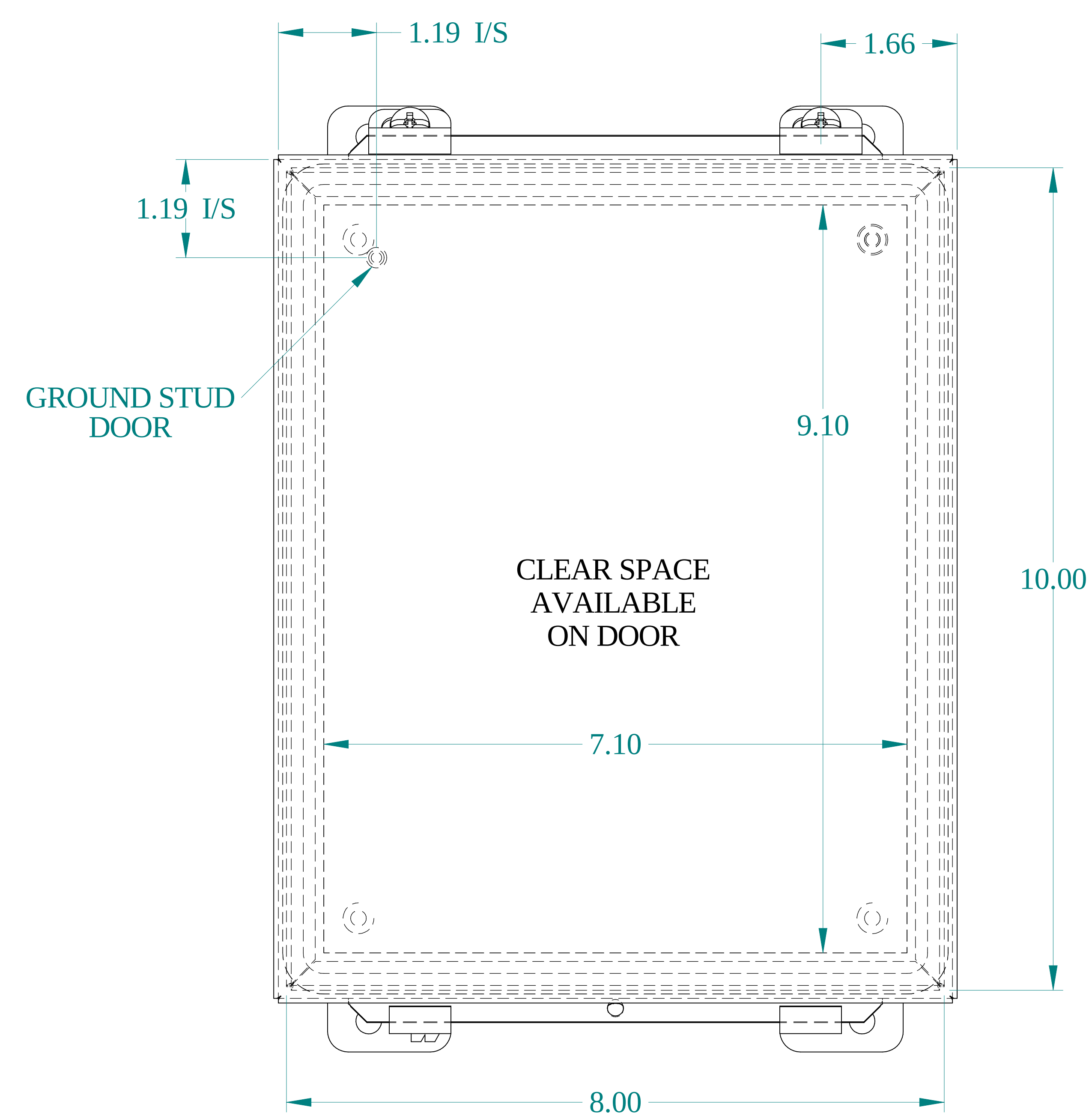
FRONT VIEW
