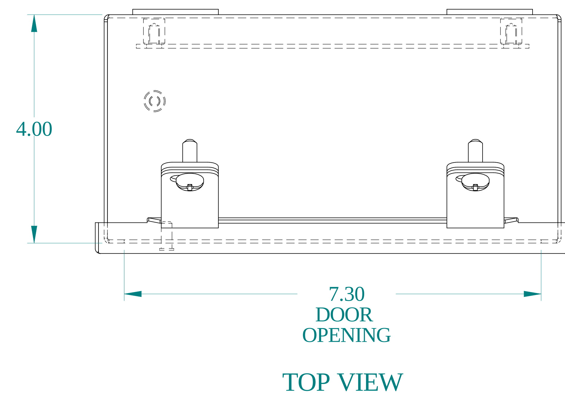
TOP VIEW
