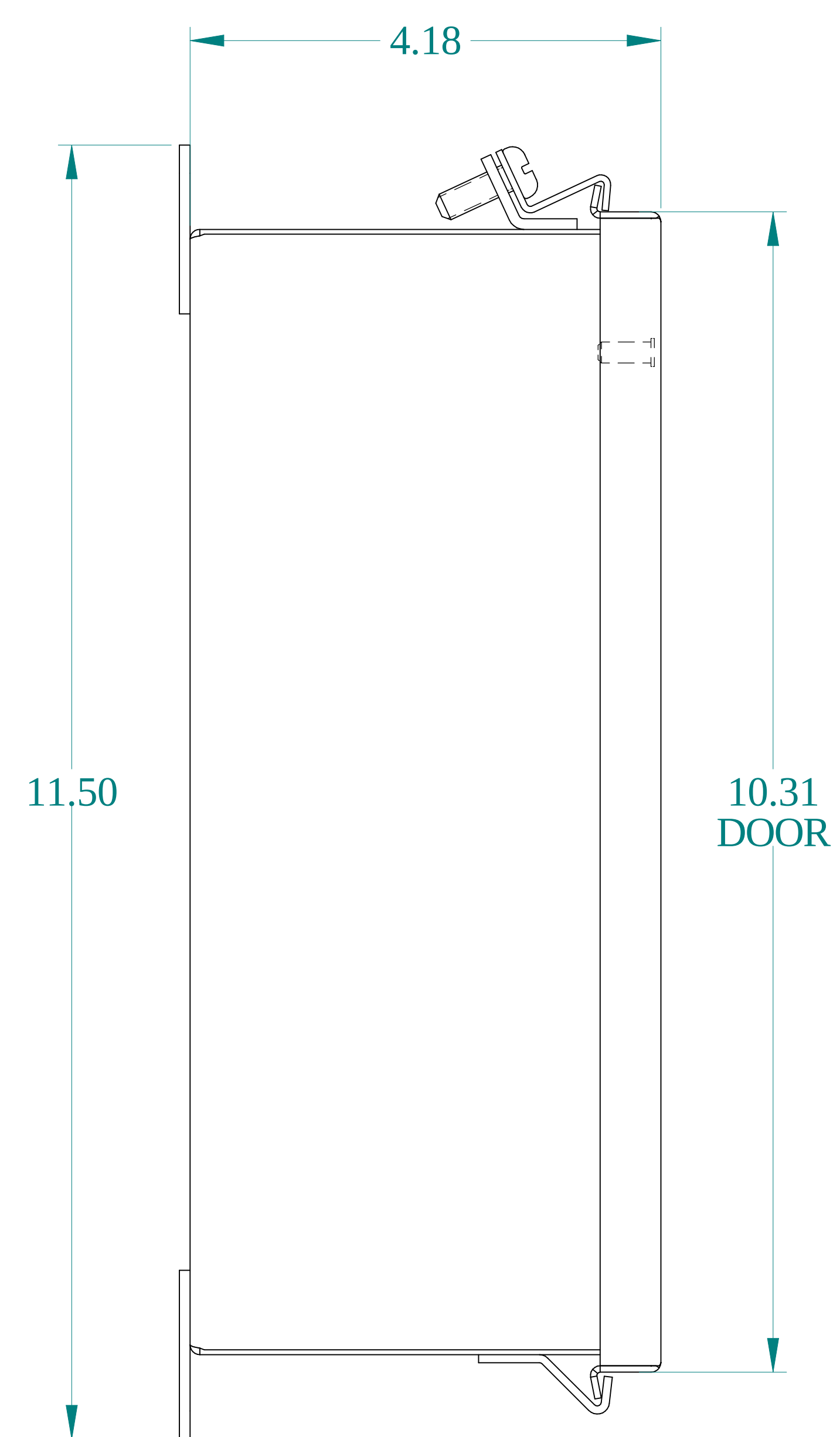
SIDE VIEW
