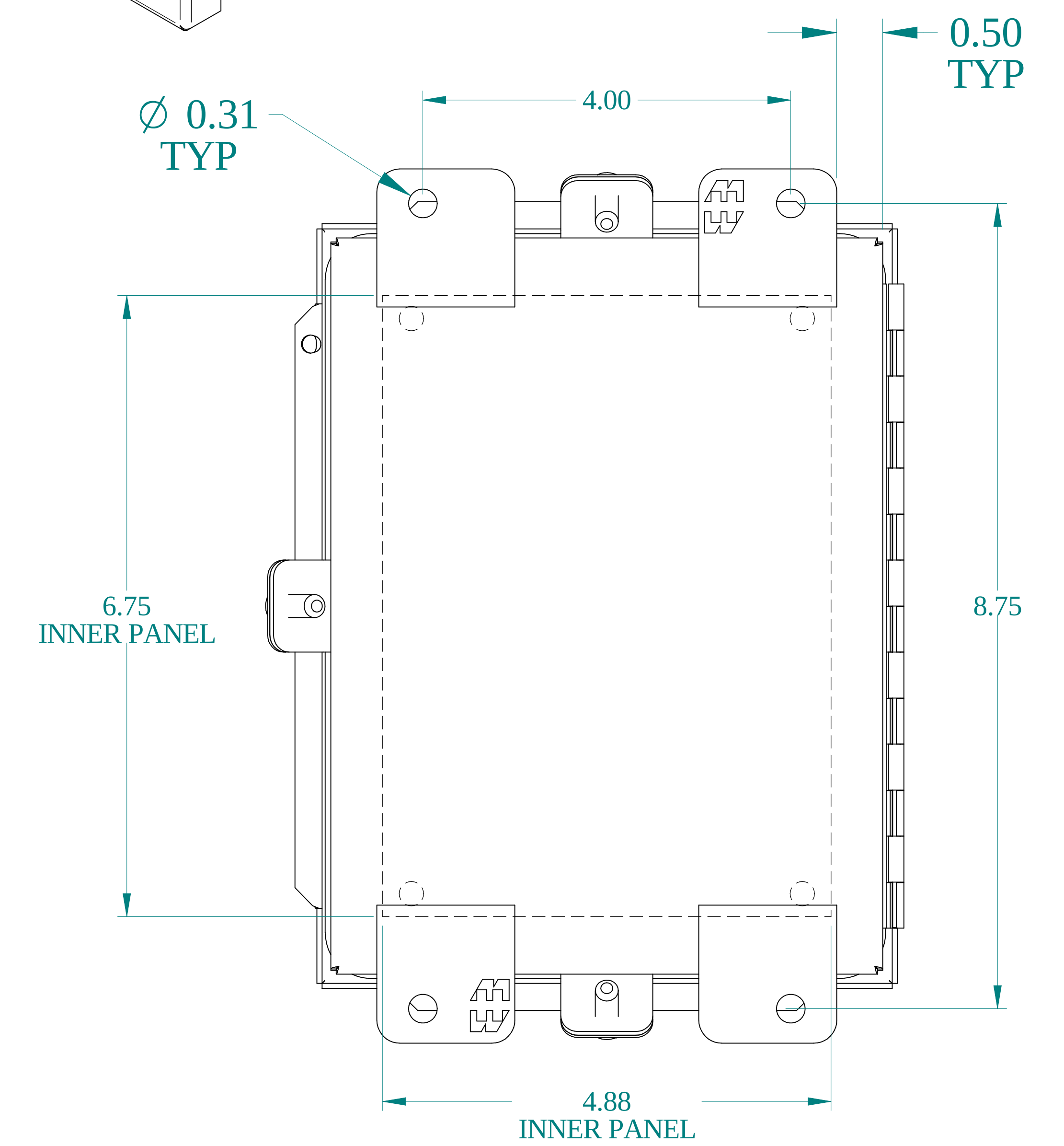
BACK VIEW
