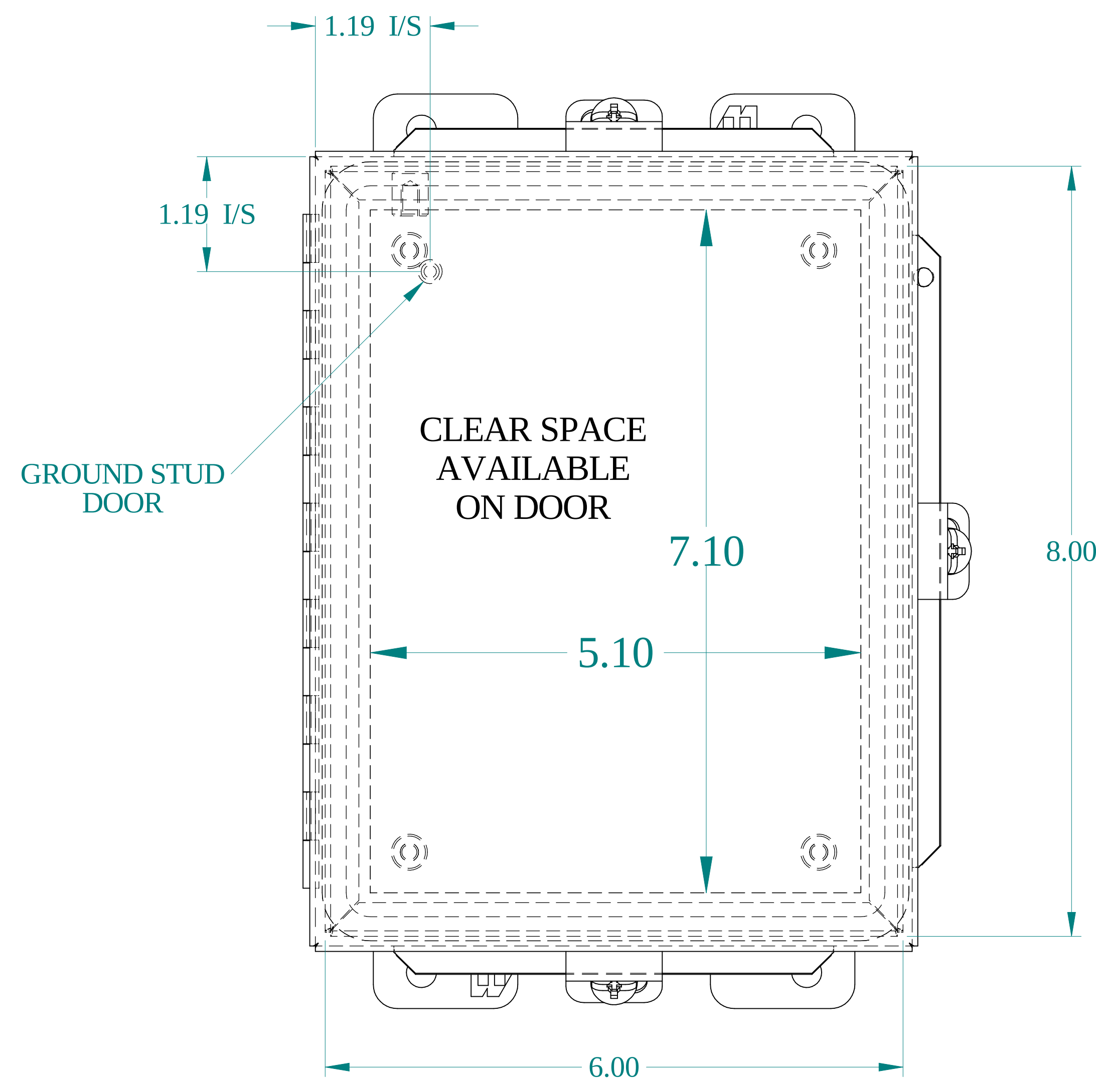
FRONT VIEW
