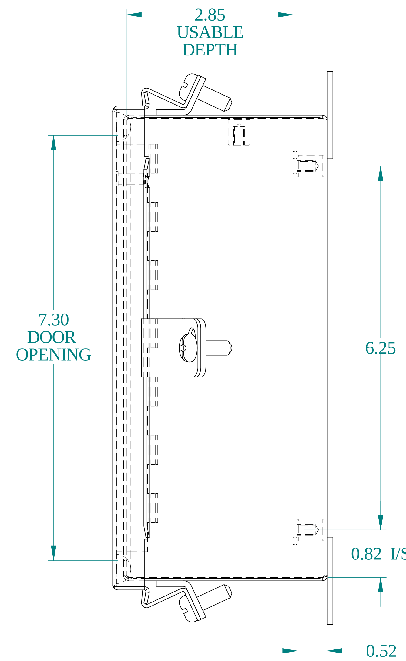
SIDE VIEW
