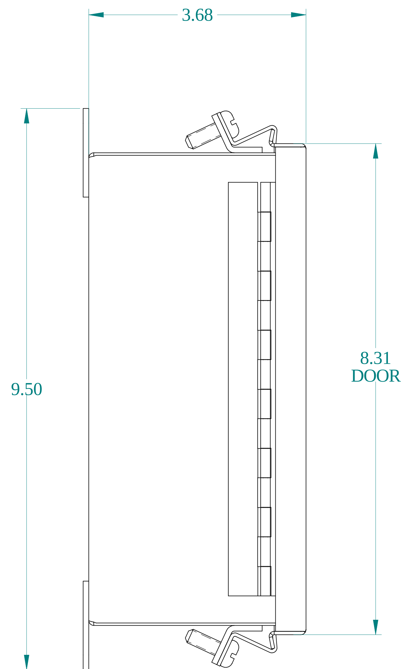
SIDE VIEW
