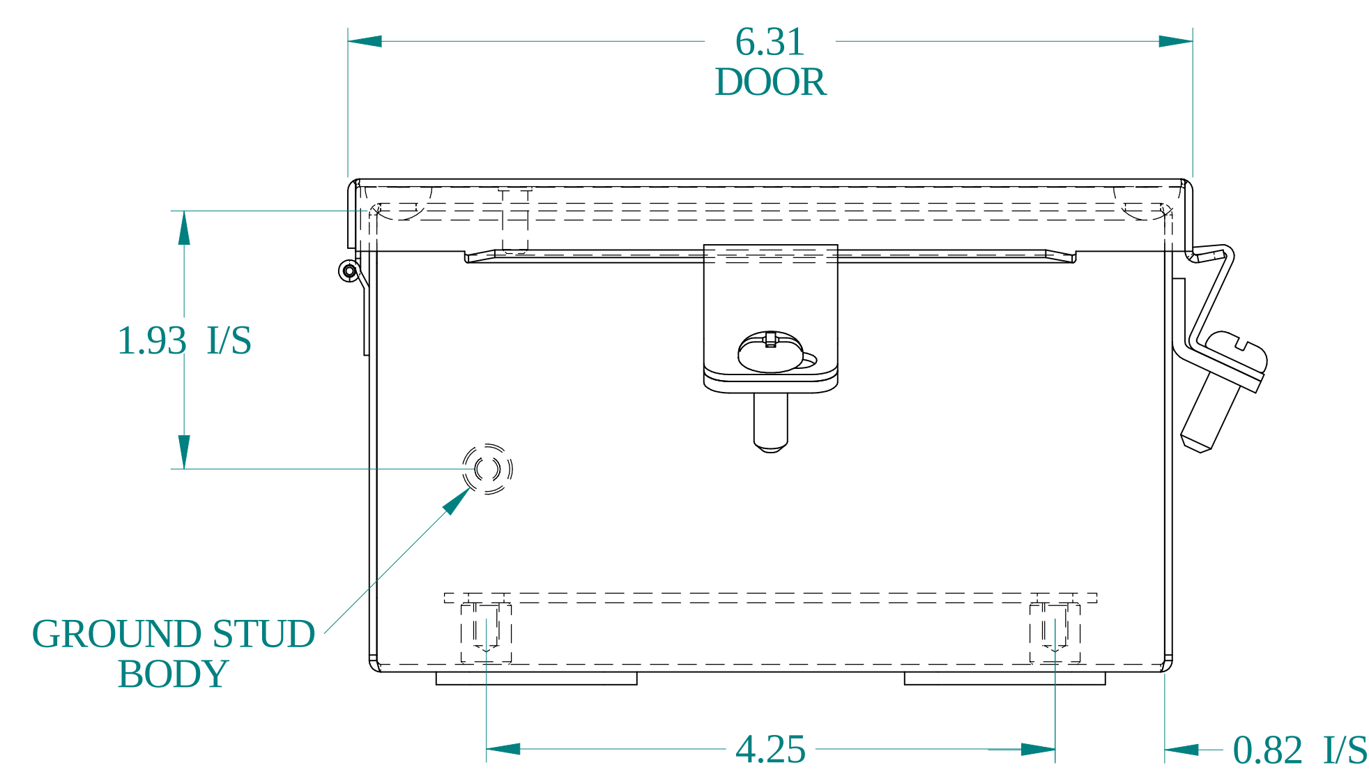
BOTTOM VIEW
