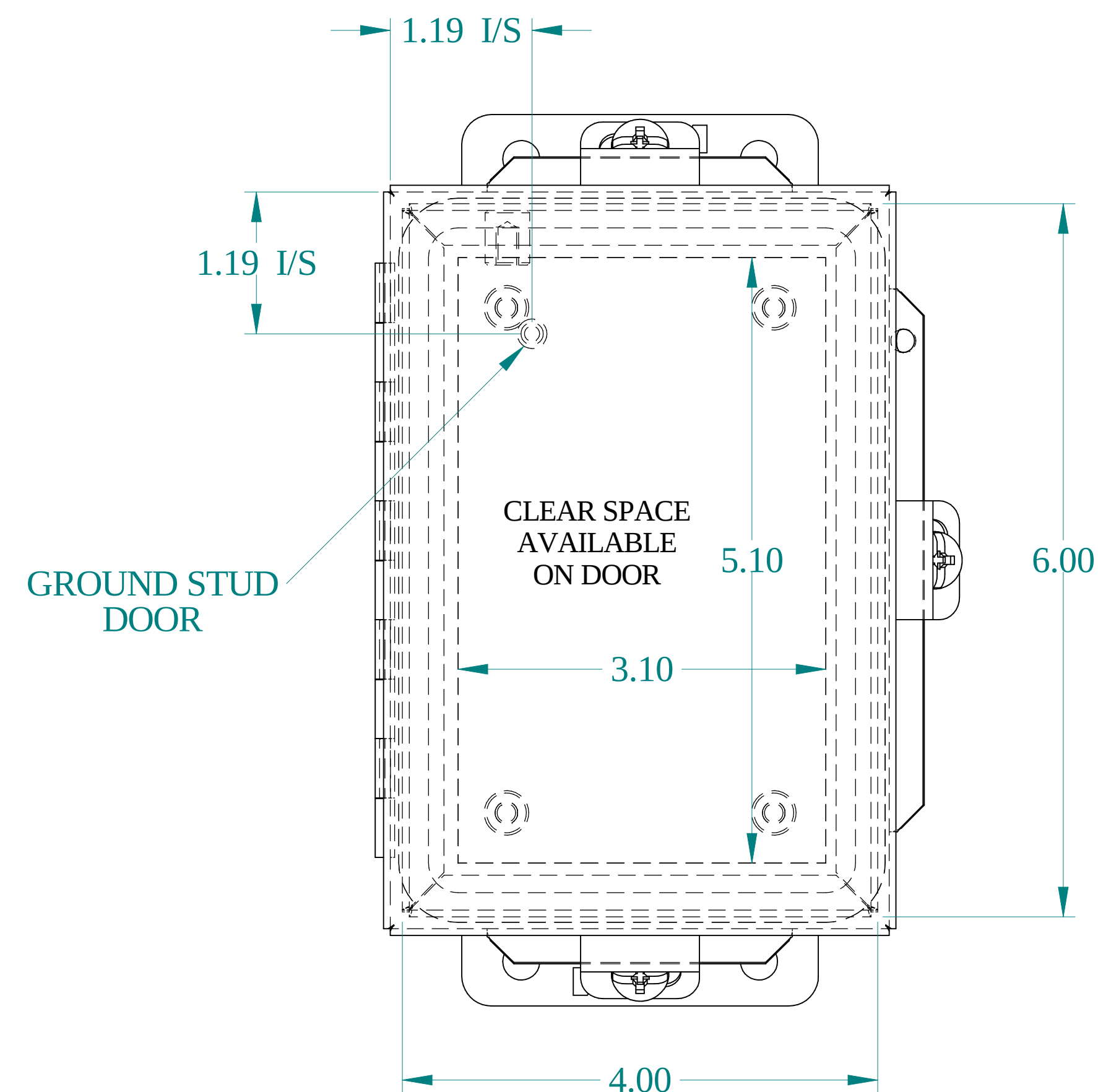
FRONT VIEW
