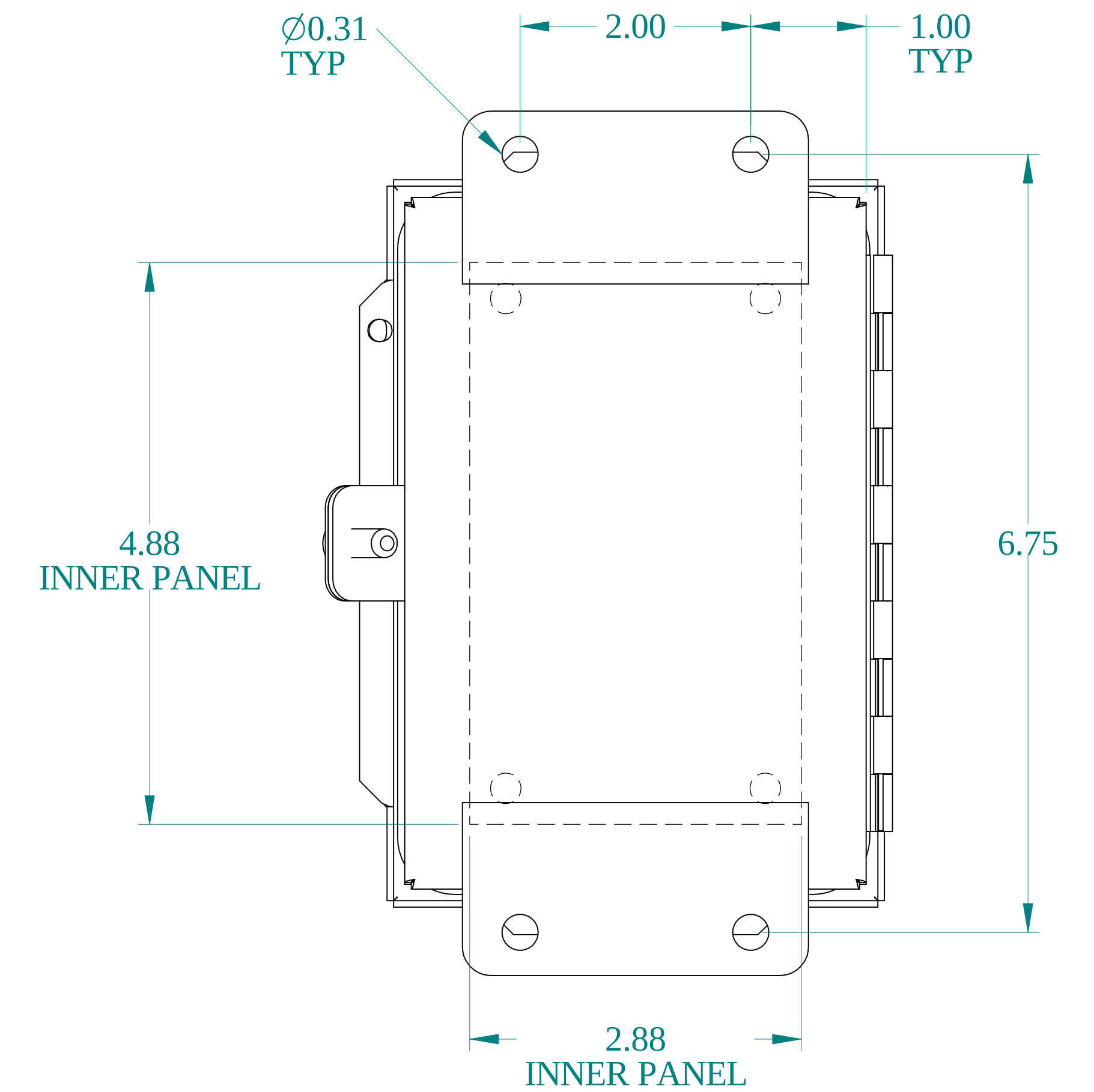
BACK VIEW
