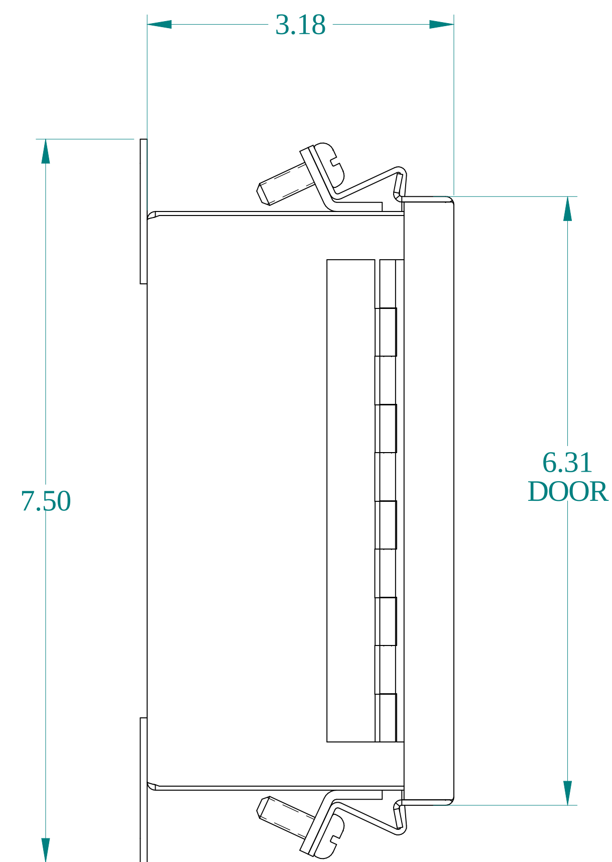
SIDE VIEW
