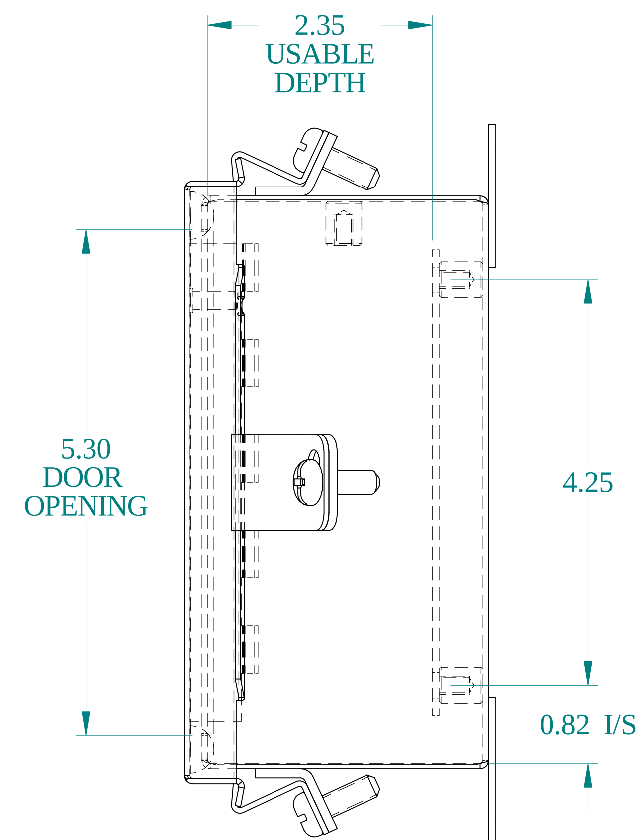
SIDE VIEW
