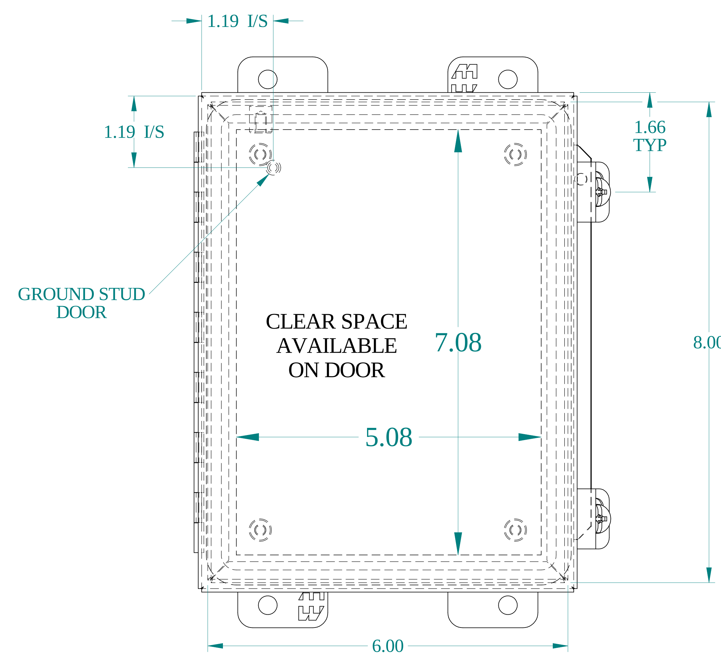
FRONT VIEW
