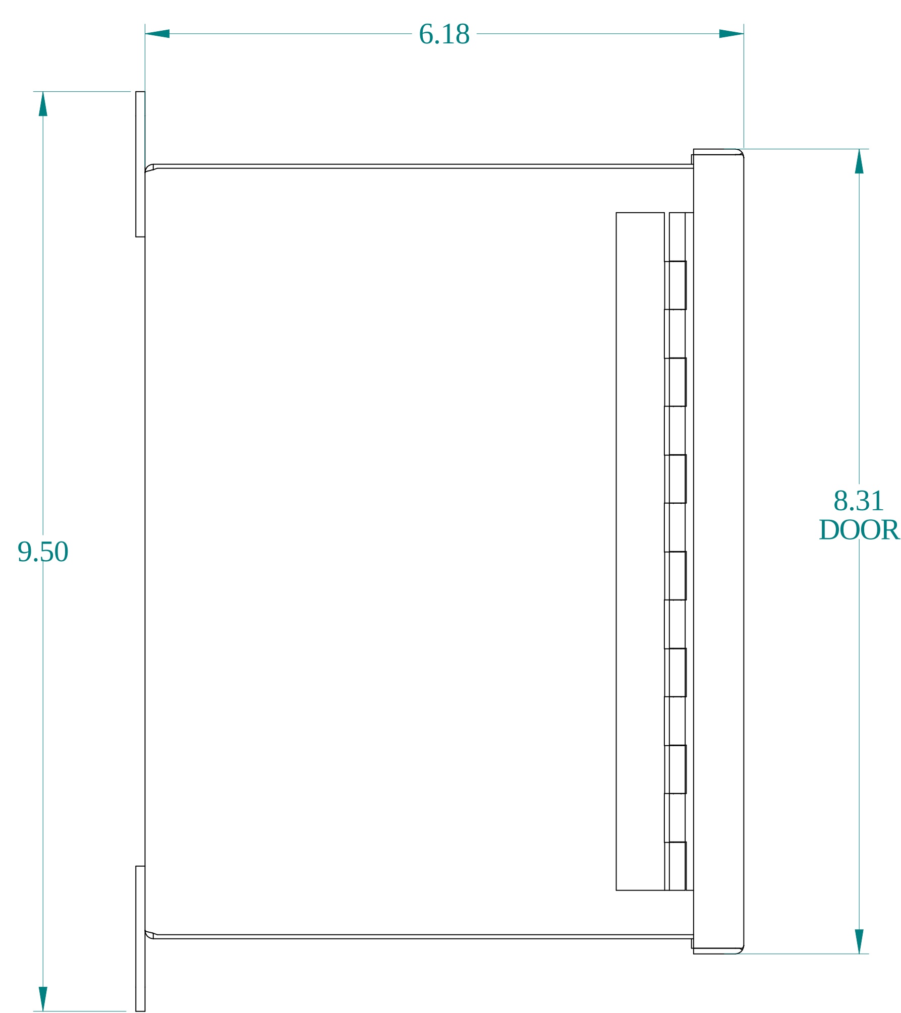
SIDE VIEW
