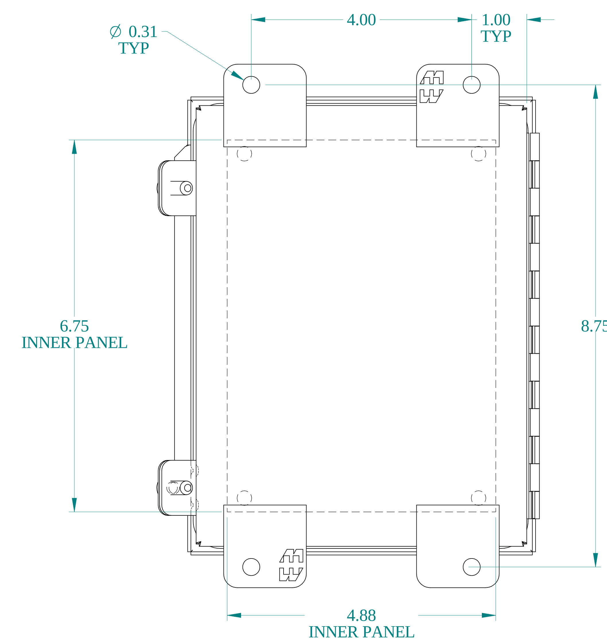
BACK VIEW
