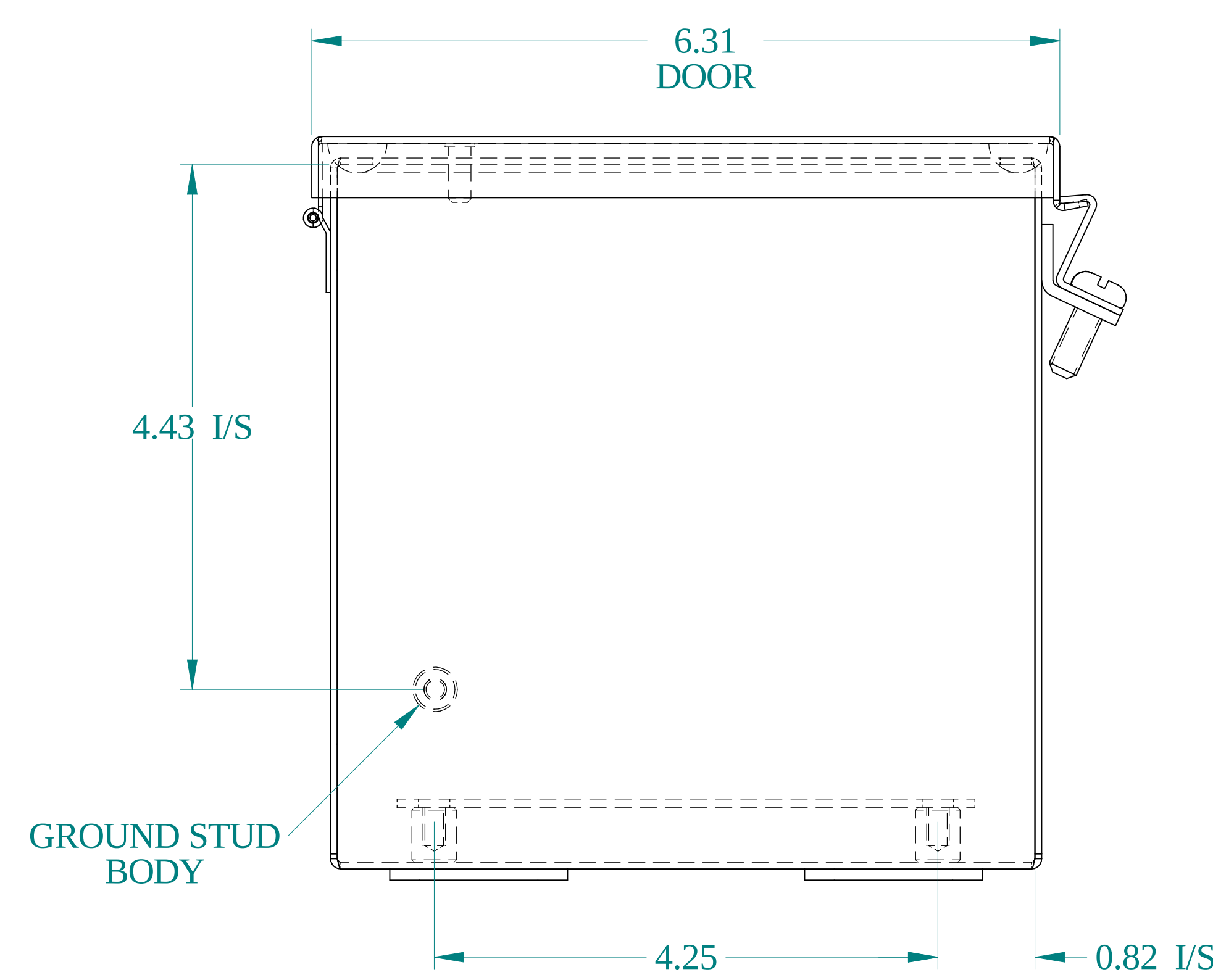
BOTTOM VIEW
