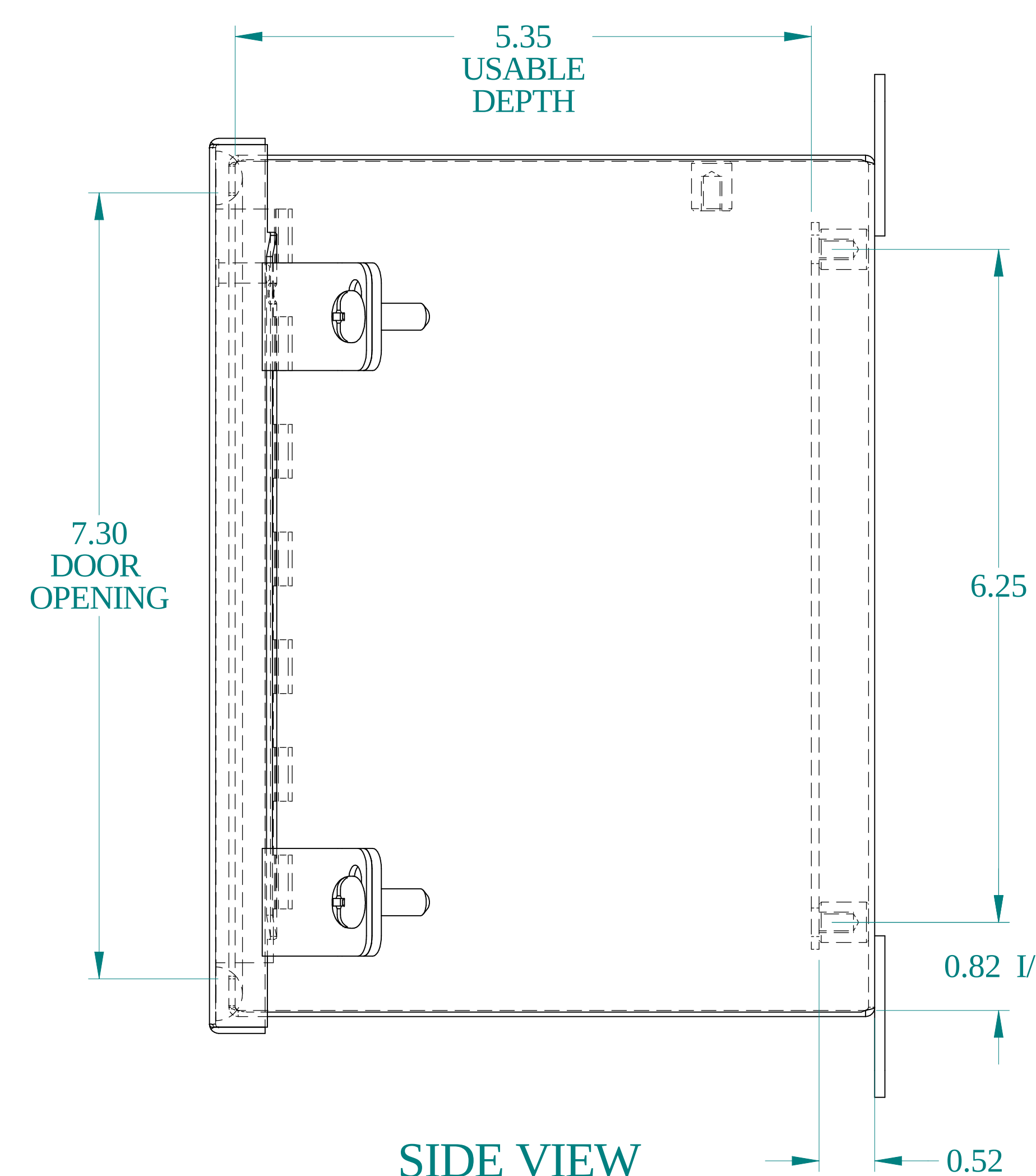
SIDE VIEW
