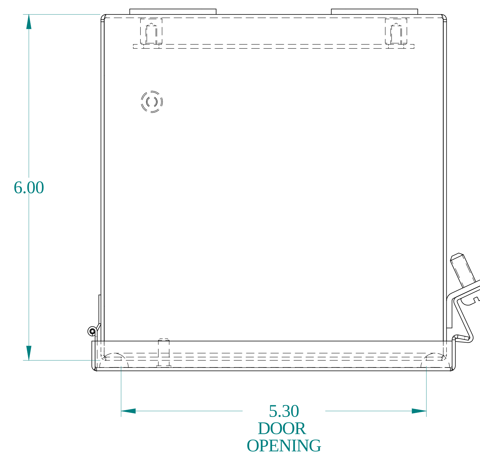
TOP VIEW
