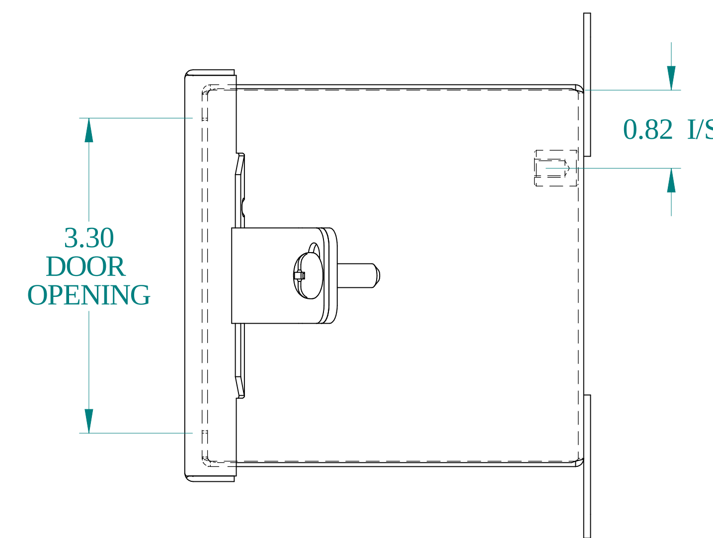
SIDE VIEW
