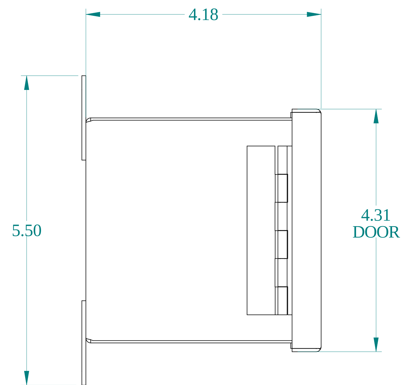
SIDE VIEW
