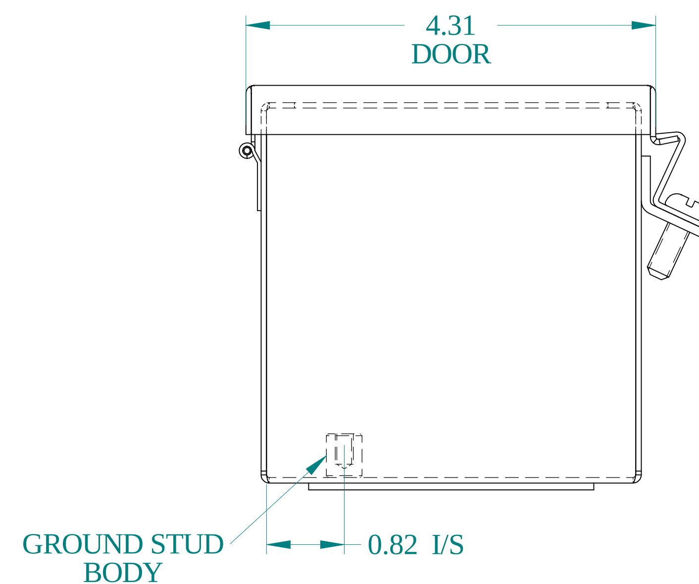
BOTTOM VIEW
