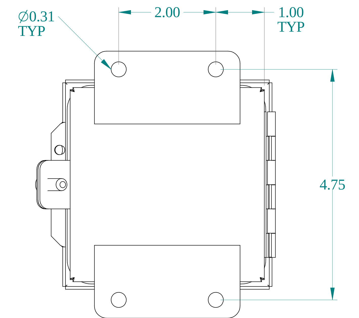
BACK VIEW
