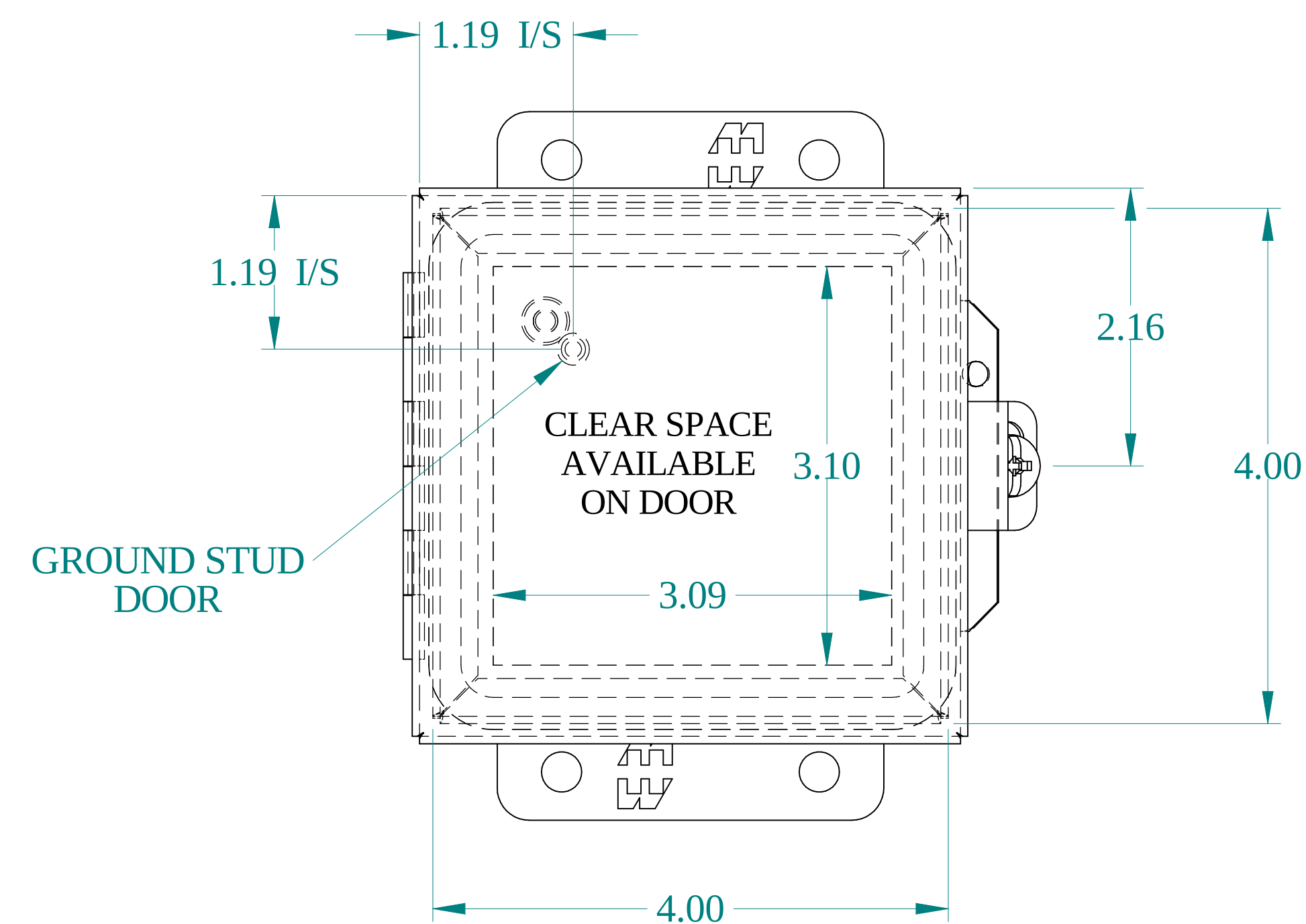
FRONT VIEW
