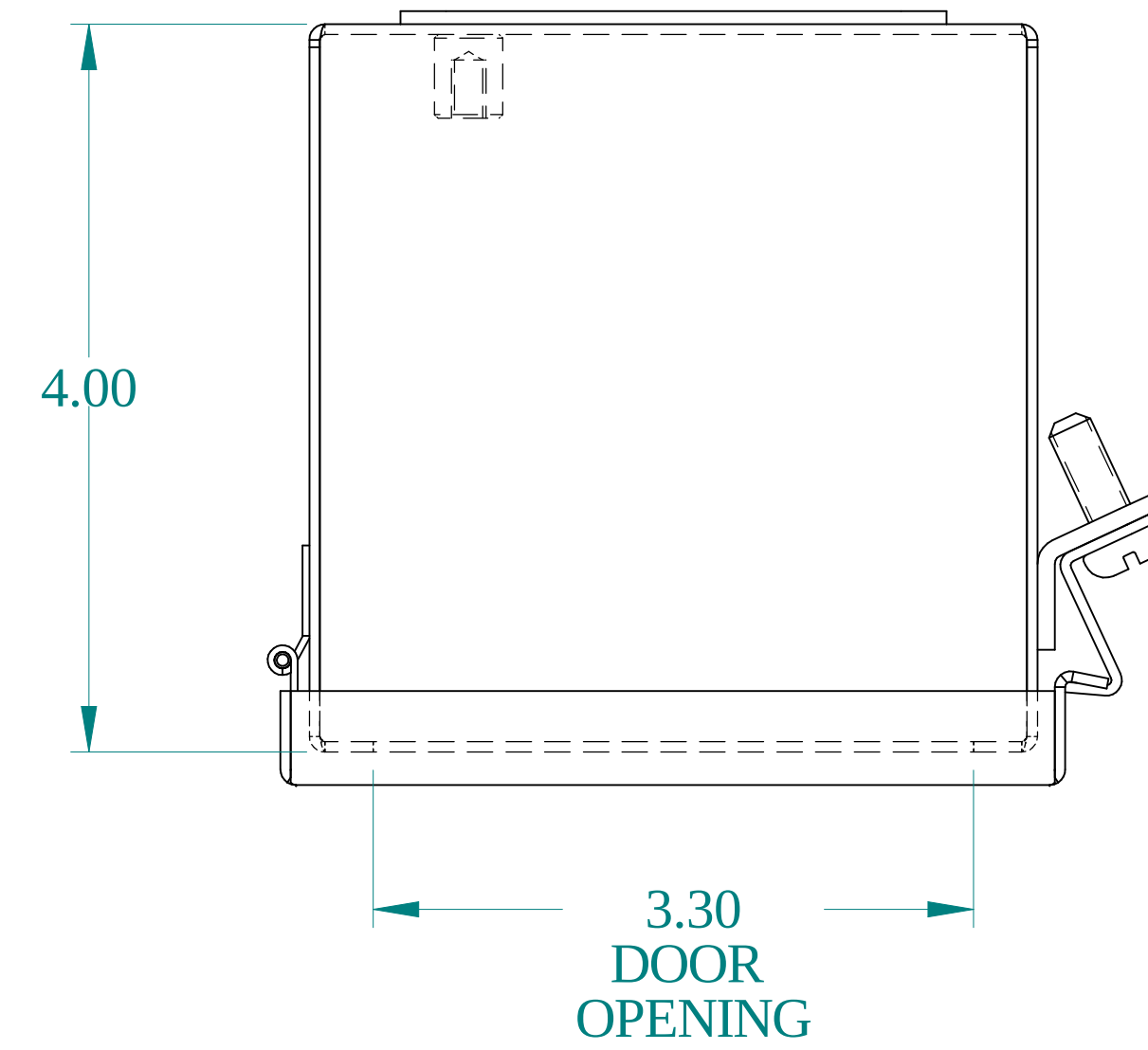
TOP VIEW
