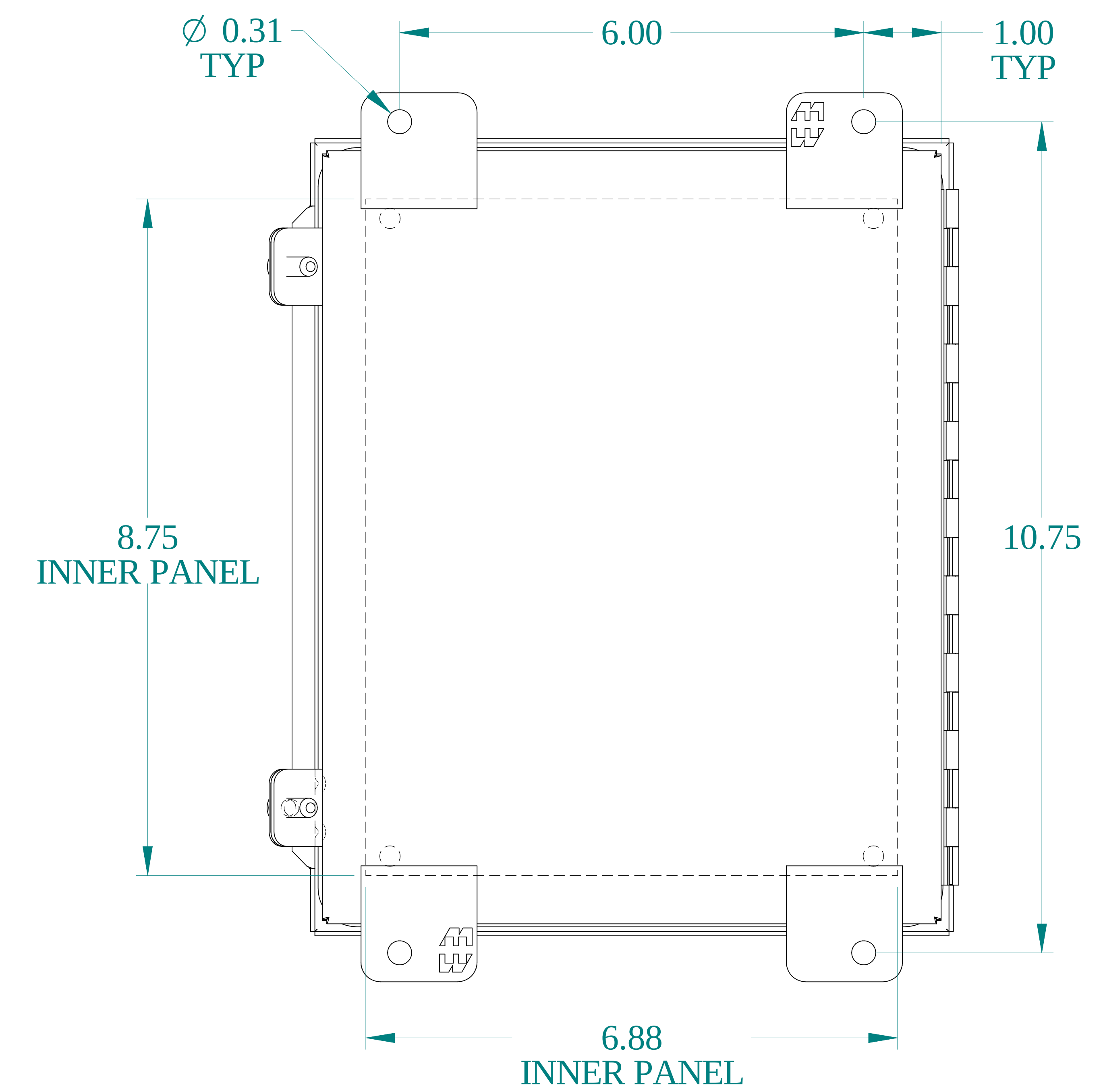
BACK VIEW
