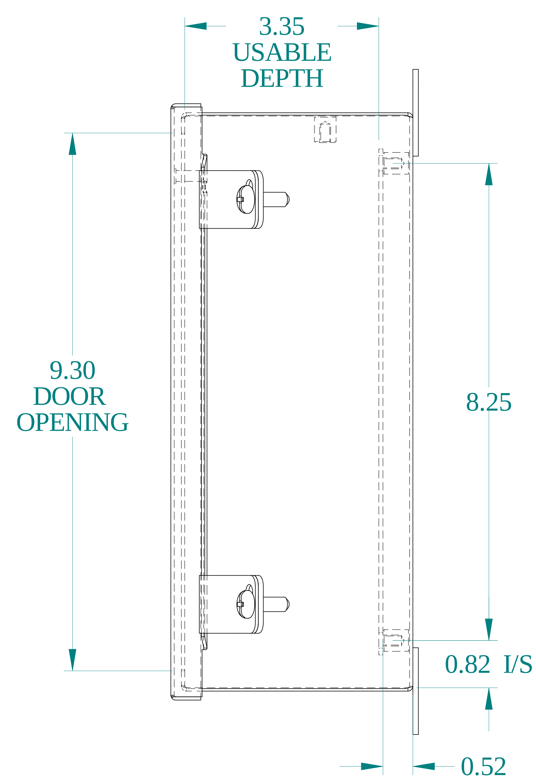
SIDE VIEW
