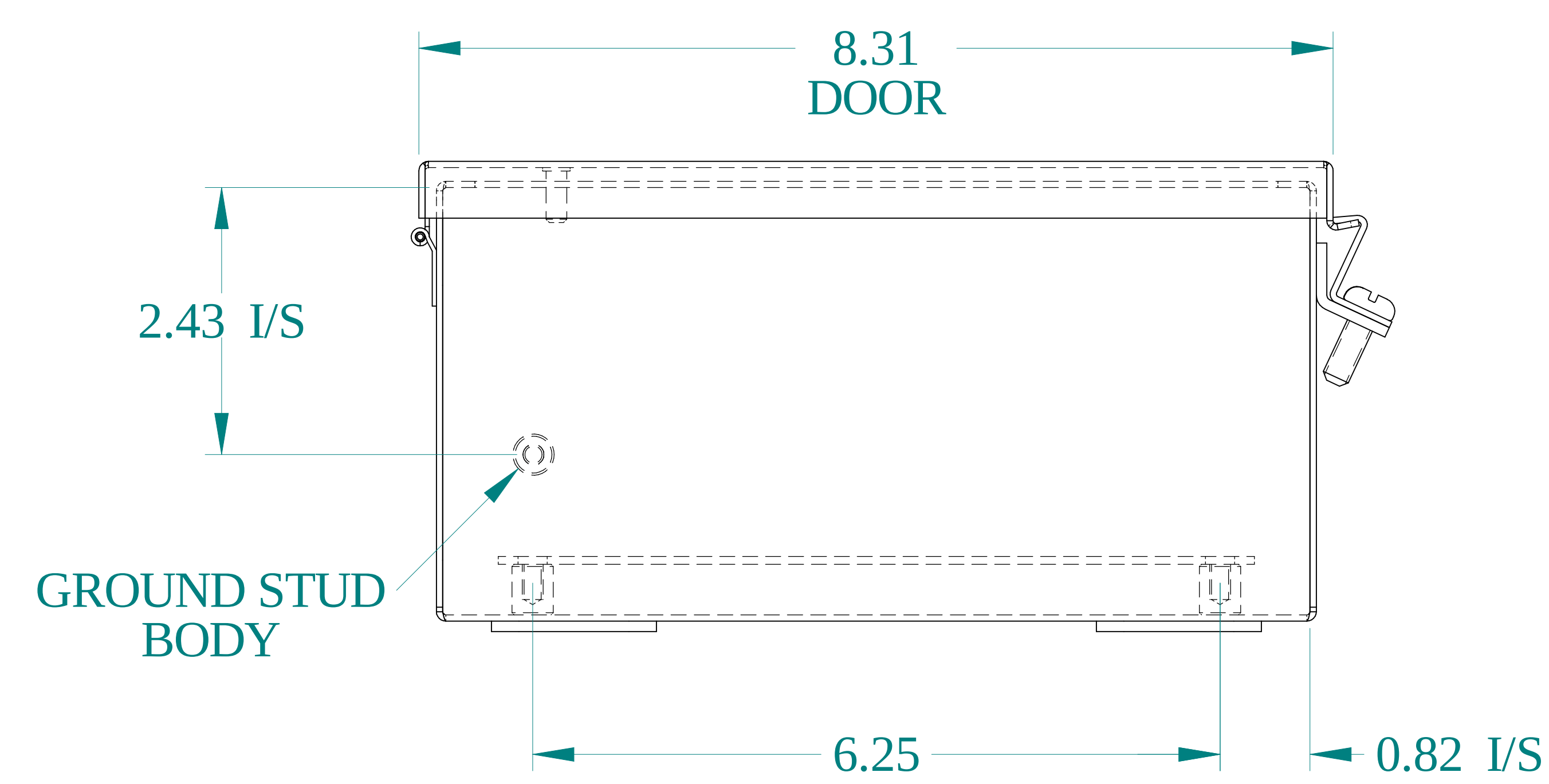
BOTTOM VIEW
