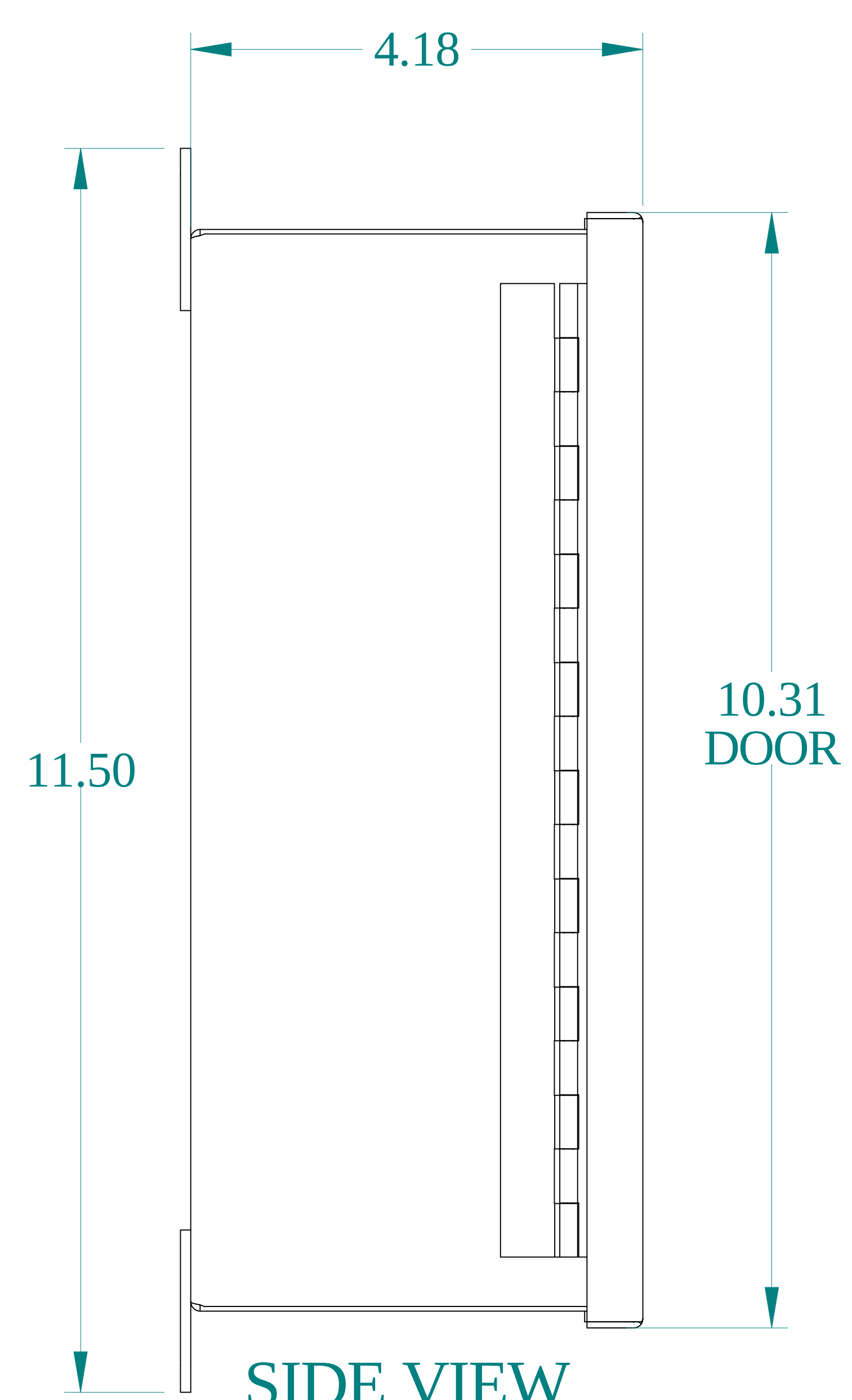
SIDE VIEW
