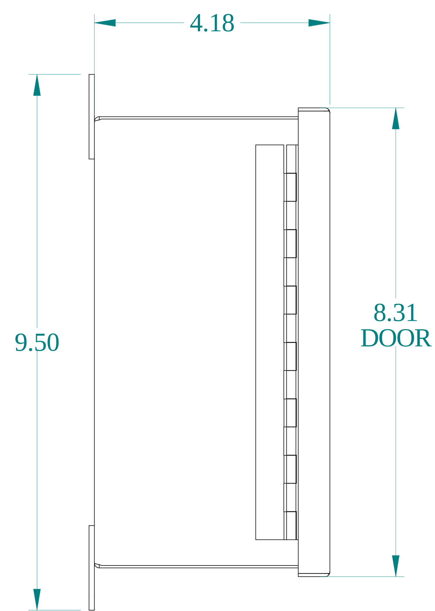
SIDE VIEW
