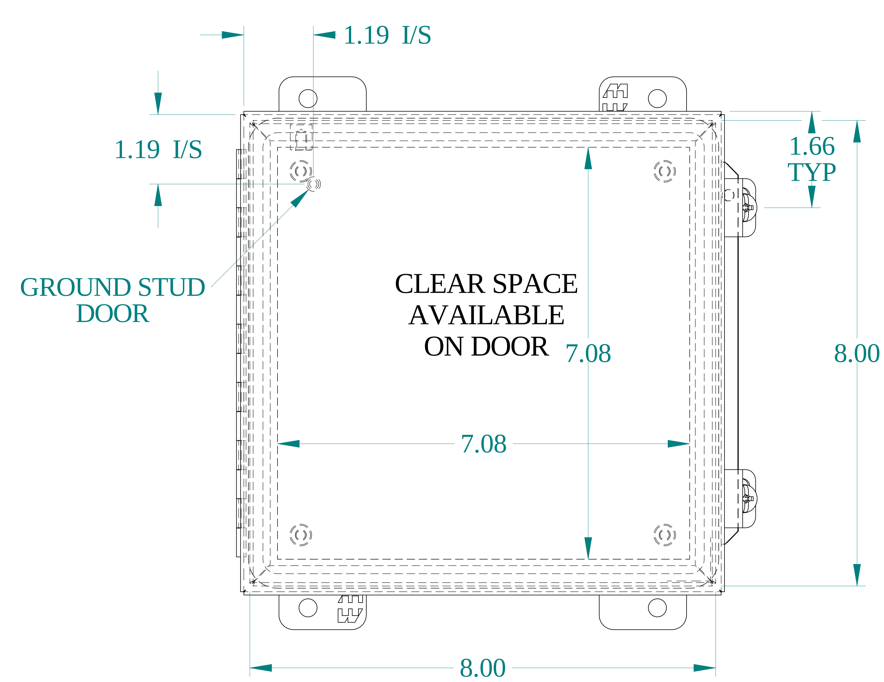
FRONT VIEW
