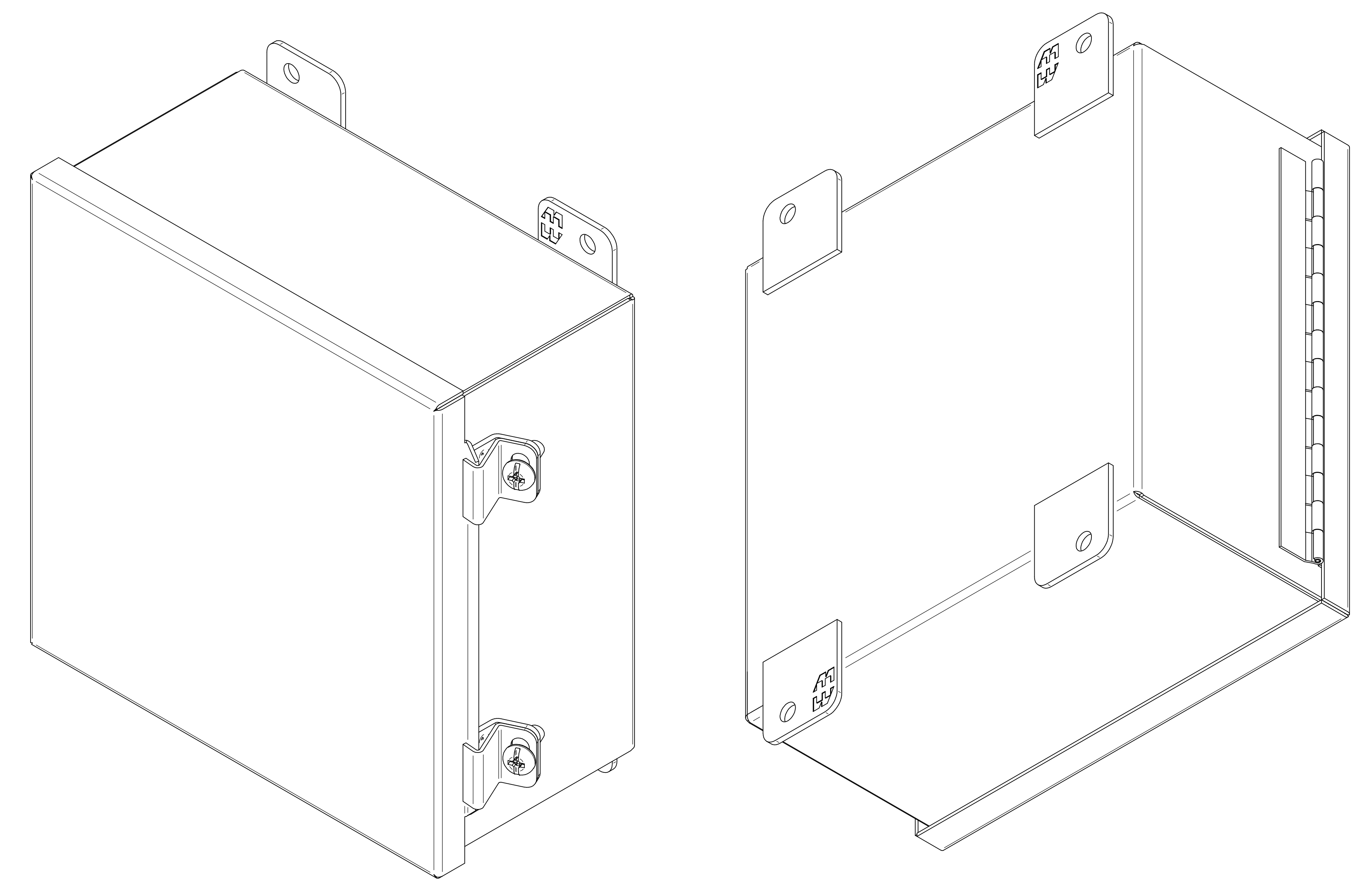
ISOMETRIC VIEWS
