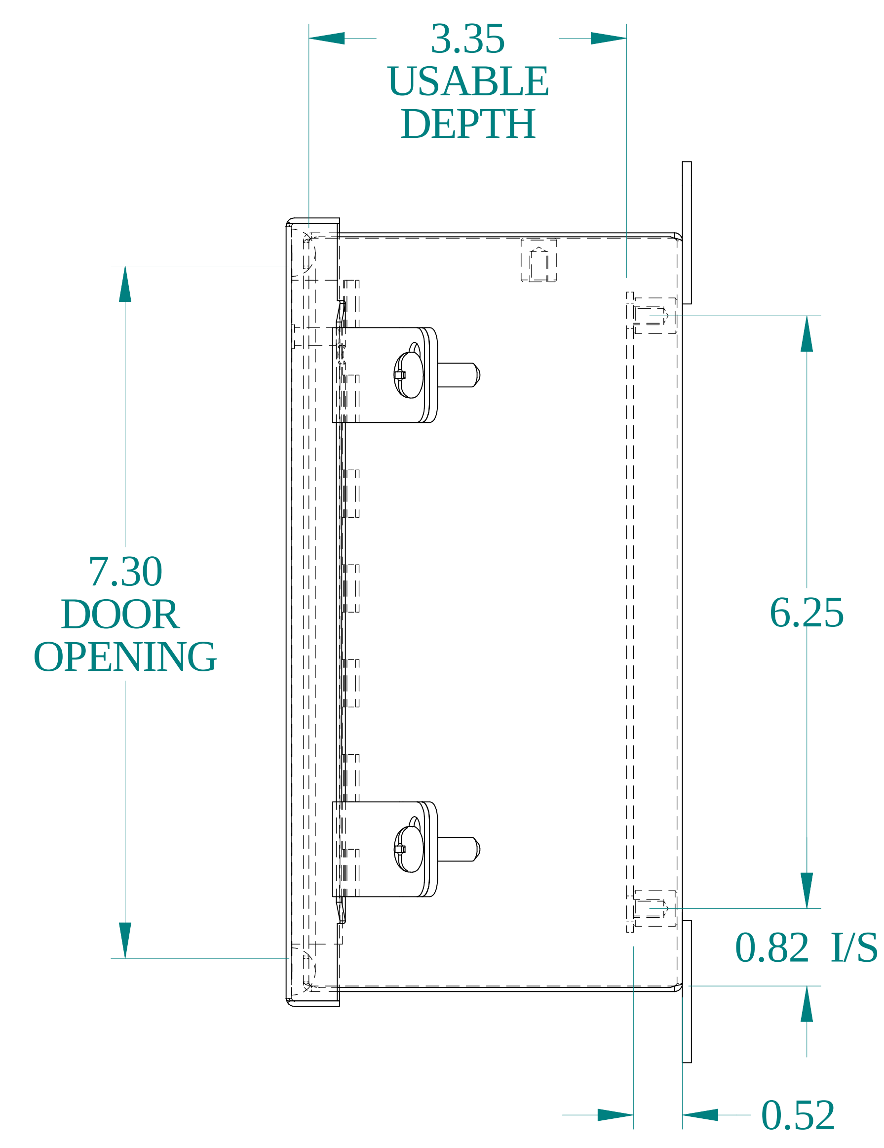
SIDE VIEW
