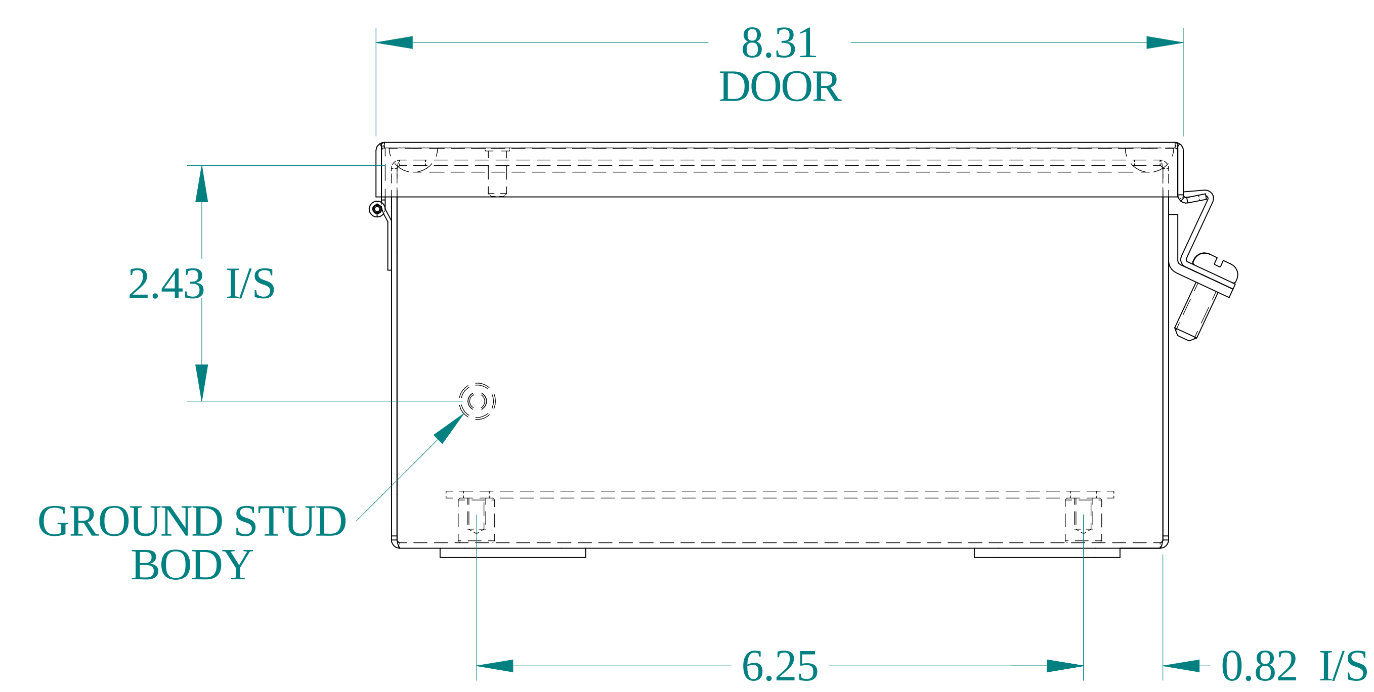
BOTTOM VIEW
