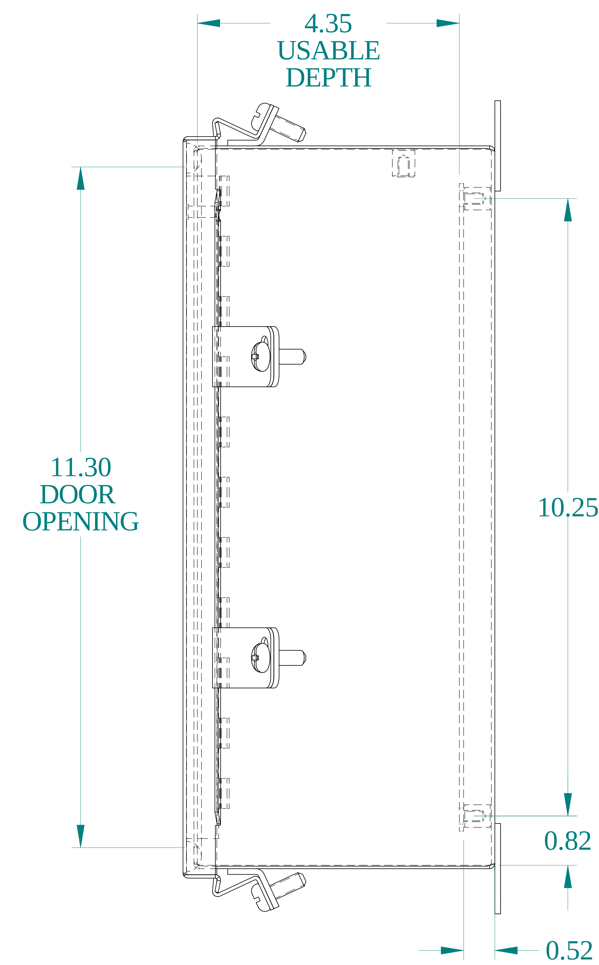
SIDE VIEW
