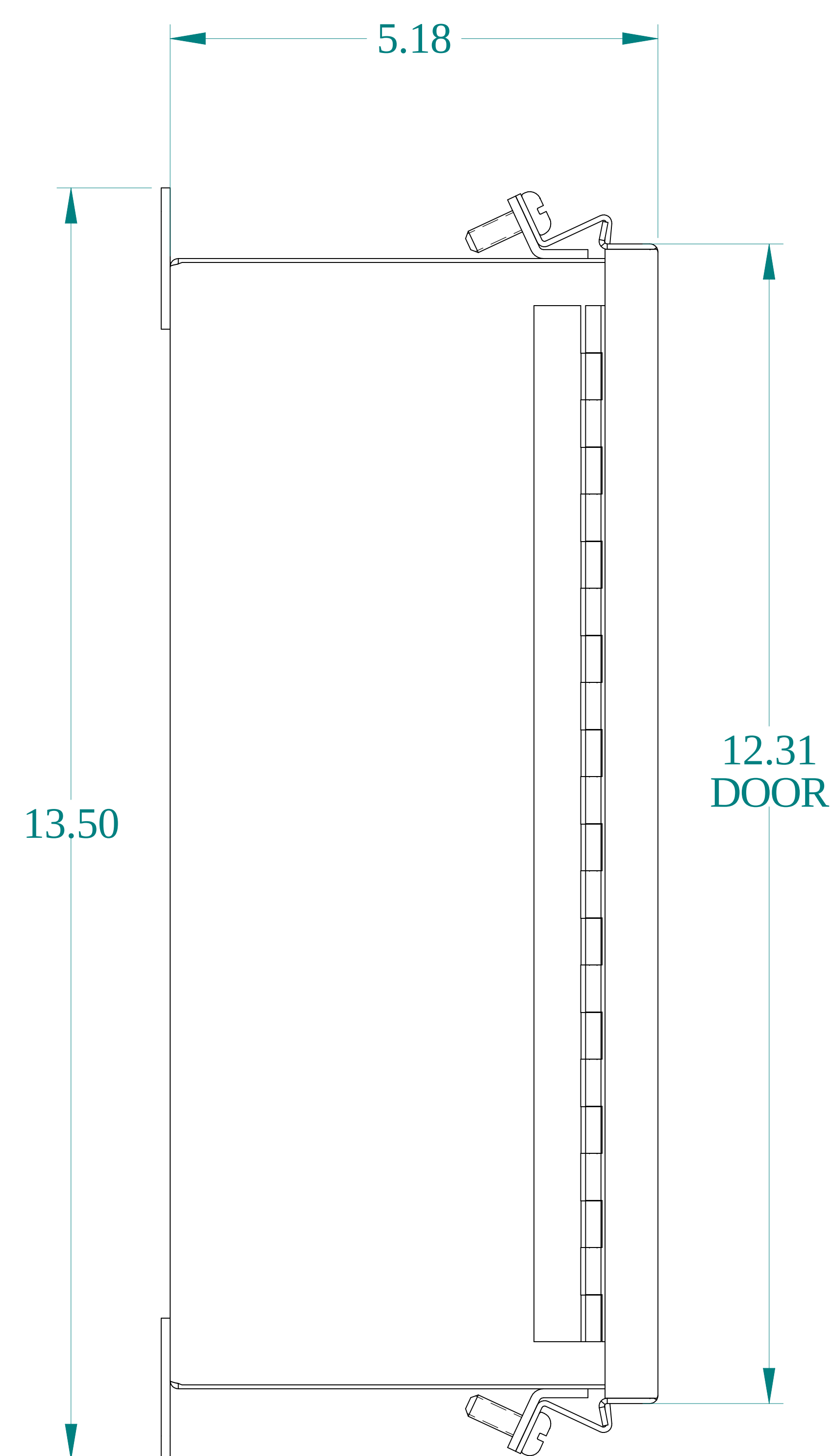
SIDE VIEW
