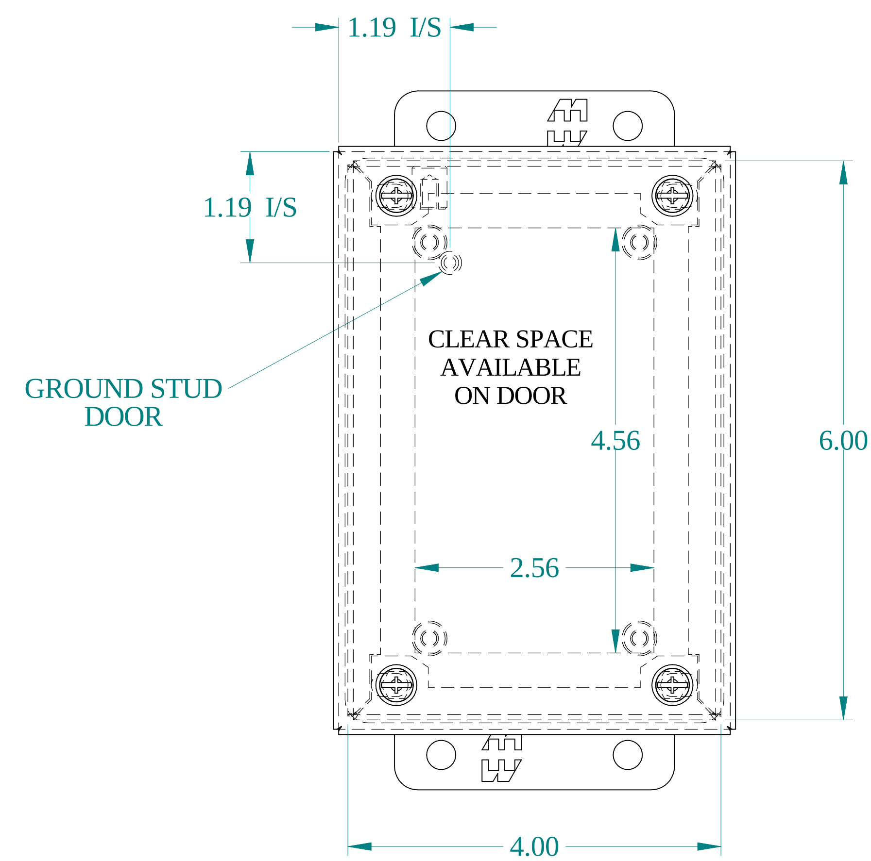
FRONT VIEW
