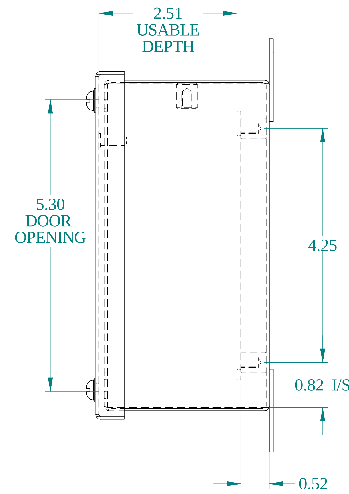
SIDE VIEW
