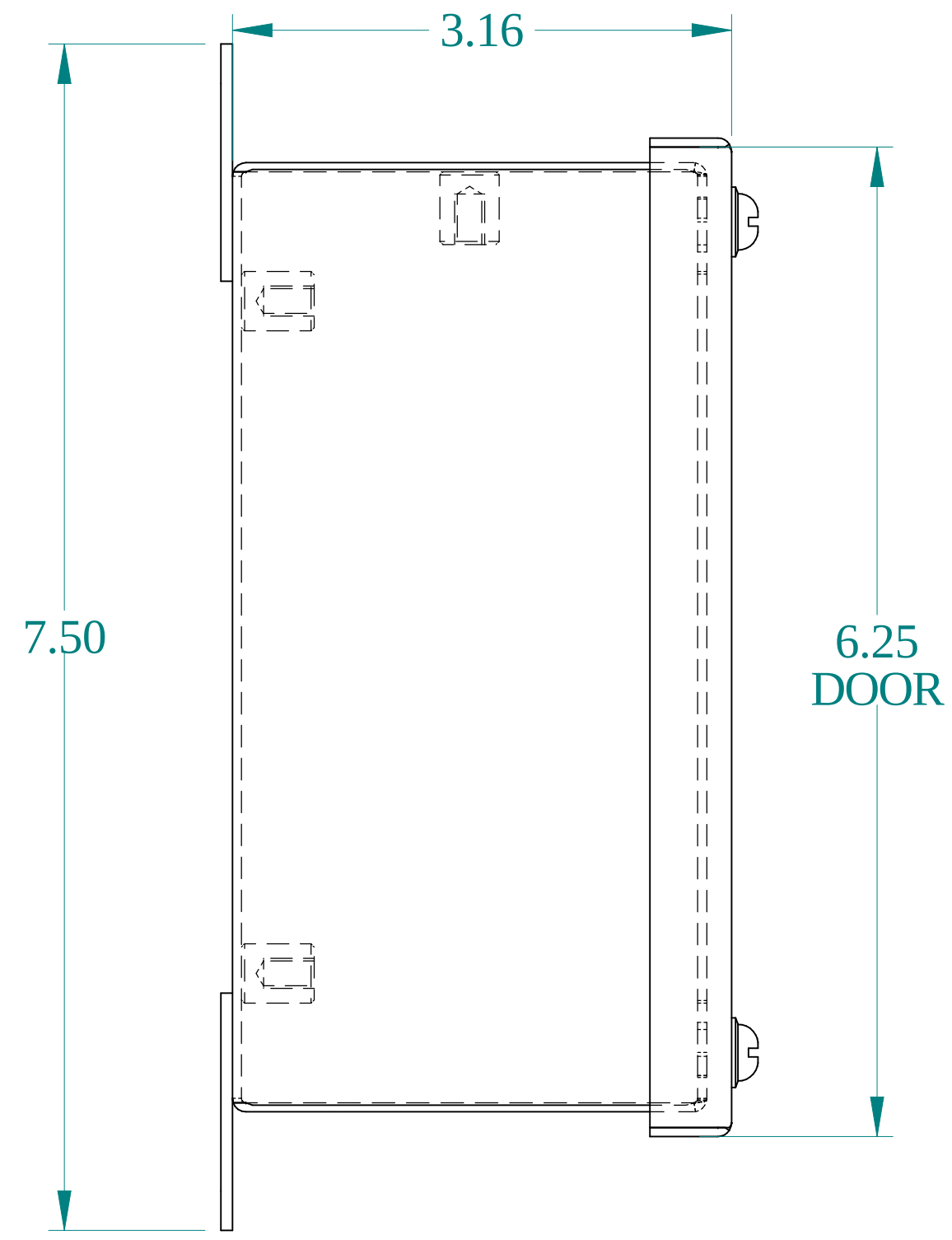
SIDE VIEW
