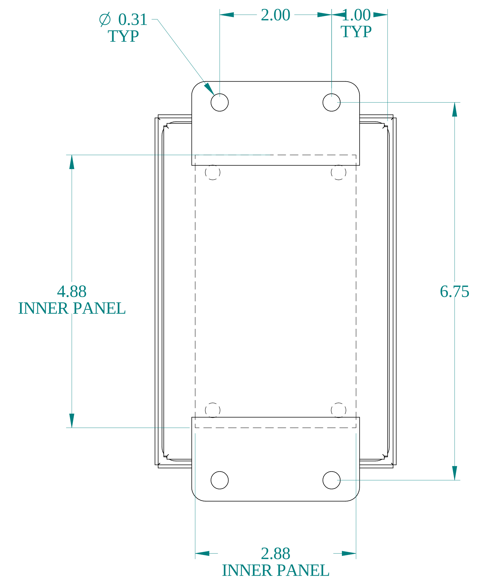
BACK VIEW
