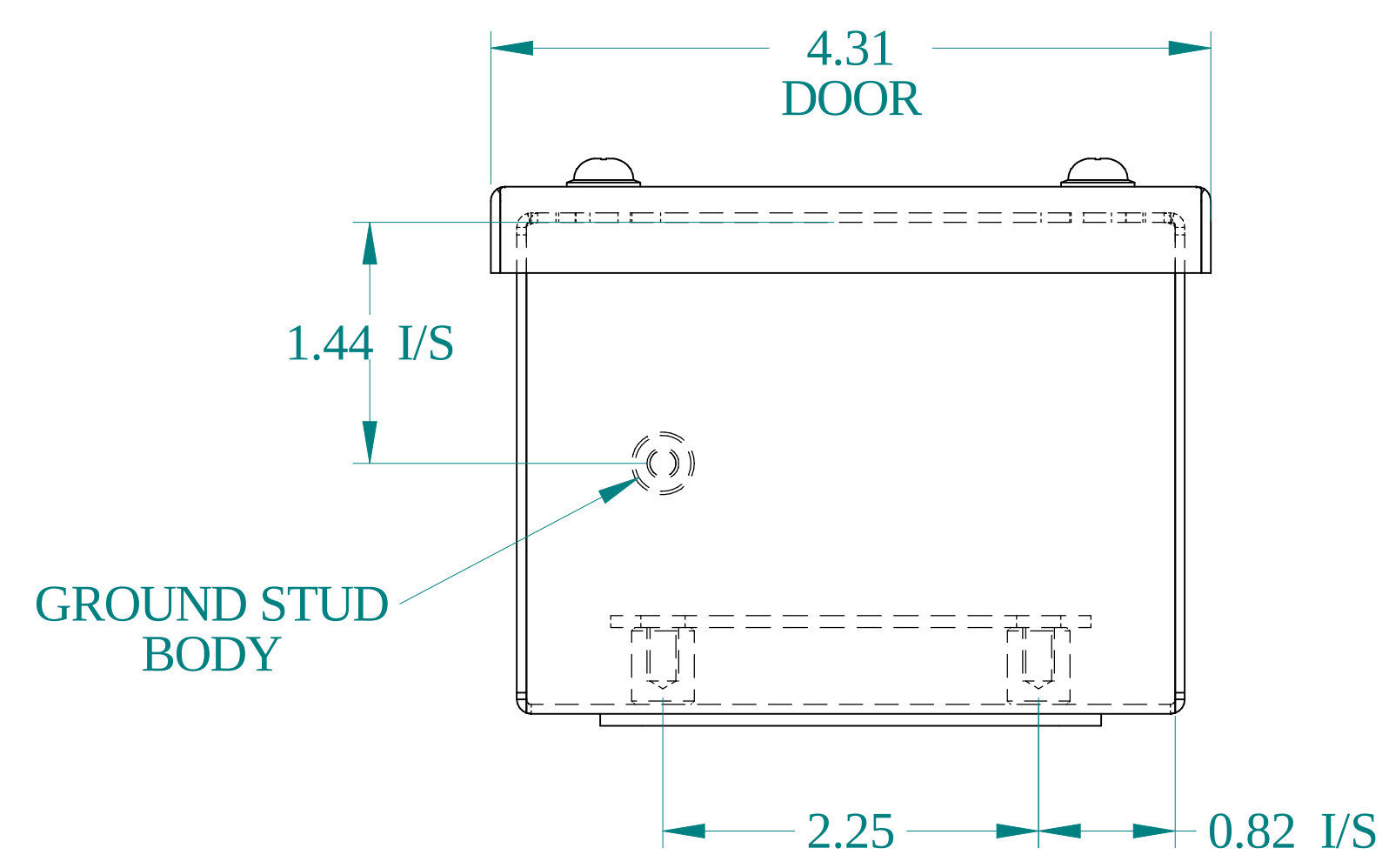
BOTTOM VIEW
