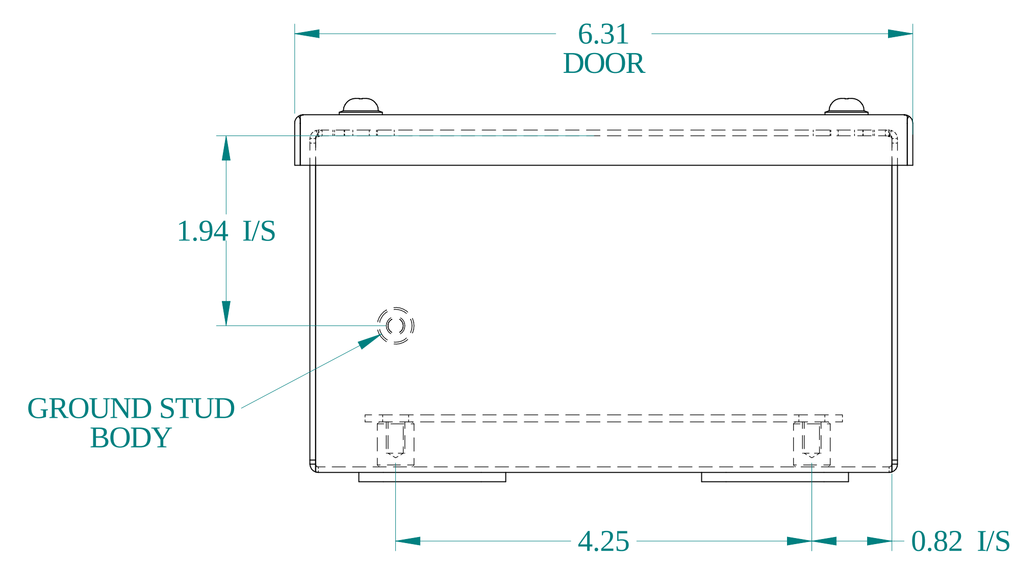
BOTTOM VIEW
