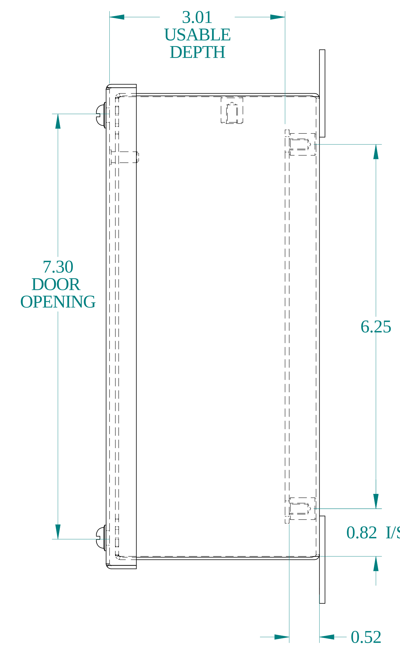
SIDE VIEW
