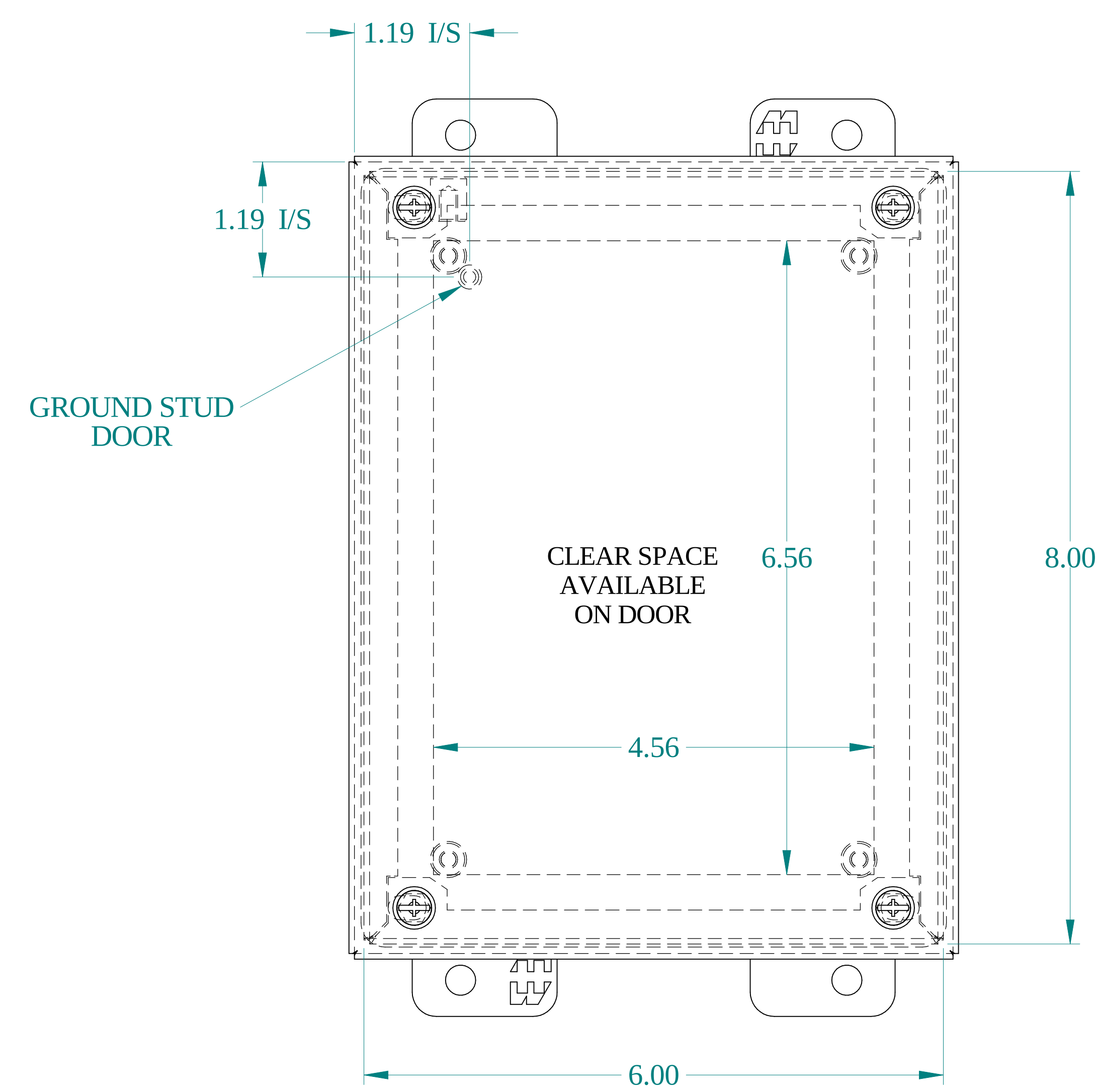
FRONT VIEW
