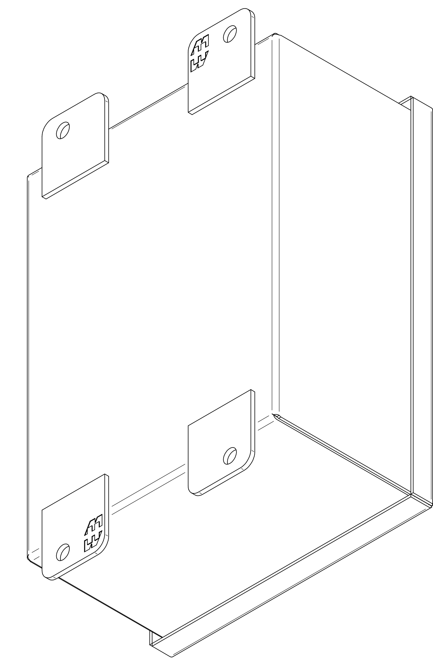
ISOMETRIC VIEWS
