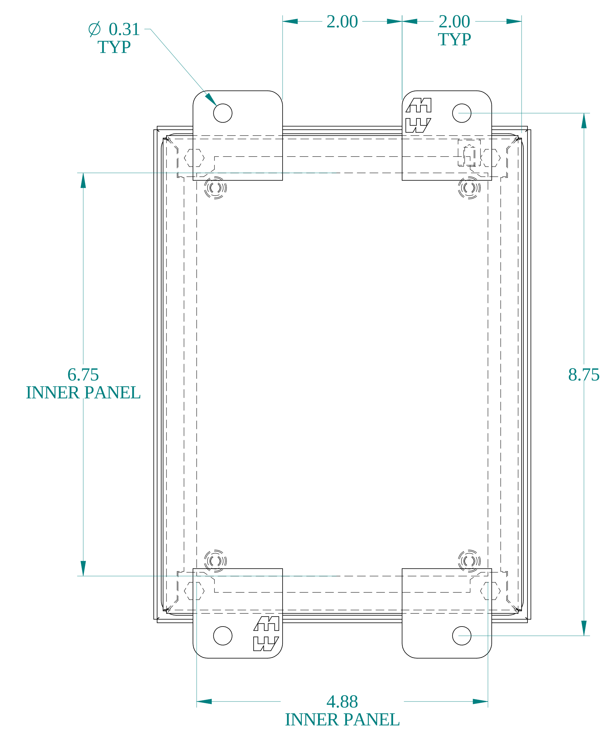
BACK VIEW
