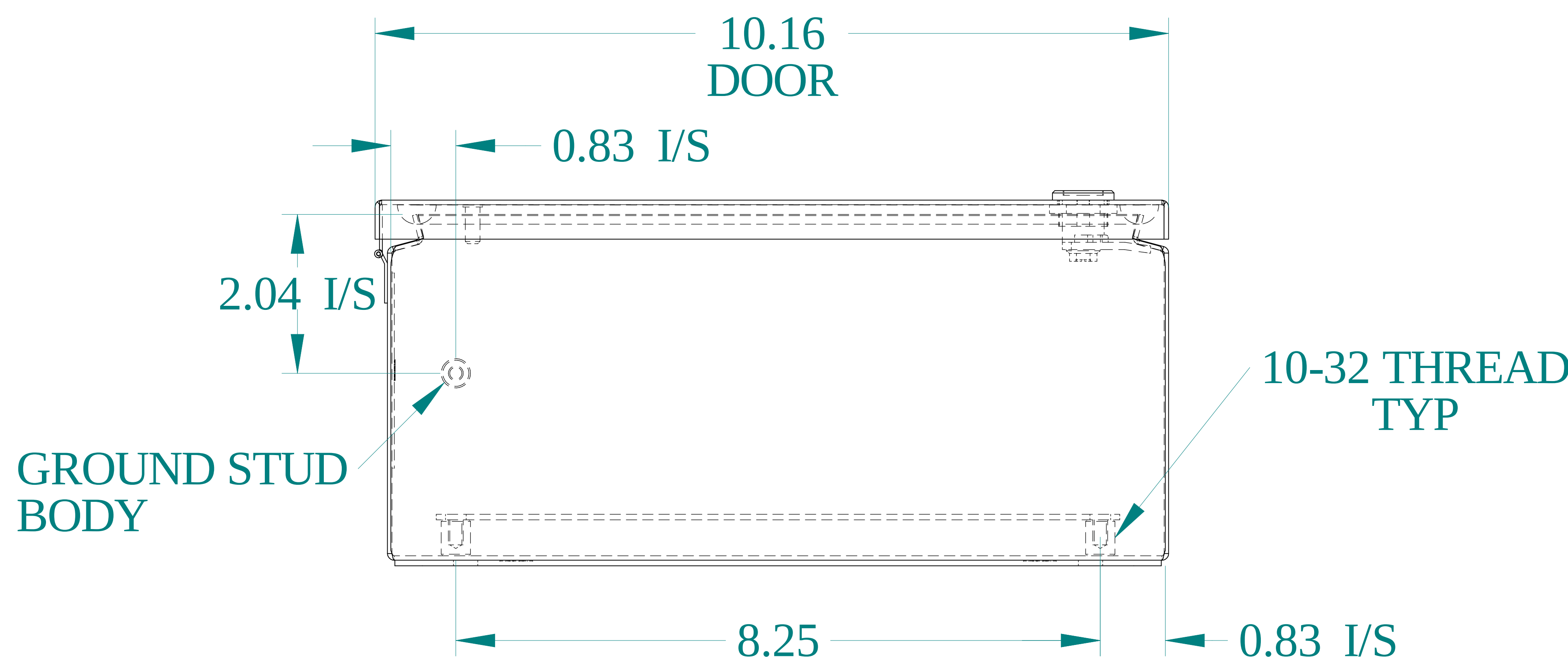
BOTTOM VIEW
