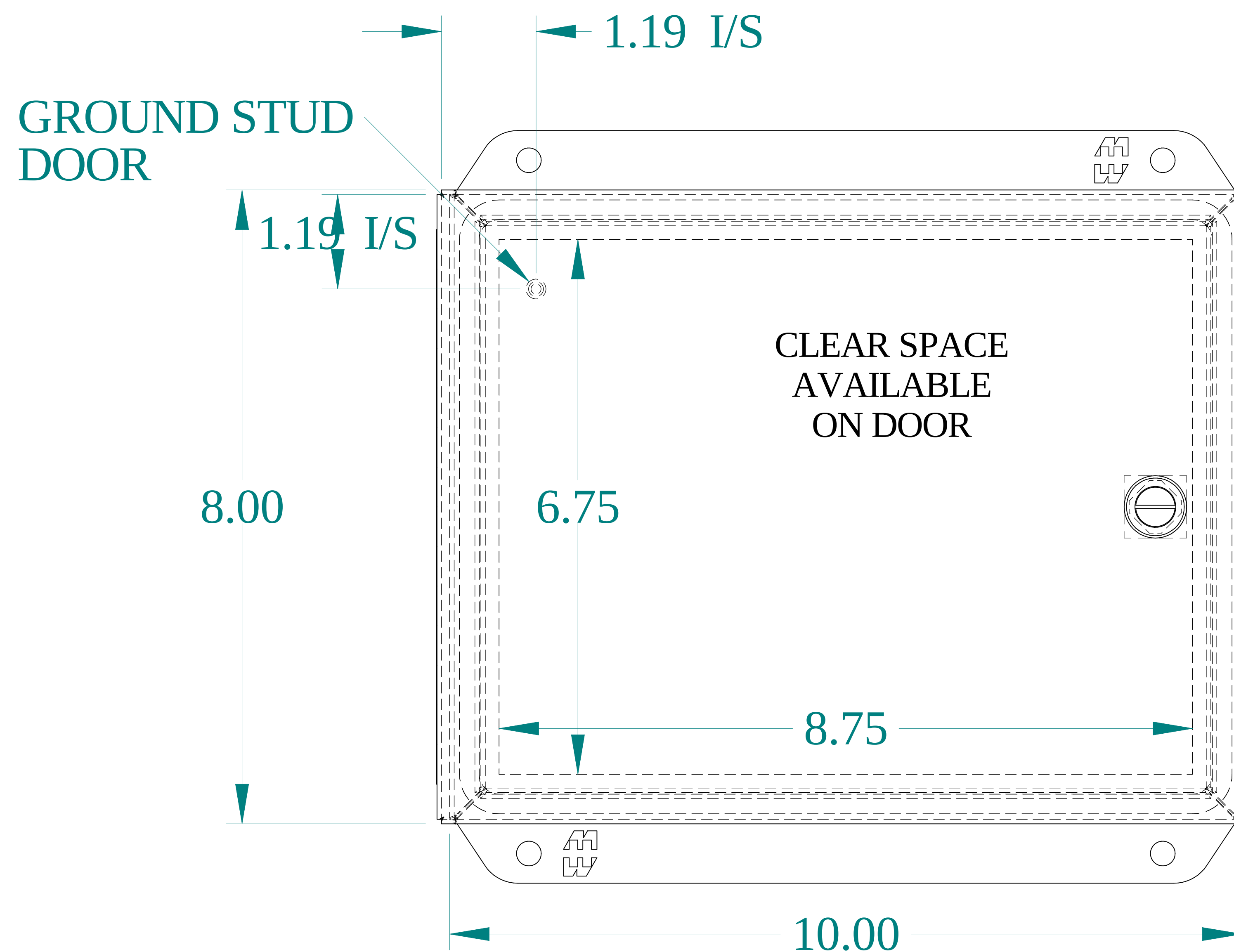
FRONT VIEW
