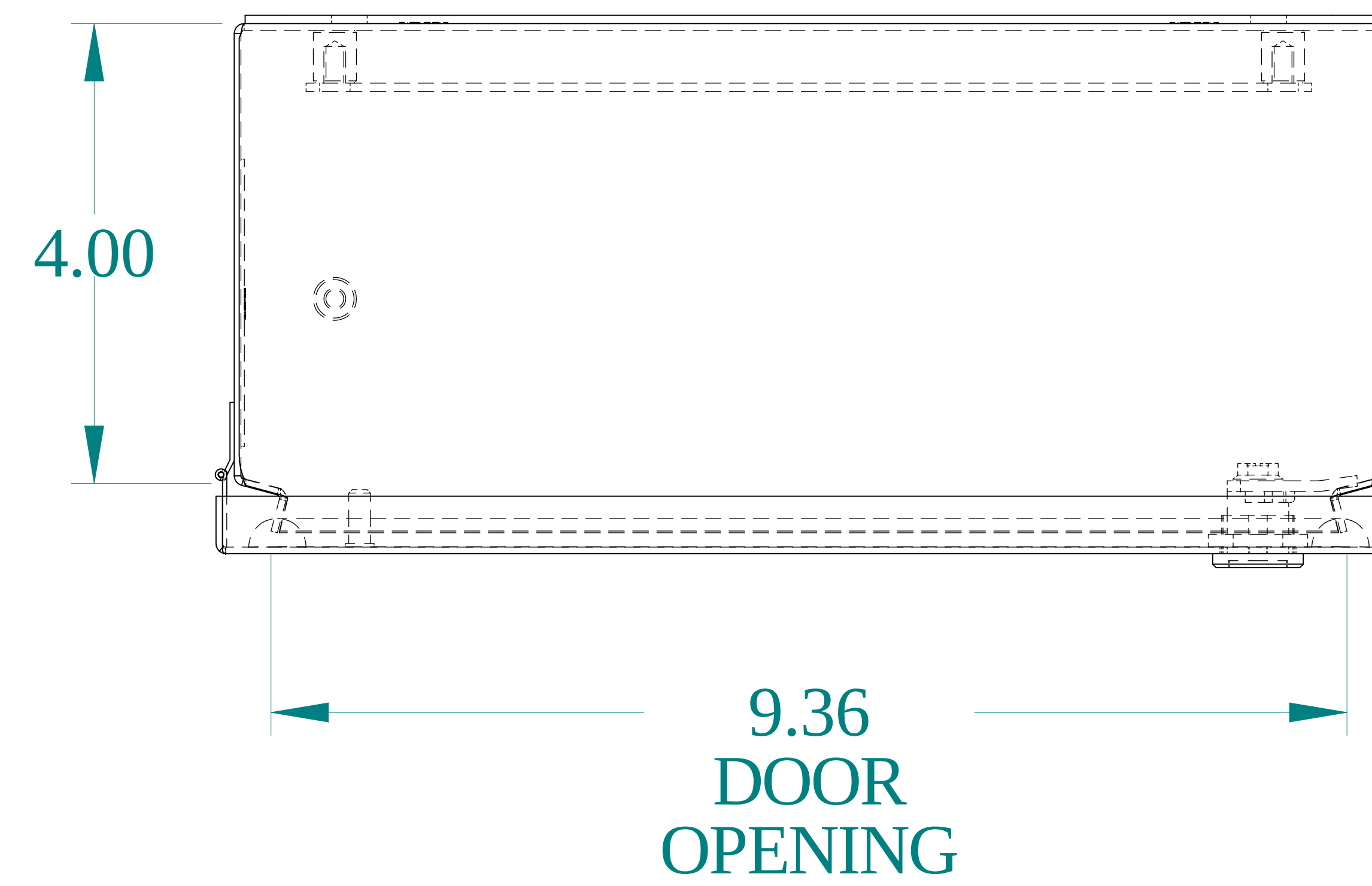
TOP VIEW
