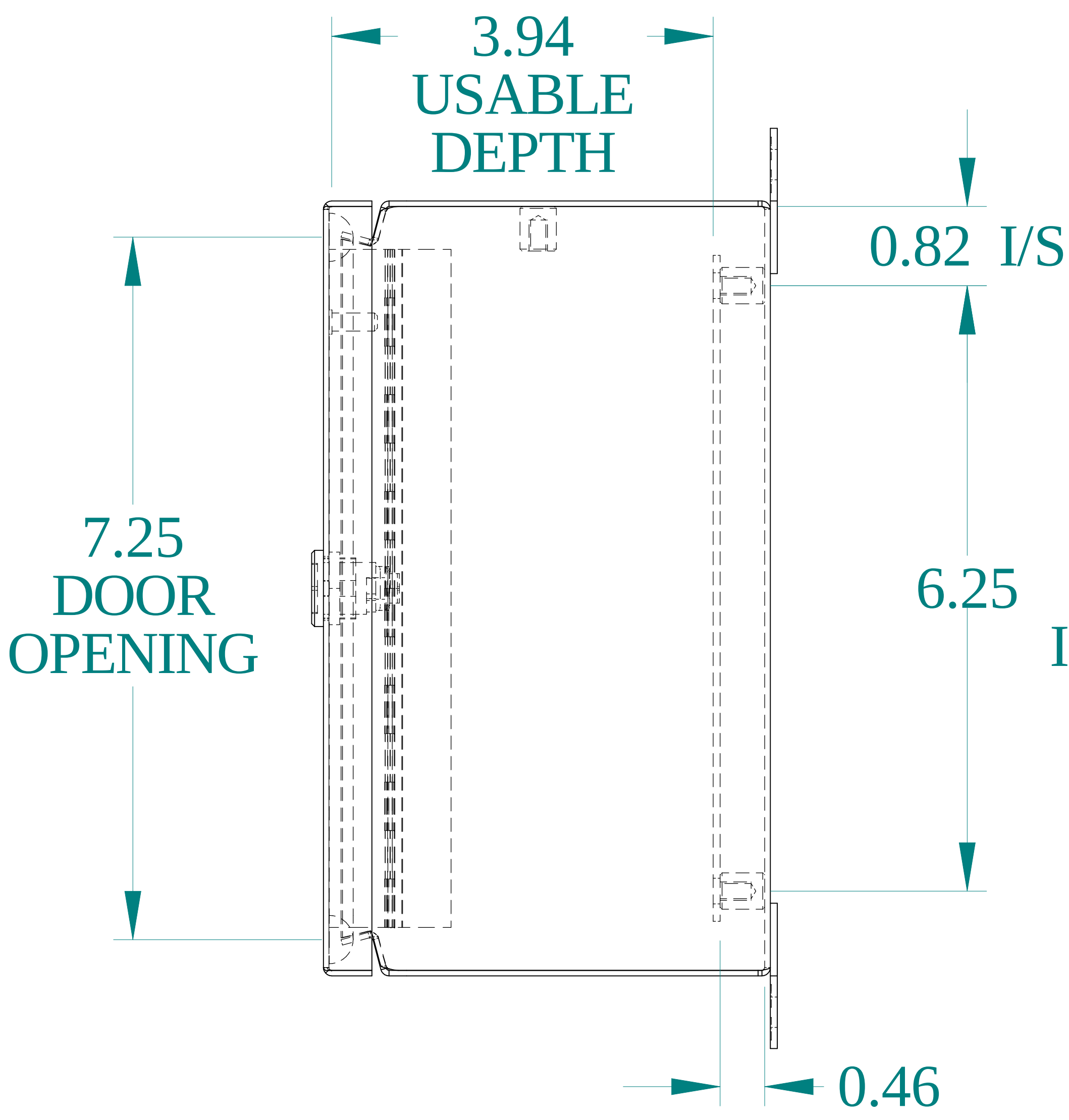
SIDE VIEW
