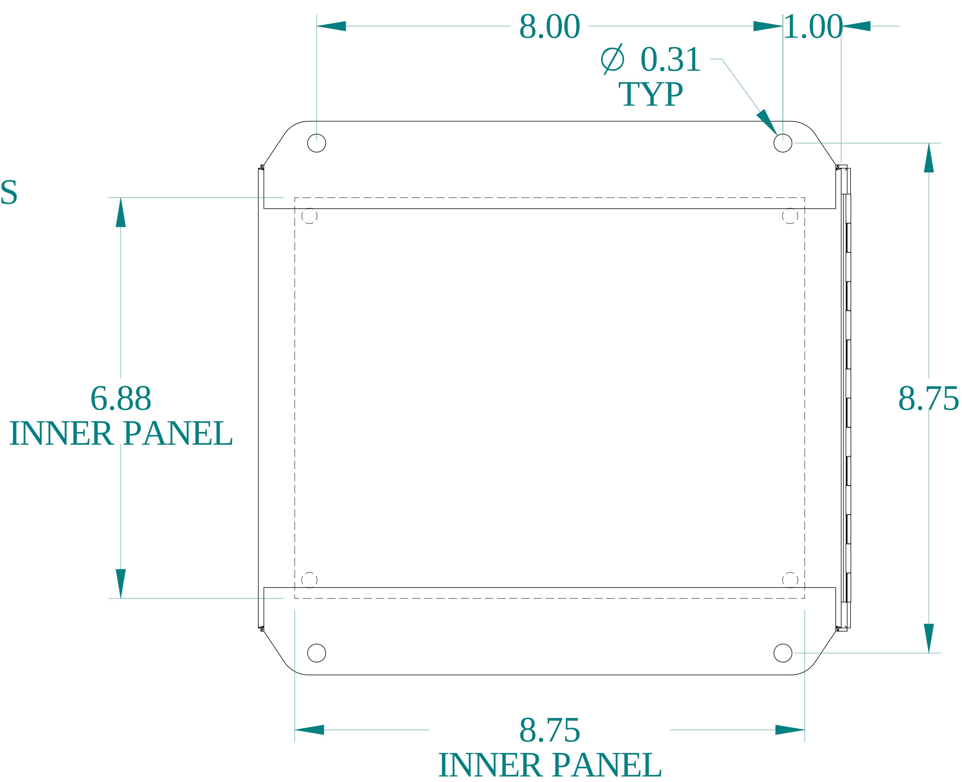
BACK VIEW
