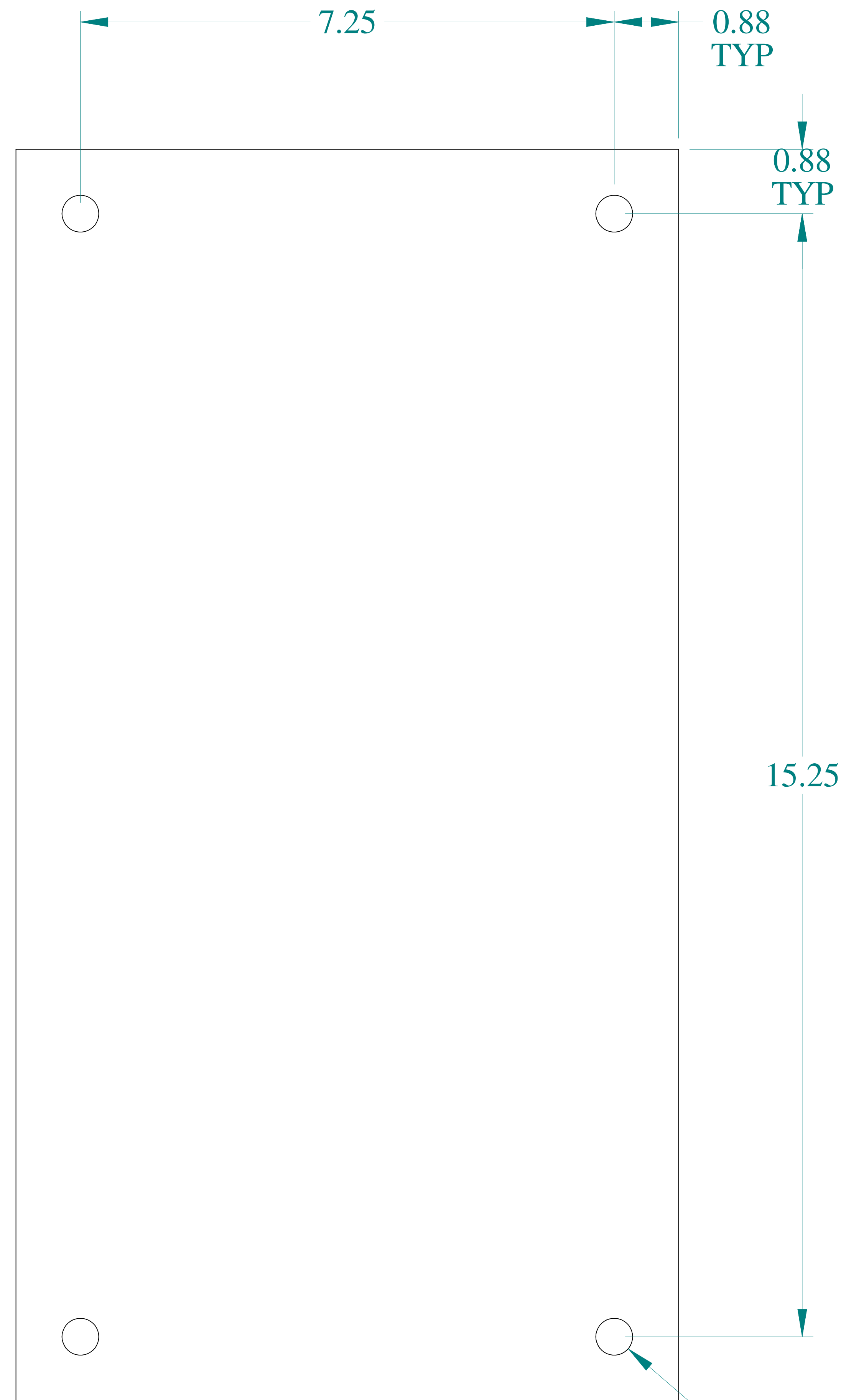
FRONT VIEW
